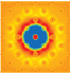
Contours of electron-density perturbation around a monovacancy in aluminum. The small red dots denote atoms around the vacancy. See article 205503.
