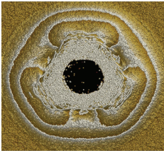
Atomistic simulation of the crater formed when a 315 000-atom gold particle hits a gold surface. The picture is of a horizontal slice 1 nm below the surface. See article 027601.
