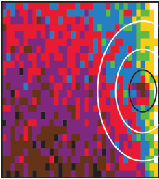
Events produced from the B^+ \rightarrow \bar{D}^0 D^0 K^+ decay binned by quantities constructed from the energy (vertical) and momentum (horizontal) of the decay products. The darker boxes within the black ellipse signal a new D_{sj} meson. See article 092001.
