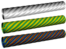
A twisted 35-walled carbon nanotube (top), its Gaussian curvature map (middle), and energy density map (bottom). See article 085503.
