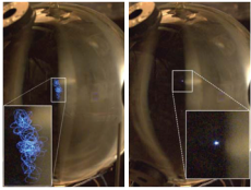
Photograph of single bubble sonoluminescence in a spherical resonator. A bubble driven acoustically at the second spherical mode of the resonator moves in orbits (left). Addition of a high harmonic results in a bright, stationary bubble (right). See article 074302.
