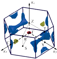
Fermi surface of solid metallic hydrogen at 414 GPa. The ab initio study predicts multiband superconductivity near room temperature. See article 257001.
