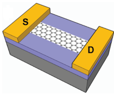
Schematic of graphene nanoribbon field-effect transistors with palladium contacts (S,D) on a 10 nm thick silicon dioxide surface (purple). The devices are found to be semiconducting at room temperature. See article 206803.
