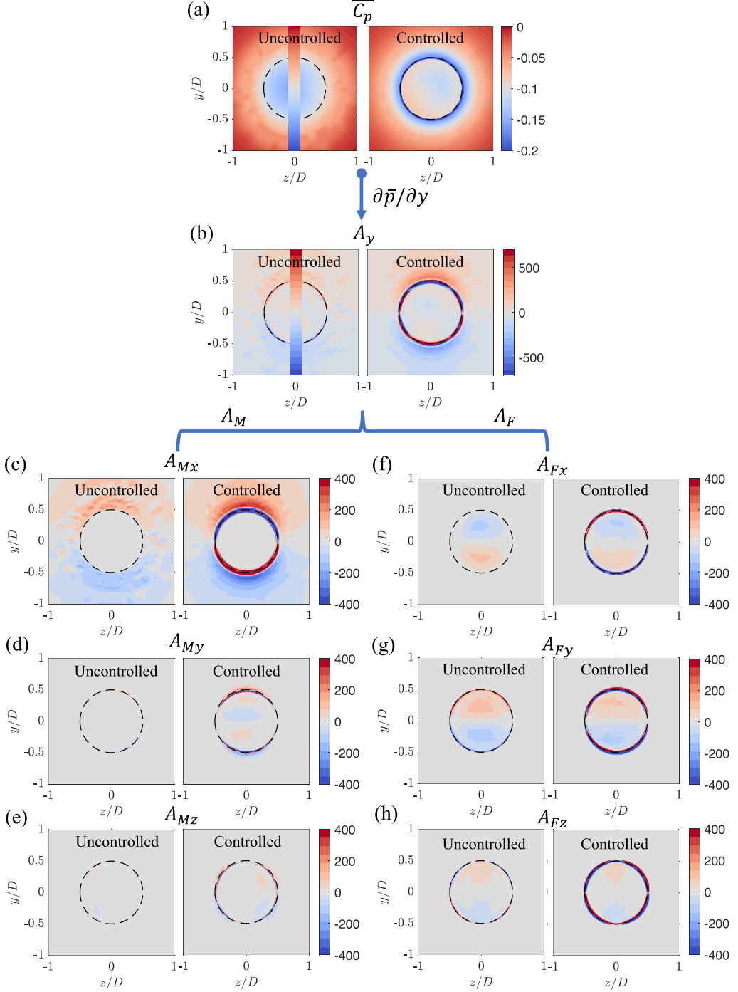
FIG. 11. The distribution of the pressure field, the pressure gradient, and the momentum budget terms close to the base (y-z plane at x/D = 0.025 ). (a) The time-averaged pressure field \bar{C}_p . (b) The y component pressure gradient \partial \bar{p} / \partial y . The acceleration terms contributing to the pressure gradient, including (c) A_{Mx} , (d) A_{My} , (e) A_{Mz} , (f) A_{Fx} , (g) A_{Fy} , and (h) A_{Fz} . In each subfigure, the left column shows the uncontrolled wake and the right column shows the controlled one. The units of the pressure gradient contour are Pa/m.
