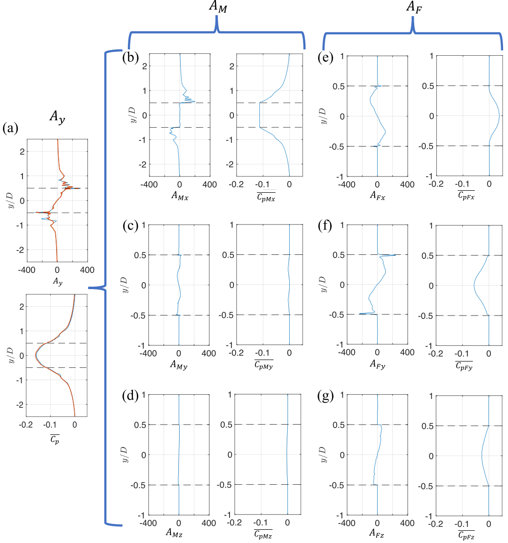
FIG. 12. The distribution of the pressure gradient and integrated pressure from each momentum budget along the integration path ( x/D = 0.025 ). The base edge ( y/D = \pm 0.5 ) is marked by the black dashed lines. In panel (a), the blue curve is from 3D LES, and the red dashed one is calculated from Eqs. (2) and (4). The units of the pressure gradient are Pa/m.
