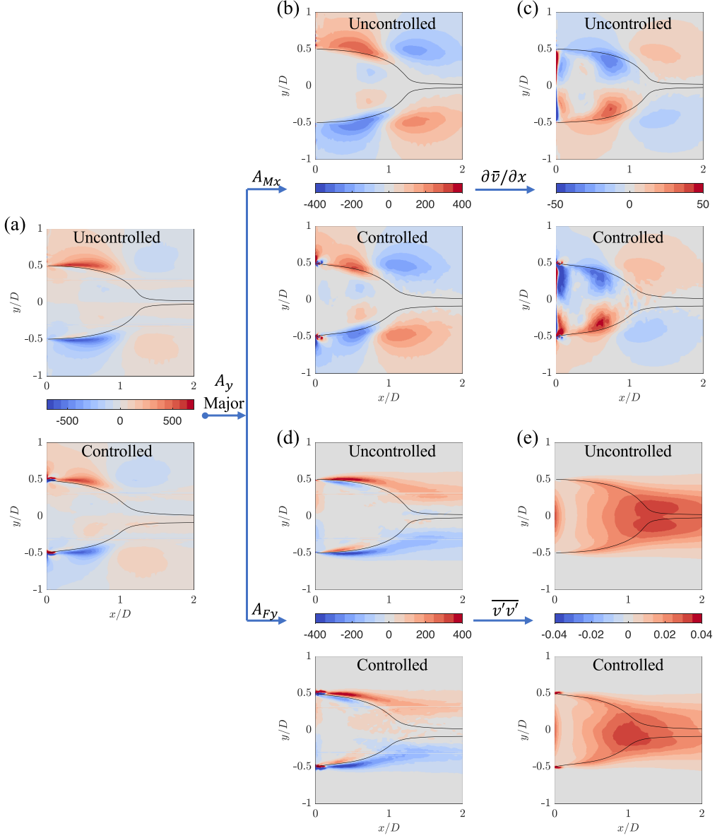
FIG. 15. A x - y slice view of (a) the y component pressure gradient, the major momentum budgets (b) A_{Mx} and (d) A_{Fy} , the term component (c) \partial \bar{v}/\partial x , and (e) \overline{v'v'} . In each subfigure, the upper side is the uncontrolled wake and the lower side is the controlled wake. The units of the pressure gradient are Pa/m. The black curve marks the separation streamline.
