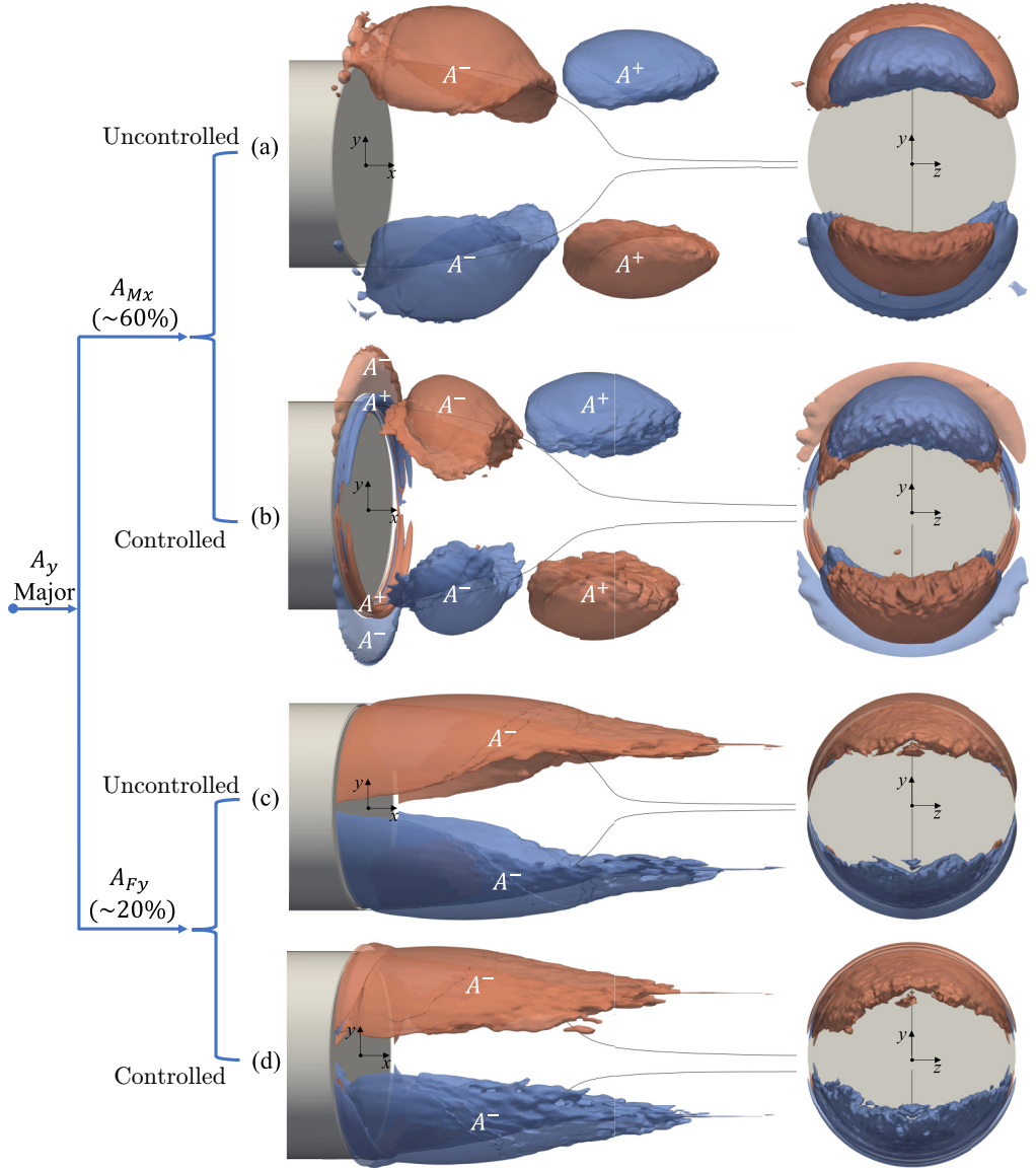
FIG. 9. Three-dimensional distribution of the major momentum budgets identified by A_n D/U_\infty^2 = 0.11 (red) and A_n D/U_\infty^2 = -0.11 (blue). A_{Mx} for (a) the uncontrolled wake and (b) the controlled wake, and A_{Fy} for (c) the uncontrolled wake and (d) the controlled wake. The left and right columns show side views perpendicular to the x - y and the y - z planes, respectively. The black curve marks the separation streamline originating from y/D = \pm 0.5 , x/D = 0 , z/D = 0 . The white A^+ and A^- indicate pressure rise and drop toward the wake, respectively.
