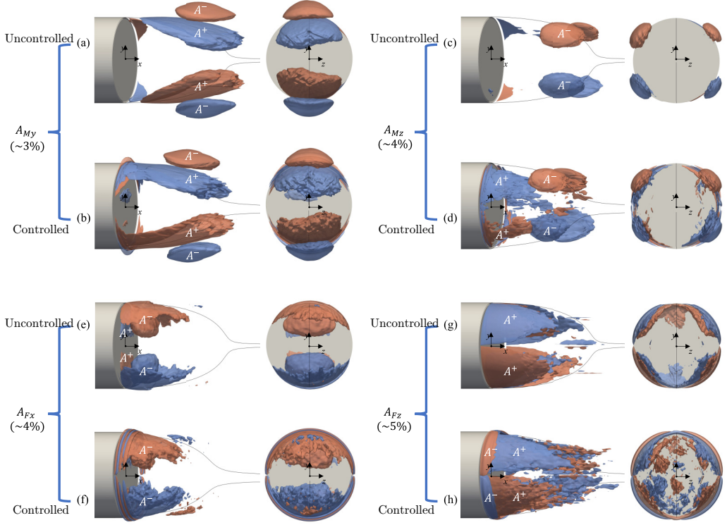
FIG. 10. Three-dimensional distribution of the minor momentum budgets identified by A_n D/U_\infty^2 = 0.035 (red) or A_n D/U_\infty^2 = -0.035 (blue). A_{My} for (a) the uncontrolled wake and (b) the controlled wake, A_{Mz} for (c) the uncontrolled wake and (d) the controlled wake, A_{Fx} for (e) the uncontrolled wake and (f) the controlled wake, and A_{Fz} for (g) the uncontrolled wake and (h) the controlled wake. The left and right columns in each subfigure show side views perpendicular to the x - y and the y - z planes, respectively. The black curve marks the separation streamline originating from y/D = \pm 0.5 , x/D = 0 , z/D = 0 . The white A^+ and A^- indicate pressure rise and drop toward the wake, respectively.
