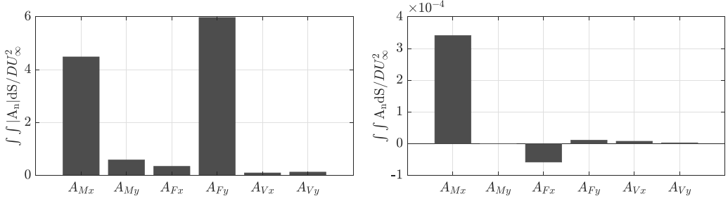
FIG. 5. The contribution of each momentum budget to the overall pressure gradient, evaluated with the absolute value (left figure, given by \iint |A_n| dS / DU_\infty^2 ) and the signed true value (right figure, given by \iint A_n dS / DU_\infty^2 ).
