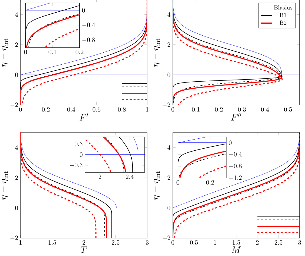
FIG. 5. First (top left) and second derivative (top right) of F as a function of \eta for a supersonic flow at \text{Ma} = 3 . The static temperature T and the local Mach number M are shown in the bottom-left and bottom-right plots, respectively. The black and red curves show cases B1 and B2, respectively, for \theta_{fp} = 0.85 (solid) and \theta_{fp} = 0.95 (dashed). The Blasius solution over a nonpermeable wall is plotted in blue for comparison. The top boundary of the interfacial region is located at \eta_{\text{int}} (blue line), while the bottom one is marked by the horizontal lines for each case.
