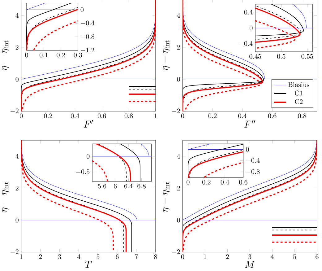
FIG. 6. First (top left) and second derivative (top right) of F as a function of \eta for a supersonic flow at Ma = 6 . The static temperature T and the local Mach number M are shown in the bottom-left and bottom-right plots, respectively. The black and red curves show cases C1 and C2, respectively, for \theta_{fp} = 0.85 (solid) and \theta_{fp} = 0.95 (dashed). The Blasius solution over a nonpermeable wall is plotted in blue for comparison. The top boundary of the interfacial region is located at \eta_{int} (blue line), while the bottom one is marked by the horizontal lines for each case.
