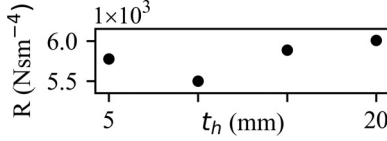
FIG. 4. Porous medium static air-flow resistivity R from the experimental calibration data of a DMND porous material with a cell size d_c of 2.5 mm [28].
