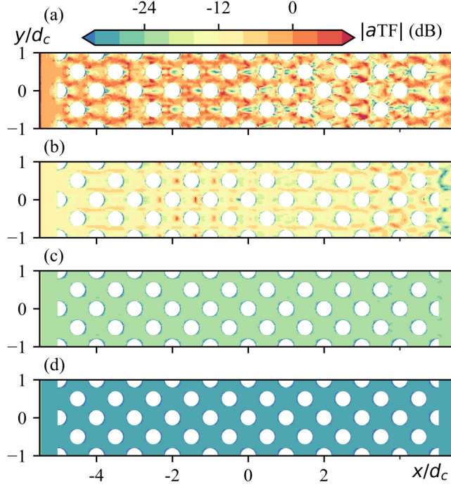
FIG. 15. Contours of the normalized local TF amplitude for inflow pressure oscillation frequencies of (a) 0.3 kHz, (b) 1 kHz, (c) 4 kHz, and (d) 9 kHz.
