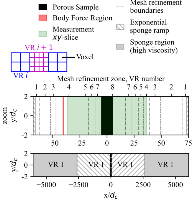
FIG. 5. Simulation domain diagram. The upper figure is a detail of the lower figure, focused on the region around the sample. The limits of the lower figure indicate the simulation domain. The variable resolution (VR) region indices i are provided and explained in the mesh diagram. The local voxel size is l_{\text{voxel},i} = d_c/2^{i-2} .
