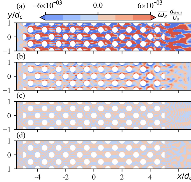
FIG. 14. Contours of the mean band-passed normalized vorticity around the z -axis \omega_z d_{\text{strut}}/U_0 . The presented cases are (a) f_p = 0.3 kHz, (b) f_p = 1 kHz, (c) f_p = 4 kHz, and (d) f_p = 9 kHz. Each case is band passed in a frequency band of f_p \pm 50 Hz.
