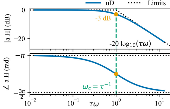
FIG. 2. Frequency response of the normalized uD equations [Eq. (7)].
