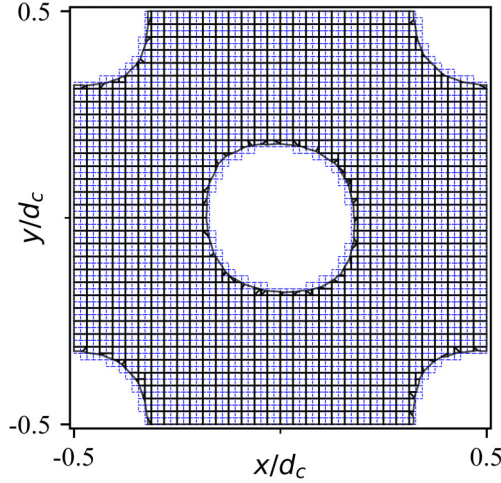
FIG. 6. Detail of the mesh for a single REV, showing a slice on the xy plane at z/d_c = 0 . The thin blue dashed lines indicate the voxel mesh, and the thick black solid lines indicate the xy -slice measurement file mesh at half the resolution of the volume mesh.
