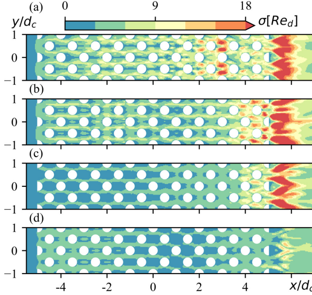
FIG. 13. Contours of the local standard deviation of the strut-based Reynolds number \sigma[Re_d] . The presented cases are (a) f_p = 0.3 kHz, (b) f_p = 1 kHz, (c) f_p = 4 kHz, and (d) f_p = 9 kHz.
