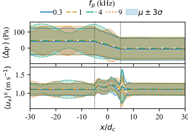
FIG. 10. Spatial evolution of the volume-averaged static pressure and x -axis velocity along the x axis on the xy plane of the LBM simulation performed with different oscillation frequencies f_p . The local mean (lines) and signal bands (filled areas) of each case are shown in the same color. The signal bands are formed by three standard deviations around the mean, i.e., \mu \pm 3\sigma . The vertical dotted black lines indicate the spatial extent of the porous material sample. The gauge pressure is defined with respect to the atmospheric outlet pressure.
