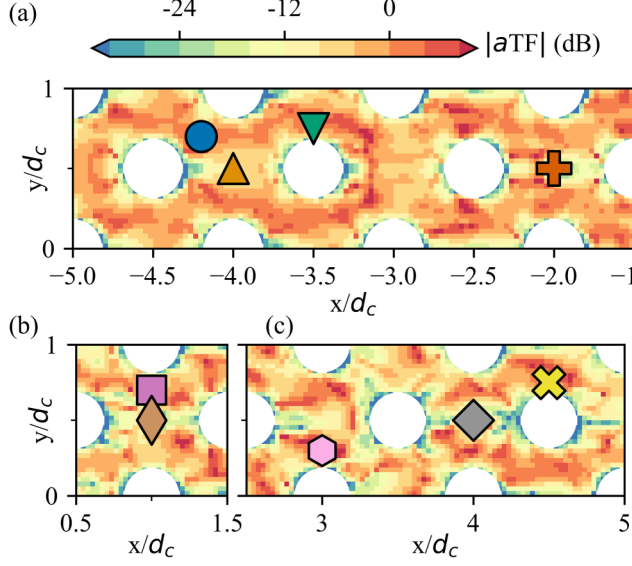
FIG. 16. Contours of normalized local TF amplitude for the case of f_p = 0.3 kHz. The markers indicate the positions of the probed frequency responses plotted in Fig. 17. Shown are the TF contours for different streamwise locations: (a) x/d_c \in [-5, -1] , (b) x/d_c \in [0.5, 1.5] , and (c) x/d_c \in [2.5, 5] .
