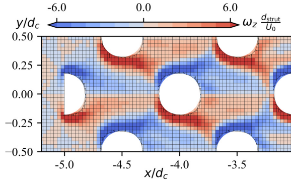
FIG. 8. Time instant of vorticity with the “half resolution” xy -slice measurement file mesh.
