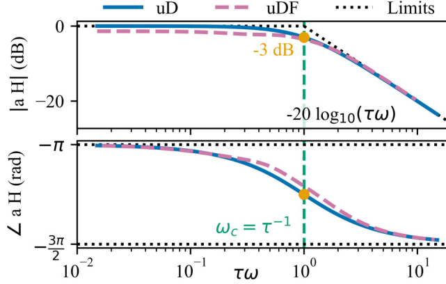
FIG. 22. Frequency response of the normalized uD and uDF equations. The Forchheimer term is estimated with 10 additional Adomian polynomial terms ( n = 10 ). The initial velocity u(0) is set to 0 \text{ ms}^{-1} [Eq. (B5)].
