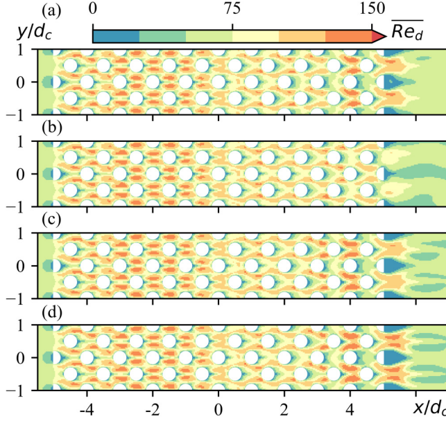
FIG. 12. Contours of the mean local of the strut-based Reynolds number \overline{Re_d} . The presented cases are: (a) f_p = 0.3 kHz, (b) f_p = 1 kHz, (c) f_p = 4 kHz, and (d) f_p = 9 kHz. The vertical extent of the contour is limited to y/d_c \in [-1, 1] for clarity.
