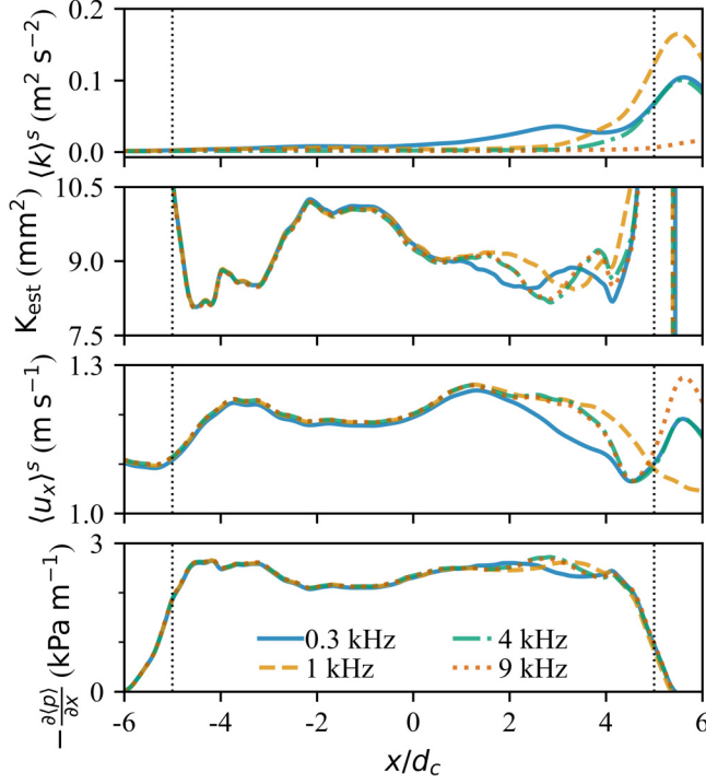
FIG. 11. Streamwise evolution of mean volume-averaged flow turbulent kinetic energy k , velocity, pressure gradient, and estimated local Darcy-equivalent permeability u_x \mu / (-\partial_x p) . The vertical black dotted lines indicate the start and end of the porous material.
