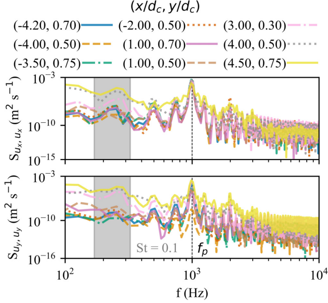
FIG. 18. Power spectral density S_{u_i, u_i} of the flow velocity components in the probe points of Fig. 17 for the inflow oscillation case f_p = 1 kHz. The natural shedding frequency band of the porous struts is estimated based on the local flow magnitude in the probe point and St = 0.1 .
