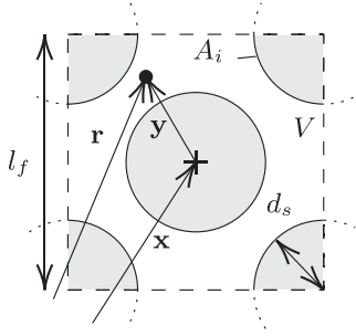
FIG. 1. Diagram of averaging volume V in a structured porous material. The solid phase is indicated in gray and the fluid phase in white. Based on the diagram of Breugem [13, p. 61].
