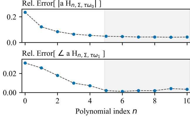
FIG. 21. Convergence of the frequency response H_n [Eq. (5)] with increasing number of corrective terms U_n [Eq. (B6)]. The amplitude is probed at \tau\omega_0 = 2 \times 10^{-2} and the phase is probed at \tau\omega_1 = 5 \times 10^{-1} . The response H_{n,\Sigma} is the sum of all terms up to and including term n . The relative error is defined with respect to the mean amplitude and phase values inside the gray-filled region.
