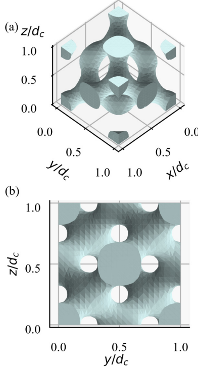
FIG. 3. REV of the altD porous material with a cell size d_c of 2 mm. (a) Isometric view. (b) yz -plane view.
