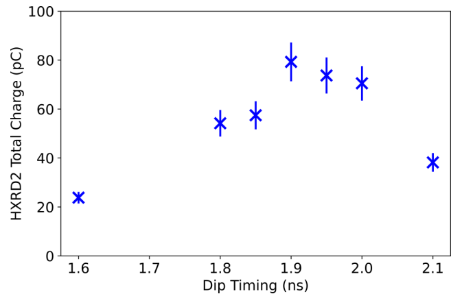
FIG. 9. Charge accumulated in the second channel of the HXR2 diagnostic. Greater charge implies a larger population of hot electrons which can preheat the shell and limit peak areal density.
