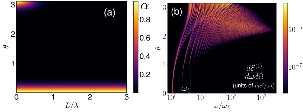
FIG. 2. Coherence factor (a) and radiation spectrum of a single particle (b) for a head-on collision of electrons with a plane wave laser pulse; \omega_1 is the fundamental harmonic of the backward radiation defined in Eq. (21); R = \lambda , p_0 = 5mc , T \approx 50 fs.
