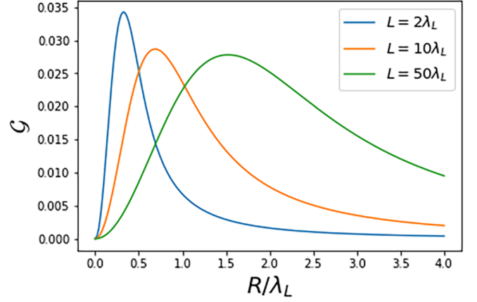
FIG. 5. Geometric factor \mathcal{G} , Eq. (30), vs bunch width R for three values of the bunch thickness L .
