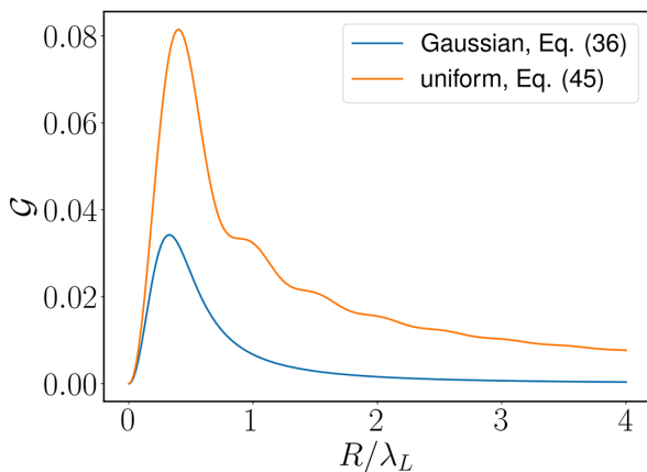
FIG. 7. Geometric factors for Gaussian and uniform distributions of the bunch density.
