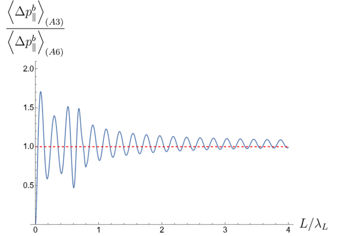
FIG. 8. Ratio of the backward contribution to the momentum loss evaluated numerically via Eq. (A3) and analytically via Eq. (A6) for \omega_L T = 5\pi .
