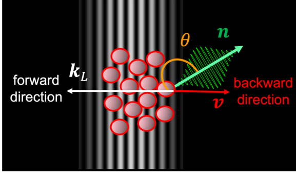
FIG. 1. Illustration of the laser-bunch collision geometry; \mathbf{k}_L —laser wave-vector; \mathbf{v} —velocity of the particles; \mathbf{n} —direction of radiation.
