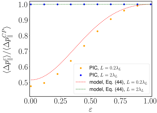
FIG. 6. Dependence of the momentum loss on laser polarization. Parameters: a_0 = \gamma_0 = 5 , T \approx 17 fs, R = 2\lambda_L , n = 0.1n_c .
