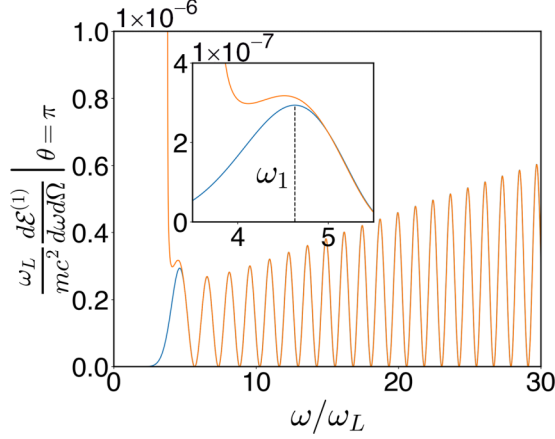
FIG. 3. Single-particle radiation spectrum in backward direction evaluated numerically (blue) and its analytical approximation Eq. (19) (orange). Other parameters: a_0 = \gamma_0 = 5 , T = 67 fs, \lambda_L = 1 \mu\text{m} . Inset: the same plot zoomed in near the first maximum \omega_1 .
