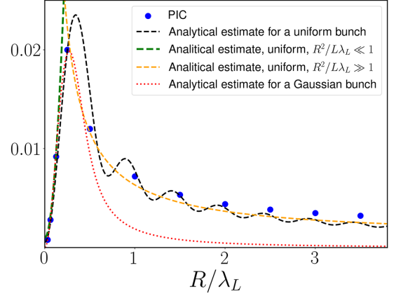
FIG. 10. Normalized particle deceleration \langle \Delta p_{\parallel} \rangle / p_0 vs bunch width R for a cylindrical bunch of uniform density distribution. Blue dots are extracted from 3D PIC simulations. Dashed curves correspond to the sum of Eq. (29) + Eq. (A6) with \mathcal{G} from Eqs. (45) (black), (A7c) (orange), and (A7d) (green). Red dotted curve corresponds to the Gaussian estimate (29) with \mathcal{G} from Eq. (36) multiplied by a scale factor of 2. Other parameters are a_0 = 5 , \omega_L T = 5\pi , n = 0.1n_c , and L = \lambda_L .
