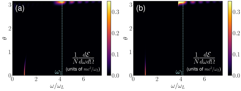
FIG. 4. Per-particle radiation spectrum of the Gaussian particle bunch [see Eq. (11)] of length L = 0.1\lambda_L , radius R = 0.5\lambda_L , n = 0.01n_c , and Lorentz factor \gamma = 5 , colliding head on with a plane wave laser pulse with the Gaussian envelope equation (13), a_0 = 5 , \omega_L T = 15\pi (50 fs). (a) numerical evaluation of Eq. (6), (b) analytical estimate equation (24).
