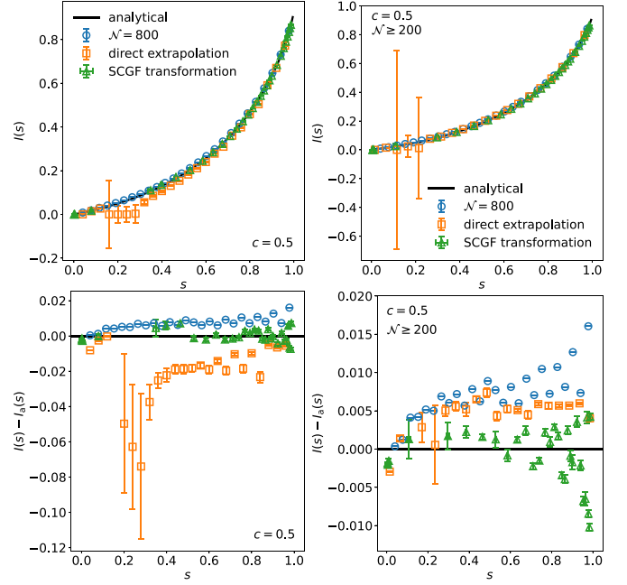
FIG. 8. The left column shows analysis results that include data points at all simulated system scales, while the right column only considers graph sizes where \mathcal{N} \geq 200 . Top row: Comparison of the analytical rate function in Eq. (24), the Legendre-Fenchel transformed extrapolated SCGF (see Sec. II C), the empirical rate function at system size \mathcal{N} = 800 (see Sec. II A), and the directly extrapolated empirical rate function (see Sec. II B) for the Erdős-Rényi random graph ensemble. The connectivity is c = 0.5 . The gap in the transformed SCGF curve at s \approx 0.25 is due to the finite-size apparent first-order phase transition of the biased graph ensemble at this point and the resulting breakdown of the assumed scaling power law in Eq. (13) used for extrapolation. Bottom row: Corresponding residuals, highlighting the difference between the presented estimation methods and the exact analytical solution. For visual purposes, the data point with the largest error value is omitted in the left plot, and likewise, the two data points with the largest errors in the right plot.
