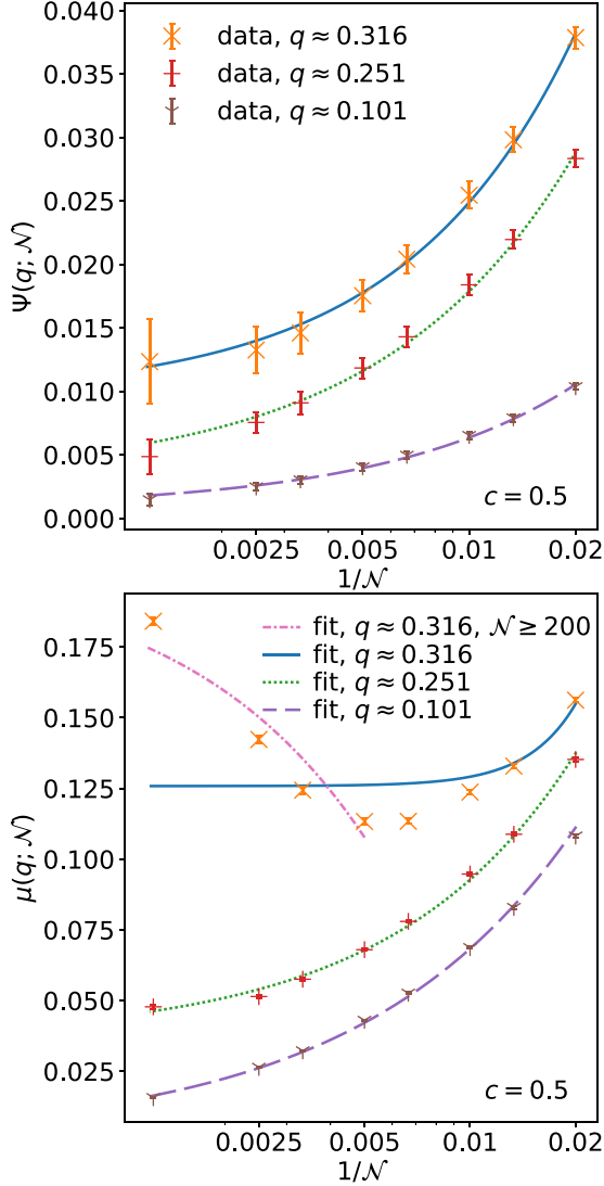
FIG. 7. Infinite system size \mathcal{N} extrapolation fit by means of the power law in Eq. (13) for the largest connected component in the Erdős-Rényi random graph ensemble with connectivity c = 0.5 . Curves for a selection of bias values q are shown together with the corresponding fits. Top: SCGF \Psi(q; \mathcal{N}) . Bottom: Biased expectation value \mu(q; \mathcal{N}) . The scaling behavior for q \approx 3.17 shows substantial deviations from that of a power law. Also shown is a fit at q \approx 3.17 only including data values with \mathcal{N} \geq 200 . Fit parameters are summarized for both panels in Table II under Appendix C.
