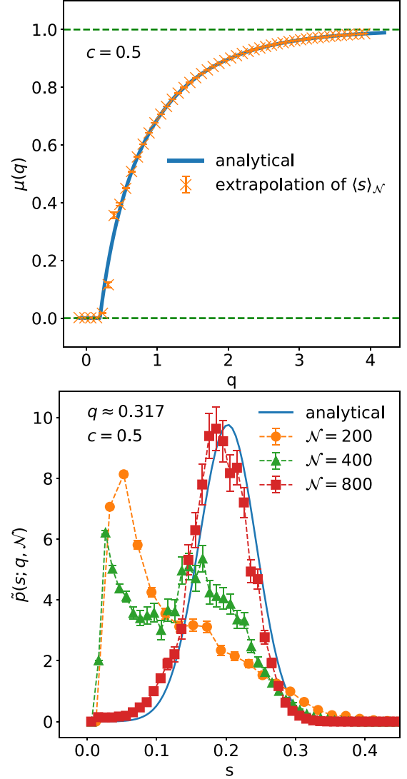
FIG. 6. Top: For connectivity c = 0.5 , analytical and extrapolated relative size \mu(q) of the largest connected component of the Erdős-Rényi random graph ensemble. The extrapolation is according to Eq. (13). The dashed horizontal lines indicate the limiting values of the expectation value \mu(q) for q \rightarrow \pm\infty . The gap at q \approx 0.3 for the extrapolated curve is caused by an apparent first-order phase transition in the corresponding biased ensemble, resulting in deviations from the assumed power-law scaling behavior. Bottom: Biased distribution of the largest connected component relative size at q \approx 0.317 . The apparent phase transition is indicated by the double peak structure that vanishes for increasing graph order \mathcal{N} . For comparison, the analytical curve is shown, too, which is given by \tilde{p}(s; q, \mathcal{N}) \sim \exp(-800 I(s)) \exp(800 q s) with rate function I(s) from Eq. (24). Lines are a guide to the eye only.
