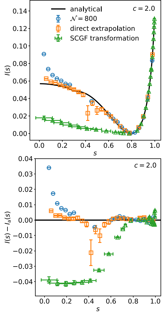
FIG. 10. Top: Plot of the analytical rate function in Eq. (24), the Legendre-Fenchel transformed extrapolated SCGF (see Sec. II C), the empirical rate function at system size \mathcal{N} = 800 (see Sec. II A), and the directly extrapolated empirical rate function (see Sec. II B) for the Erdős-Rényi random graph ensemble. The connectivity is c = 2.0 . The transformed SCGF is only located below the convex envelope of the true rate function in the regime s \approx 0.3 \dots 0.75 . There, the analytical rate function is partially concave. Bottom row: Corresponding residuals, highlighting the difference in the presented estimation methods and the exact analytical solution.
