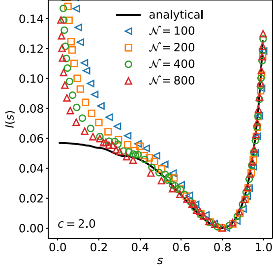
FIG. 9. For the Erdős-Rényi random graph ensemble at connectivity c = 2.0 , the analytical rate function in Eq. (24) and empirical rate functions at various system scales \mathcal{N} (see method under Sec. II A). While the analytical curve is already matched for values s \geq 0.8 by the curves at finite system sizes \mathcal{N} , the convergence at smaller values of s is slower.
