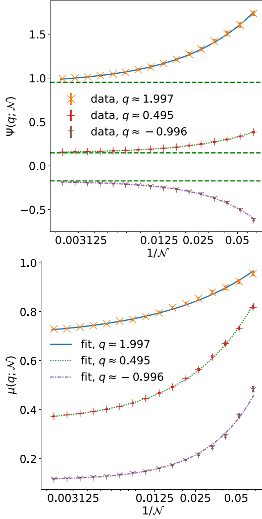
FIG. 3. Fit of the power law in Eq. (13) for the binomial distributed data to extrapolate toward infinite system sizes N . Curves for a selection of bias values q are shown together with the corresponding fits. Top: SCGF \Psi(q; N) . Also shown are the correct limiting values according to Eq. (18) as dashed horizontal green lines. Bottom: Biased expectation value \mu(q; N) . Fit parameters are summarized for both panels in Table I under Appendix C.
