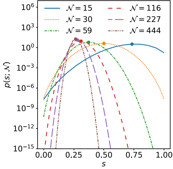
FIG. 1. Normalized binomial distributions with scale-dependent parameter r(\mathcal{N}) as given in Eq. (16). In contrast to a binomial distribution with a constant value of r(\mathcal{N}) , the mean and variance change with the system scale \mathcal{N} . The circles mark the corresponding distribution maximum. Only a selection of system scales \mathcal{N} is shown for visual purposes.
