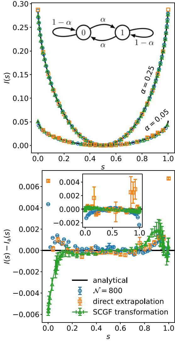
FIG. 5. Top: Comparison of the analytical rate function in Eq. (24), the Legendre-Fenchel transformed extrapolated SCGF (see Sec. II C), the empirical rate function at system size \mathcal{N} = 800 (see Sec. II A), and the directly extrapolated empirical rate function (see Sec. II B) for the two-state Markov process case study with transition probabilities \alpha = 0.25 and \alpha = 0.05 . The inset shows the state transition diagram of the Markov chain. Bottom: Corresponding residuals (main plot: \alpha = 0.25 , inset \alpha = 0.05 ), highlighting the differences of the presented estimation methods to the exact analytical solutions.
