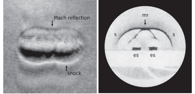
FIG. 8. Mach reflection of shocks generated by the two-lobed plasma kernel of a laser-induced breakdown plasma. (Left, reproduced from Fig. 4 at 250 \text{ ns} ) Schlieren image of the shocks generated by the two-lobed plasma kernel. (Right) First visualization of the interaction of shocks by Ernst Mach. Two spherical shocks ( s ) are generated by two electric sparks ( es ) near a glass plate. The interacting shocks generate a third shock known as a Mach reflection ( mr ). Reproduced from Ref. [57] with permission of Wiley-VCH GmbH. Copyright © 1890 Wiley-VCH GmbH. All rights reserved, including rights for text and data mining and training of artificial intelligence technologies or similar technologies.
