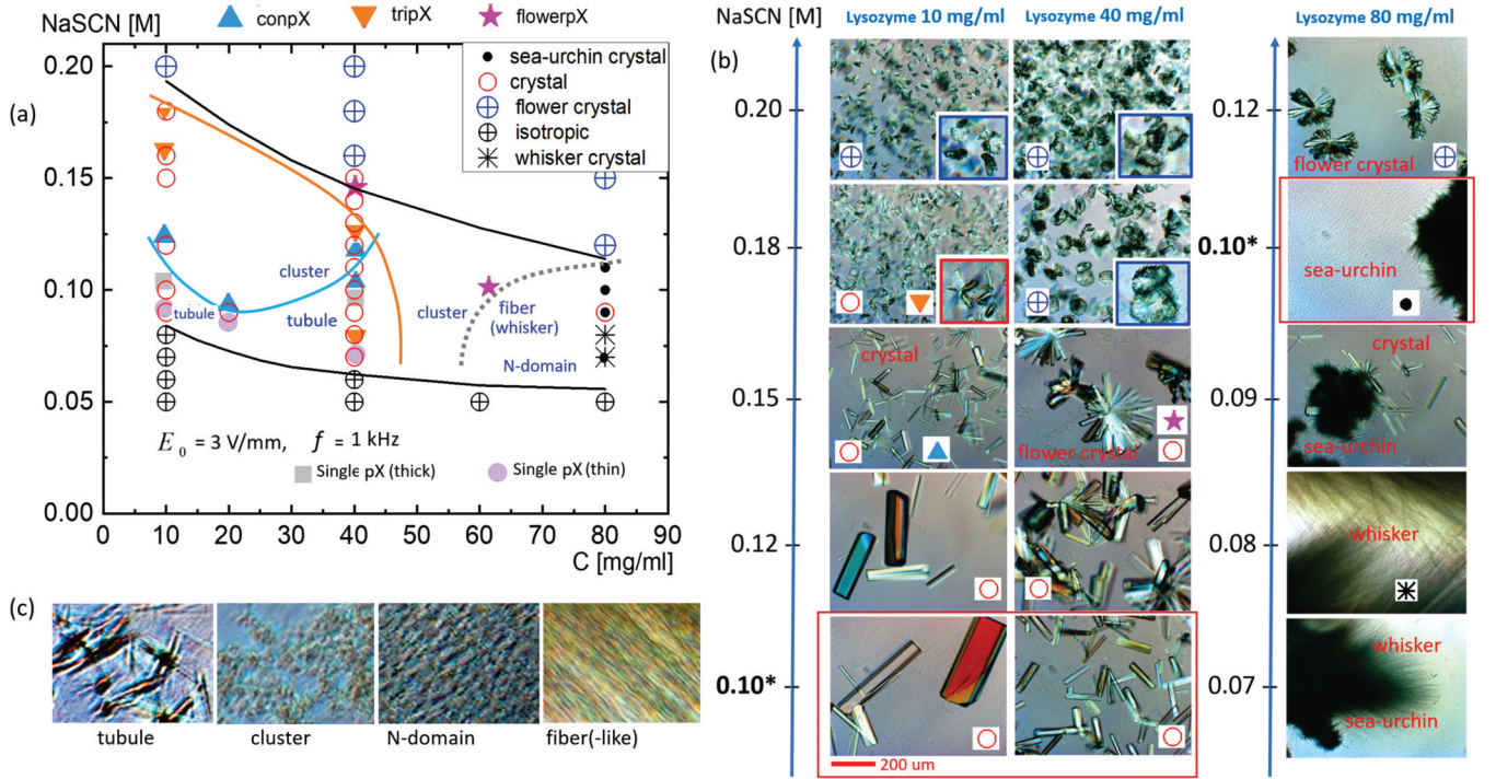
FIG. 1. Protein crystal morphologies under a given electric field: (a) Morphology-state diagram of lysozyme protein vs NaSCN concentration under an applied electric field of amplitude E_0 = 3 \text{ V/mm} and frequency f = 1 \text{ kHz} . The category labeled “crystals” in Ref. [33] is here refined into two subtypes: single-arm protein crystals (single pXs) and multi-arm protein crystals (multiarm pXs). The latter are further subdivided into three representative morphologies: conic pX (conpX), triconic pX (tripX), and flower pX (flowerpX), as discussed in the main text. Colored lines serve as guides to the eye, indicating regions where each multiarm morphology predominates, as discussed in the main text: blue (distinction between conpX and tripX), orange (distinction between tripX and flowerpX), and dotted black lines (distinction between flowerpX and fiber). The black lines mark the crystallization boundary (lower) and the liquid-liquid phase separation (LLPS) line (upper). (b) Representative polarized-light microscope images of crystal morphologies at selected NaSCN and protein concentrations (10 mg/ml, 40 mg/ml, and 80 mg/ml, as indicated). The thin red rectangles highlight the case of 0.1 M NaSCN detailed later. (c) Microscopy images of field-driven metastable morphologies observed near the crystallization boundary. These include tubules, clusters, nematic (N) domains, and fiber structures, which appear as protein concentration increases from left to right. The approximate regions where these morphologies occur are labeled in the morphology-state diagram (a).
