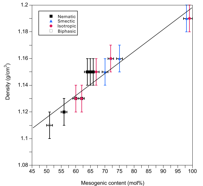
FIG. 1. The density of materials templated in the nematic (black squares), smectic (blue triangles), and isotropic (pink circles) phases. A phase-separated nematic LCE is also included (empty black square).
