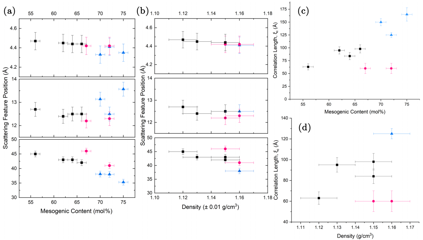
FIG. 3. Network spacings measured for side-to-side, EHA-related and end-to-end periodicities ( \sim 4.4 \text{ \AA} , \sim 12 \text{ \AA} , and \sim 45 \text{ \AA} , respectively) for the monodomain nematic (black squares), isotropic (pink circles), and smectic (blue triangles) LCEs, measured as a function of (a) the mesogenic content and (b) the density of the LCE. The correlation lengths parallel to the director, \xi_{||} , for monodomain nematic (black squares) and smectic (blue triangles) LCEs as a function of (c) mesogenic content and (d) the density of the LCE, with the correlation lengths of the isotropic LCEs (pink circles) also included.
