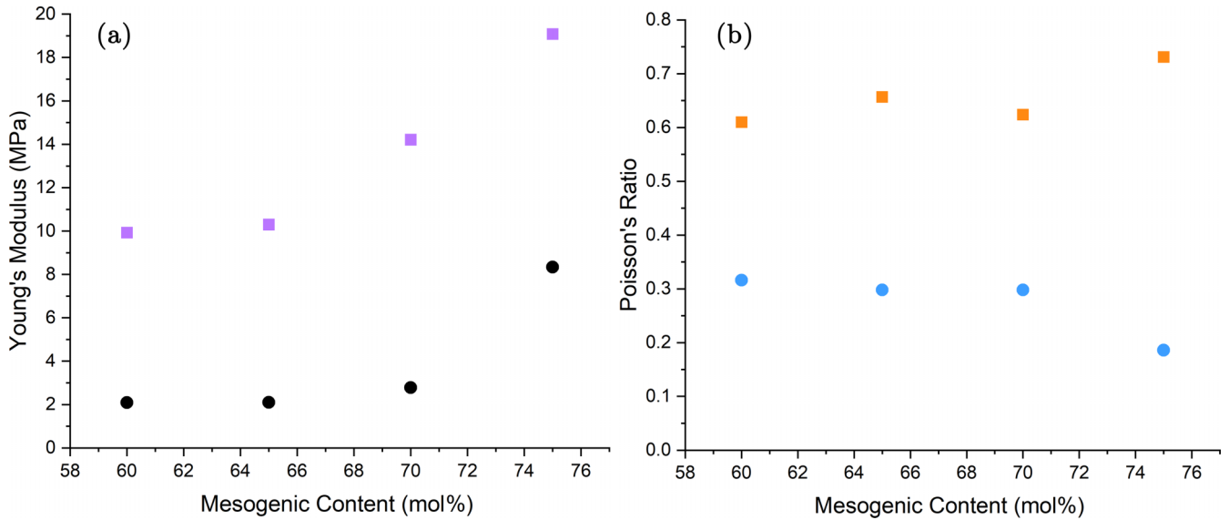
FIG. 4. (a) Young's moduli measured for LCEs between 60 mol% and 75 mol% mesogenic content, with the applied stress parallel (purple squares) and perpendicular (black circles) to the director. (b) Poisson's ratios for different concentrations of mesogenic content when the applied stress is along the z axis and parallel to the director (defined in the Supplemental Material [33]). The blue circles and orange squares represent \sigma_{\parallel x} and \sigma_{\parallel y} , respectively. All measurements were taken at 21 °C.
