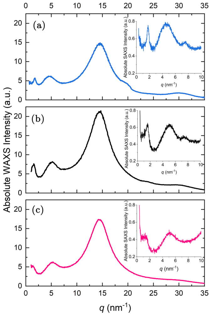
FIG. 2. Wide- and Small-Angle X-ray Scattering intensity from (a) sLCE-75, (b) nLCE-66, and (c) iLCE-67.
