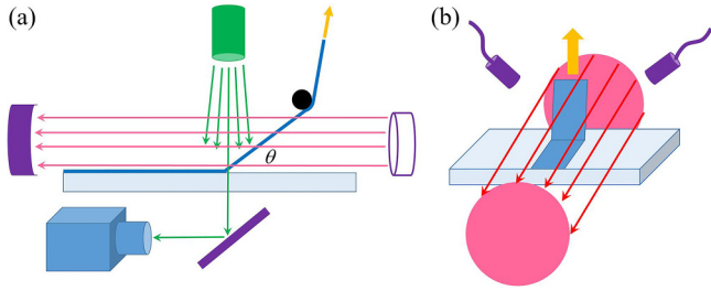
FIG. 1. Sketches of the experimental setup. (a) Side view with the bottom-view camera. (b) Front view with the collimated schlieren light shone along the glass plate and the placement of the two microphones, positioned one on each side of the tape. More detailed drawing and photographs are included in the Supplemental Material [17].
