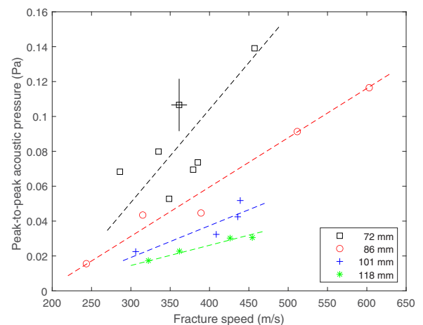
FIG. 5. Peak-to-peak sound pressure vs the observed fracture speed, measured with the microphone at different distances from the edge of the tape.
