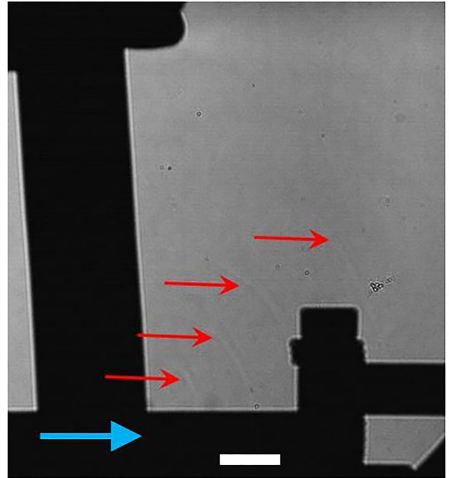
FIG. 4. Schlieren frame from a high-speed video clip, taken at 2 000 000 fps with a 100 ns exposure. It shows four weak shock fronts (marked by the red arrows) emerging from the right side of the tape. The fractures are traveling from left to right as indicated by the cyan arrow. Their frequency of appearance here is approximately 37 kHz. See also Video 2 in the Supplemental Material [17]. The white scale bar is 10 mm long.
