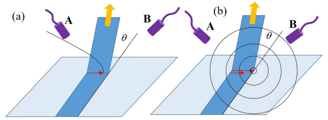
FIG. 2. Sketches of the two proposed competing sound generation mechanisms. (a) The tip of the supersonic crack produces a shock wave into the air. (b) The actual observed mechanism, where the sound shocks are generated when each crack reaches the edge of the tape.
