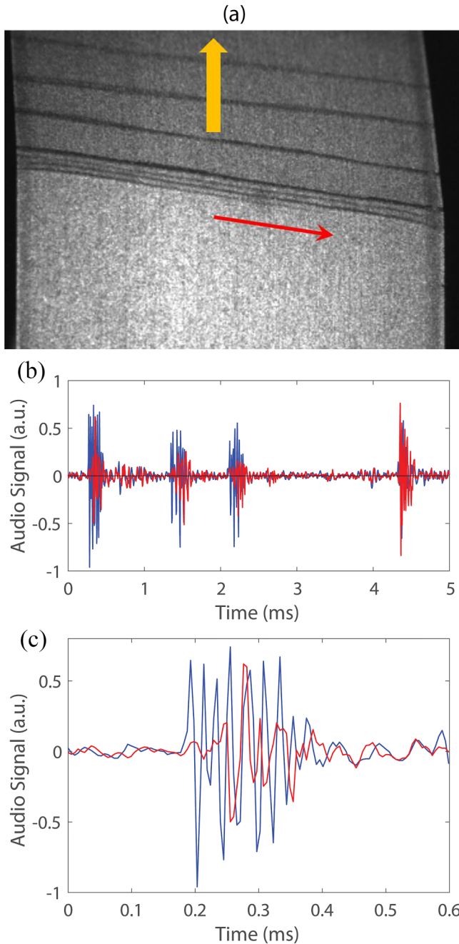
FIG. 3. Simultaneous video capture and sound recordings during a typical rapid stick-slip peeling of the tape. (a) Video frame taken through the bottom glass plate, showing typical transverse fractures traveling from left to right as indicated by the red arrow. The orange arrow shows the pulling direction of the detached section of the tape. For scale, the attached part of the tape is 19 mm wide. The frame is taken from a 96011 fps video clip, which is included in the Supplemental Material [17]. (b) Audio signals from the two microphones, positioned one on each side of the tape. The blue curve corresponds to the microphone closer to the right edge of the tape, where the fractures end, while the red curve is for the one on the left side. (c) Close-up view of the first slip phase in (b).
