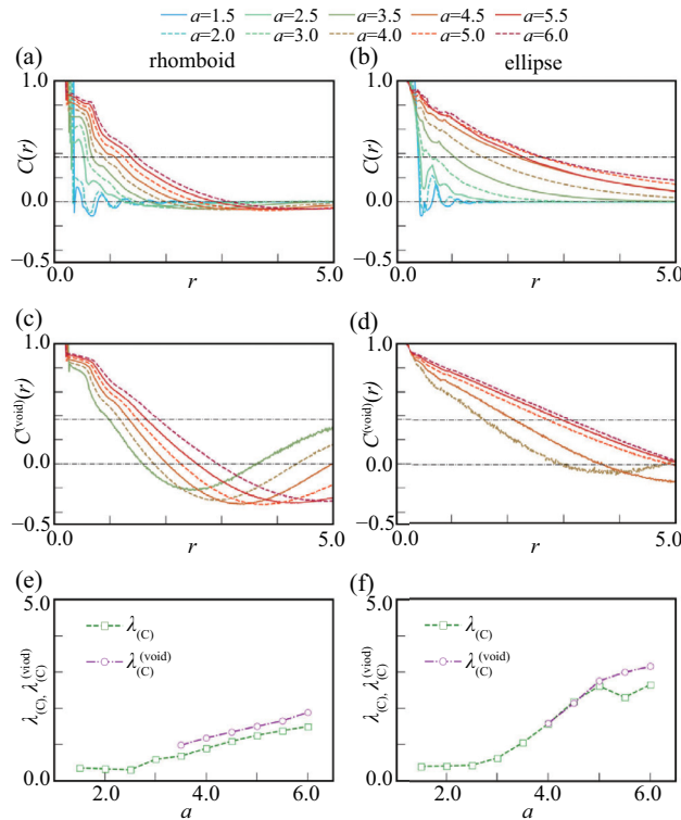
FIG. 8. (a), (b) Spatial correlation of the particle orientation C(r) in the whole region for the systems with (a) rhomboidal and (b) elliptical particles. (c), (d) Spatial correlation of the particle orientation for particle pairs located around the same void regions C^{(void)}(r) for the systems with (c) rhomboidal and (d) elliptical particles. (e), (f) Correlation lengths in the whole region \lambda_{(C)} and those for particle pairs located around the same void regions \lambda_{(C)}^{(void)} depending on the aspect ratio a for the systems with (e) rhomboidal and (f) elliptical particles.
