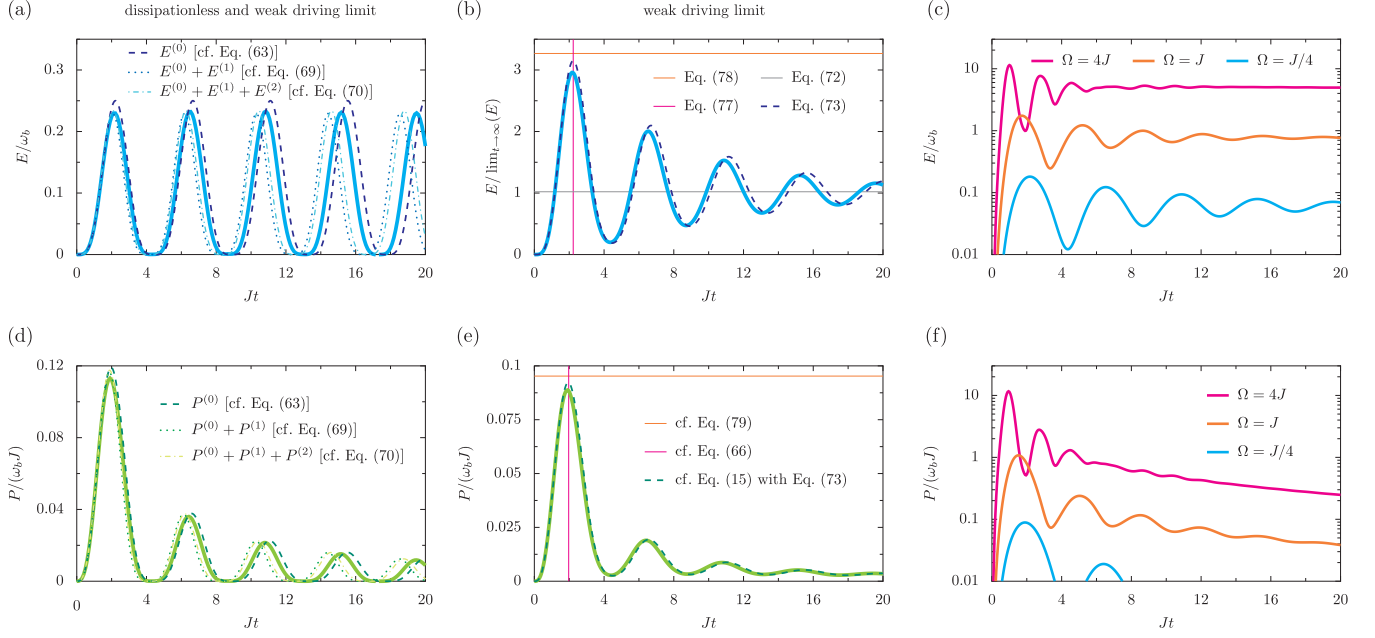
FIG. 3. Dynamics of the quantum battery with nonlinear coupling. (a) The energy E stored in the quantum battery in the dissipationless limit (solid cyan line) and in units of the energy level spacing \omega_b , as a function of time t (in units of 1/J , the inverse of the coupling rate J ). Dashed, dotted, and dashed-dotted lines: three approximate results, derived with perturbation theory of increasing order [cf. Eq. (62), along with Eqs. (63), (69), and (70)]. (b) The stored energy E (solid cyan line) in units of the steady state energy, within the weak driving regime \Omega \ll J . Dashed blue line: the approximate behavior [cf. Eq. (73)]. Vertical pink line: the optimal charging time t_E [cf. Eq. (77)]. Horizontal orange line: the approximate maximum stored energy E(t_E) [cf. Eq. (78)]. Thin grey line: the approximate steady state energy \lim_{t \rightarrow \infty}(E) [cf. Eq. (72)]. (c) a semilogarithmic plot of the dynamic energy E in units of \omega_b . (d), (e), (f) the charging power P of the quantum battery, in units of \omega_b J , corresponding to the stored energies of (a), (b), (c) respectively [cf. Eq. (15)]. In (e), the vertical pink line corresponds to the optimal charging time t_P [cf. Eq. (66)] and the horizontal orange line represents the maximum power P(t_P) [cf. Eq. (79)]. Within this figure, in the first two columns \Omega = J/4 and in the final two columns \gamma = J/2 .
