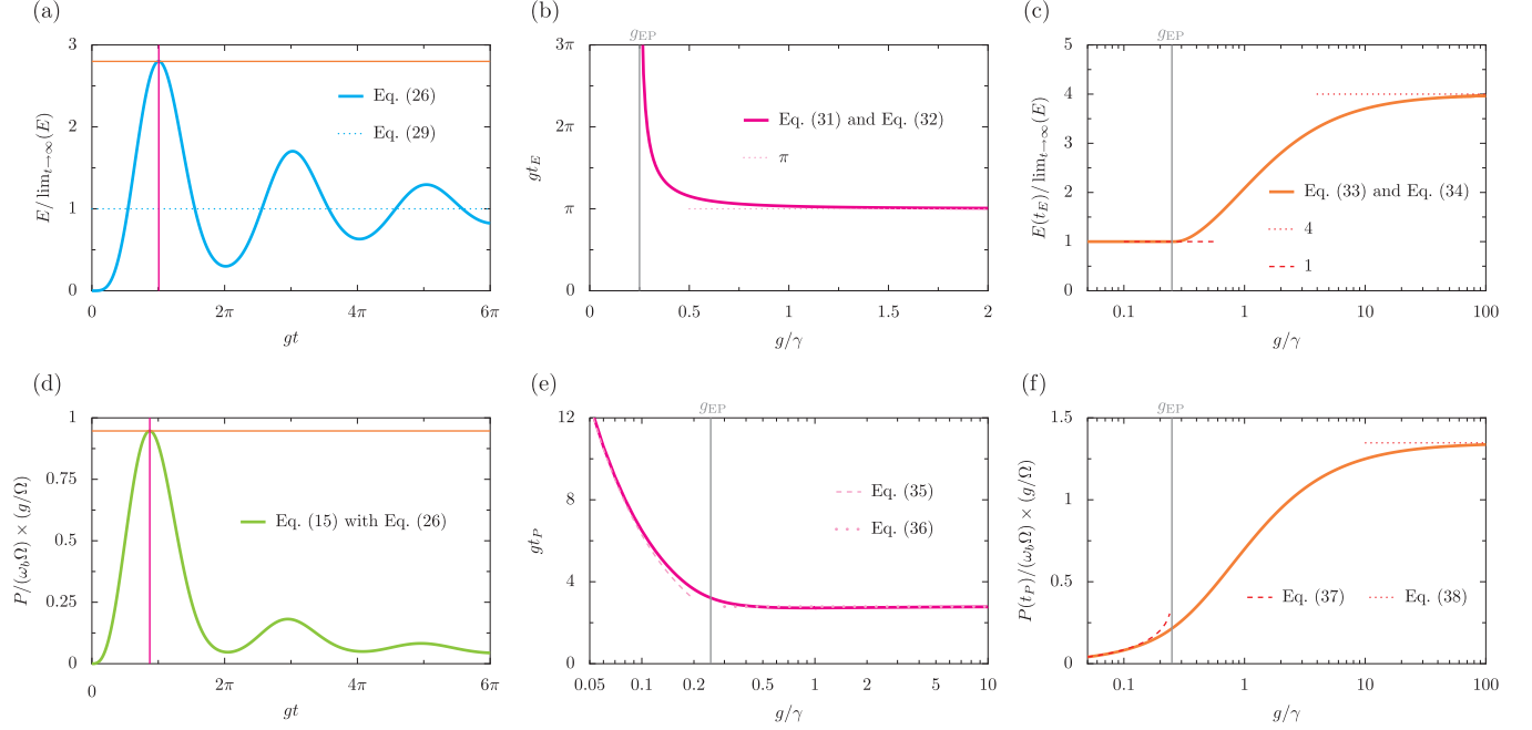
FIG. 2. Performance of the quantum battery with linear coupling. (a) The energy E (cyan line) stored in the quantum battery, in units of the asymptotic result \lim_{t \rightarrow \infty}(E) , as a function of time t (in units of 1/g ) [cf. Eq. (26)]. Dotted line: the steady state energy [cf. Eq. (29)]. The instant in time (pink line) and specific energy (orange line) of the energetic maximum is marked. In this column we take the charger-battery coupling strength g = \gamma/2 , where \gamma is the decay rate of the charger. (b) the optimal charging time t_E (pink line) in units of 1/g , as a function of the dimensionless ratio g/\gamma [cf. Eq. (31) and Eq. (32)]. Dotted line: the asymptote t_E = \pi/g of the dissipationless limit. (c) the maximum energy E(t_E) (orange line) as a function of g/\gamma [cf. Eq. (33) and Eq. (34)]. Dashed line: the steady state result [cf. Eq. (29)]. Dotted line: in the dissipationless limit, the result is four times the steady state result [cf. Eq. (30) when t = \pi/g ]. (d) the charging power P (green line) of the quantum battery, in units of \omega_b \Omega^2/g , as a function of time t [cf. Eq. (15) with Eq. (26)]. The instant in time (pink line) and specific power (orange line) of the power maximum is marked. (e) the optimal time t_P (pink line) as a function of g/\gamma . Dashed line: the weak coupling limit [cf. Eq. (35)]. Dotted line: the strong coupling limit [cf. Eq. (36)]. (f): the maximum power P(t_P) (orange line) as a function of g/\gamma . Dashed line: the weak coupling limit [cf. Eq. (37)]. Dotted line: the strong coupling limit [cf. Eq. (38)]. In this figure the vertical grey lines in (b), (c), (e), (f) mark the location of the exceptional point g_{EP} [cf. Eq. (28)], and the energies E referred to in the top row of panels are exactly equivalent to ergotropies \mathcal{E} since the quantum battery is in a minimum uncertainty state [cf. Eq. (40)].
