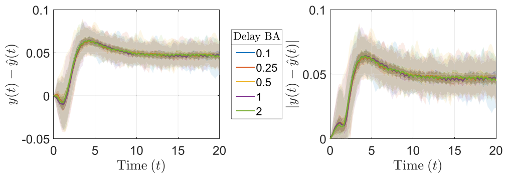
FIG. 18. Error (left) and absolute error (right) of our prevalence approximation (15) with respect to NIMFA on discrete-time RWIG without self-loops. The delay between the start of the RWIG and NIMFA process is varied. Additionally, the walkers have BA-policies.
