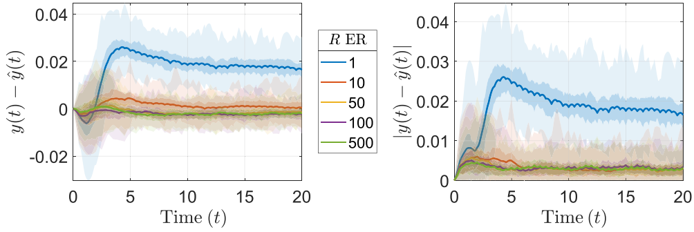
FIG. 10. Error (left) and absolute error (right) of our prevalence approximation (15) with respect to NIMFA on discrete-time RWIG without self-loops. The number of different walker policies R is varied.
