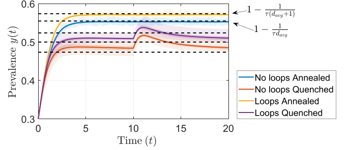
FIG. 5. Comparison of the steady states of NIMFA with and without self-loops in the annealed and quenched regime. The light-shaded area shows 100% of simulations, while the dark-shaded area shows the 50% of simulations closest to the mean (thick line). The three steady-state values from Fig. 4, as well as those with the average degree substituted, are shown in dashed black. The baseline parameters as described in Appendix B 1 are used with the exception of BA walker policies, K = 200 and \Delta t = 0.1 for annealed and \Delta t = 5 for quenched.
