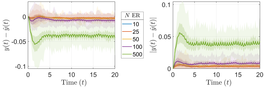
FIG. 12. Error (left) and absolute error (right) of our prevalence approximation (15) with respect to NIMFA on discrete-time RWIG without self-loops. The policy size N is varied.
