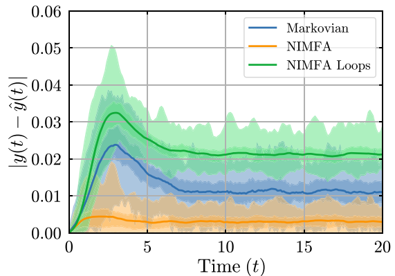
FIG. 22. Left: prevalence of Markovian SIS (blue) and NIMFA with (green) and without (orange) self-loops on continuous-time RWIG, compared with the prevalence approximation (15) and with the corrected approximation (see Sec. VIC) in black and red respectively. Right: Absolute error of our prevalence approximation (15) compared to the prevalence of Markovian SIS and NIMFA with and without self-loops on continuous-time RWIG. The baseline parameters from Table I are used.
