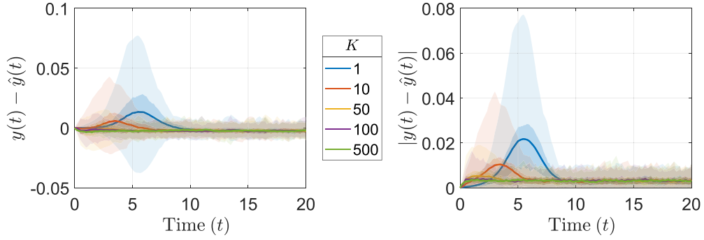
FIG. 8. Error (left) and absolute error (right) of our prevalence approximation (15) with respect to NIMFA on discrete-time RWIG without self-loops. The number of initially infected walkers K is varied.
