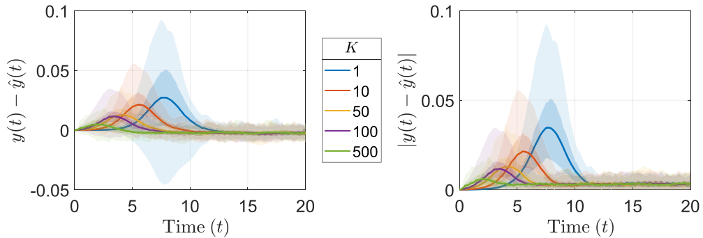
FIG. 9. Error (left) and absolute error (right) of our prevalence approximation (15) with respect to NIMFA on discrete-time RWIG without self-loops. The number of initially infected walkers K is varied. Additionally, the initially infected walkers have v_m(0) = 0.1 instead of v_m(0) = 1 .
