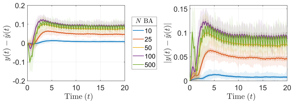
FIG. 15. Error (left) and absolute error (right) of our prevalence approximation (15) with respect to NIMFA on discrete-time RWIG without self-loops. The policy size N is varied. Additionally, the walkers have BA-policies with the same node ordering.
