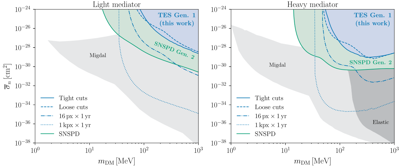
FIG. 7. DM-nucleon scattering. New limits and projections at the 95% CL for DM-nucleon scattering. The shaded dark and light gray regions indicate the strongest existing terrestrial constraints to date [73–83] based on elastic interactions and the Migdal effect, respectively. All other features are identical to those of Fig. 5. Constraints may be relaxed for \bar{\sigma}_n \gtrsim 10^{-25} cm 2 due to atmospheric scattering (see text).
