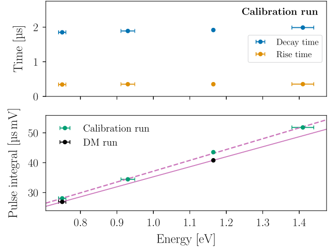
FIG. 2. Calibration measurements. Top: mean fitted rise time \tau_+ and decay time \tau_- as defined by Eq. (1). The time uncertainties are not visible at this scale. The uncertainties of the energy represent the spectral width of the laser diodes, as measured with a spectrometer. The rise and decay time of the calibration photons are mostly constant over this energy range. Bottom: mean pulse integral from the fitting function for different energies for our calibration run (green) and DM run (black). The uncertainties on the pulse integral are not visible at this scale. The relationship between the pulse integral and energy of the calibration photons follows an affine relation as indicated by the dashed purple line. In our analysis, we assume that a similar relation also holds for the DM run, indicated by the solid purple line. Environmental changes between different cooldowns can cause differences in the calibration relations.
