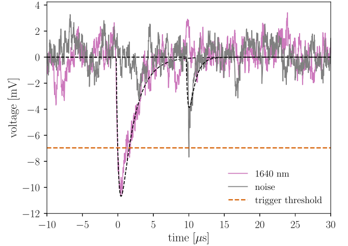
FIG. 3. Example pulses. Example pulses measured with the TES system. The purple curve shows time series measurements for a 1640 nm calibration pulse (DM run), while the gray curve represents a pulse yielding a trigger from noise recorded as part of the DM search measurement and removed before the cut analysis. The dashed black line represents the FFT fits and the red dashed line shows the applied trigger level. A mismatch between the pulse height of the fit and the minimum of the time series itself is clearly visible for the noise spike. But for a single sample surpassing the threshold, our pipeline would not have triggered on this pulse.
