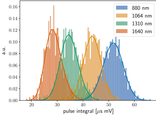
FIG. 8. Scaled pulse integral distributions of TES pulses measured with different calibration wavelengths. The distributions are fitted to skewed Gaussian functions described by Eq. (A1).
