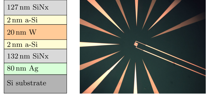
FIG. 1. Prototype TES detector. Left: schematic showing different layers of the optical TES stack with the active tungsten (W) layer placed in between dielectric amorphous Si layers and on a reflective Ag mirror and Si substrate. This layering optimizes the absorption at 1064 nm. Right: close-up of the TES sensor on the silicon substrate, provided by NIST; the fins around the square chip are for aligning purposes only (taken from Ref. [44]).
