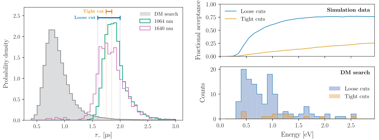
FIG. 4. DM science run. Left: distribution of FFT fitting parameter \tau_- of the direct DM search measurement (gray) and the two measured calibration wavelengths (green and magenta) for reference. While the lasers' distributions overlap with each other to a large extent, much of the DM search measurement distribution lies outside of that region due to small decay times of fast noise spikes. Rigorous cuts can be applied based on this distinction, which also holds for photonlike signals of a broader energy range. Right top: total acceptance \mathcal{A} in simulation data for the loose and tight cuts (see Table I). Right bottom: energy spectrum measured over 489 h and calibrated with the FFT pulse integral parameter based on the loose and tight cuts. The bin size approximates the energy resolution of \sim 0.1 eV at \sim 0.76 eV.
