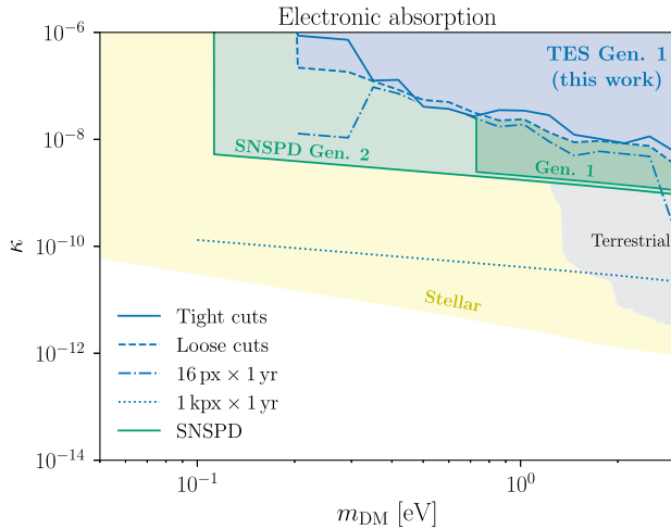
FIG. 6. Dark photon DM absorption. New TES limit and projections at the 95% CL on dark photon DM absorption on electrons. Model-dependent stellar constraints [65,69,70] are shown in shaded yellow. All other features are identical to those of Fig. 5. Constraints may be relaxed due to atmospheric overburden (see text).
