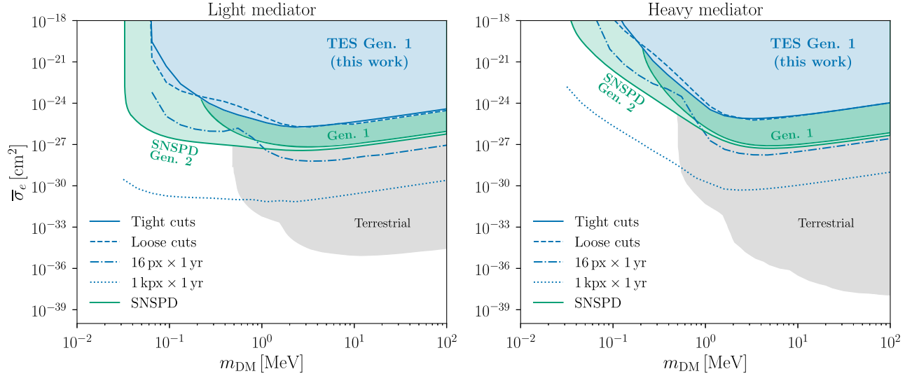
FIG. 5. DM-electron scattering. New bound and projections at the 95% CL on DM scattering with electrons via a light (left) or heavy (right) mediator in a TES sensor. In both panels, the shaded blue region indicates the new constraint we place with the existing TES data from DESY using the tight (solid curve) or loose (dashed curve) cuts. The projected reach of a future experiment using a 16-pixel array exposed for a year (3.2 ng · yr) and using the loose cuts, with each unit similar to our current TES and with background scaling with exposure, is shown by the dot-dashed curve. The projection for a 1000-pixel array exposed for a year (0.2 \mu\text{g} \cdot \text{yr} ), assuming a lower energy threshold of 70 meV and no backgrounds, is shown with the dotted blue line. For comparison, we show existing constraints from SNSPD sensors [12,14,27], indicating the improvement achieved from first- to second-generation devices. Other existing terrestrial constraints are shown in shaded gray [59–64]. Constraints may be relaxed for \bar{\sigma}_e \gtrsim 10^{-24} \text{ cm}^2 due to atmospheric scattering (see text).
