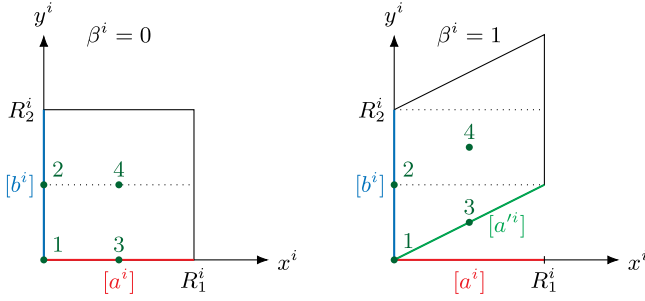
FIG. 1. The \mathbb{Z}_2 invariant a -type (left) and b -type (right) lattices. \mathbb{Z}_2 fixed points \{1, 2, 3, 4\} are shown as blobs. The \mathcal{R} invariant x^i axis is along the 1-cycle [a^i] - \frac{\beta^i}{2}[b^i] with \beta^i = 0 for the a -type lattice and \beta^i = 1 for the b -type lattice. \mathcal{R} acts as reflection along the y^i axis, which is spanned by the 1-cycle [b^i] . For the a -type lattice, all \mathbb{Z}_2 fixed points are invariant under \mathcal{R} , whereas for the b -type lattice, only 1 and 2 are invariant while 3 \xleftrightarrow{\mathcal{R}} 4 .
