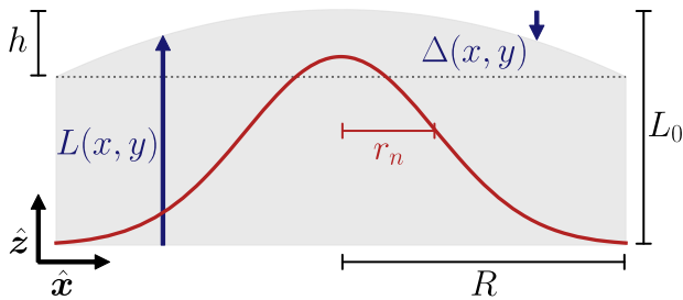
FIG. 1. Cross-section schematic of a plano-convex bulk acoustic resonator. The device dimensions, h, R, L_0 are outlined in black, and the x, y -dependent distances [ L(x, y) and \Delta(x, y) ] are highlighted in blue. An example Gaussian phonon mode profile is shown in red, with a radius r_n given in Eq. (4).
