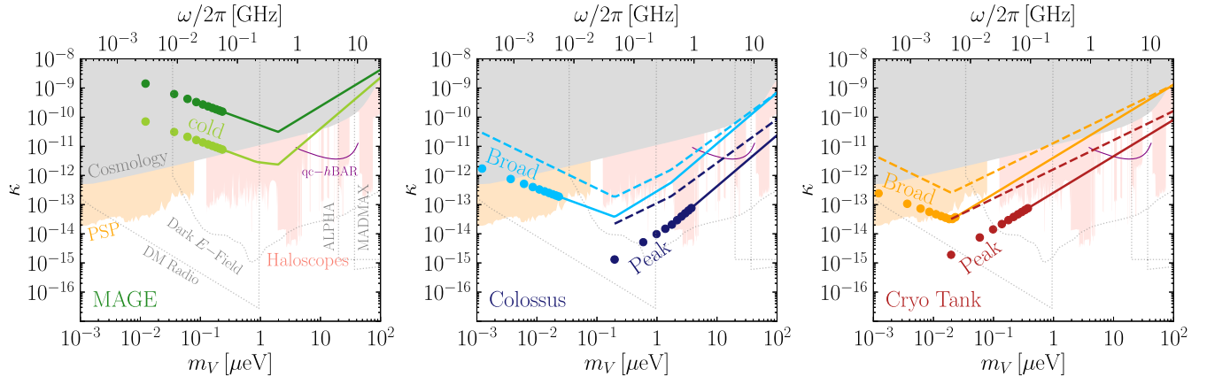
FIG. 2. Projected sensitivity of a single piezoelectric BAR to the kinetic mixing parameter, \kappa [Eq. (1)], for the designs in Table II, averaging over the DM polarizations ( \cos \theta_V \rightarrow 1/\sqrt{3} ). The sensitivity of the first ten resonances is indicated by dots; for higher modes the sensitivity lies along the extending line. Dots and solid lines assume T_{\text{obs}} = 1 month. Dashed lines show the scanning sensitivity, assuming T_{\text{obs}} = 1 yr, and simultaneous readout of all phonon modes, for each e -fold in m_V . The minimum detectable mass for each design is m_V^{\text{min}} = \pi c_1 / L_0 . The prominent turnover at m_V \sim 1/R_s is due to shielding effects [Eq. (5)]. Gray shaded regions are excluded cosmologically [19], orange shaded regions are excluded by recent Parker Solar Probe (PSP) bounds [49], and red shaded regions are excluded by current haloscope experiments [48]. The purple line is the projected “Gen. II” sensitivity of a qubit-coupled high-overtone BAR (qc-hBAR) using single phonon readout [11]. Dotted gray lines are projections for the ALPHA [50], DM-Radio [36], Dark E -field [51], and MADMAX [50,52] experiments.
