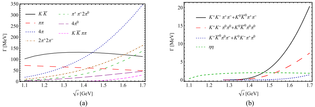
FIG. 3. Dependence of the partial widths of different channels on the center-of-mass energy \sqrt{s} with fixed coupling g_{F\kappa\bar{\kappa}} = 35 GeV and cutoff parameter \alpha(\alpha_B) = 2(1) . Because the scales in widths for some channels are much smaller than others, we present them in two separate figures with distinct scale for clarity. (a) K\bar{K} , \pi\pi , 4\pi , and K\bar{K}\pi\pi channels. Different specific 4\pi states are also presented. (b) K\bar{K}\pi\pi and \eta\eta channels. Different specific K\bar{K}\pi\pi states are also presented. Note that \Gamma(K^+K^-\pi^+\pi^-) = \Gamma(K^0\bar{K}^0\pi^+\pi^-) , \Gamma(K^+\bar{K}^0\pi^0\pi^-) = \Gamma(K^0K^-\pi^+\pi^0) and \Gamma(K^+K^-\pi^0\pi^0) = \Gamma(K^0\bar{K}^0\pi^0\pi^0) . For the \eta\eta channel, \Gamma(F \rightarrow \eta\eta) is presented.
