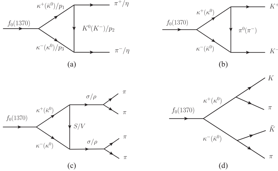
FIG. 1. Mechanism for f_0(1370) decay as a \kappa\bar{\kappa} molecular state. (a) \pi^+\pi^-/\eta\eta final states. (b) K^+K^- final states. (c) 4\pi final states. S/V denotes that the t -channel exchange meson is either a scalar \kappa or a vector K^* . (d) K\bar{K}\pi\pi final states.
