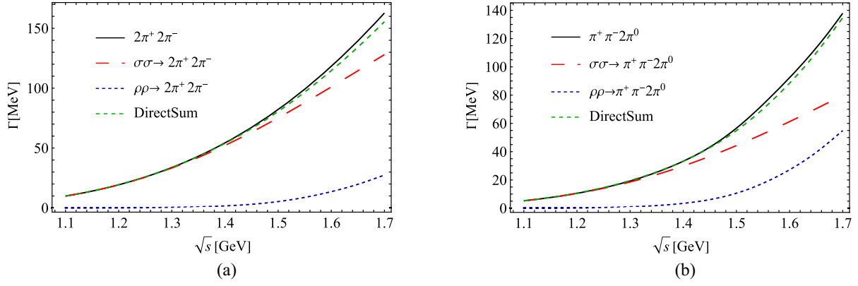
FIG. 4. Dependence of the partial widths of 4\pi states on the center-of-mass energy \sqrt{s} . Contributions from different intermediate channels \sigma\sigma and \rho\rho are also plotted. (a) For the 2\pi^+2\pi^- states. (b) For the \pi^+\pi^-2\pi^0 states.
