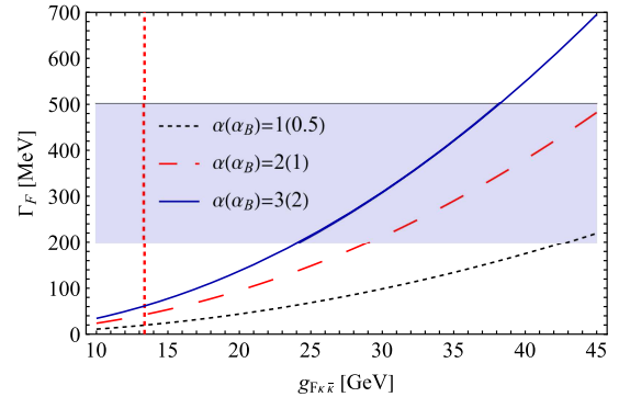
FIG. 2. Total width of f_0(1370) dependent on the parameter g_{F\kappa\bar{\kappa}} with \sqrt{s} = 1.37 GeV and three form factor parameter sets \alpha(\alpha_B) = 1(0.5)/2(1)/3(2) . The red dashed vertical line indicates the reference value g_{F\kappa\bar{\kappa}} = 13.4 GeV which is estimated from the Weinberg compositeness criterion [64,65] using a complex \kappa mass \sqrt{s}_\kappa = 0.7 - 0.3i GeV with X = 1 ; the light purple band indicates the range of the Breit-Wigner width of f_0(1370) measured in experiments.
