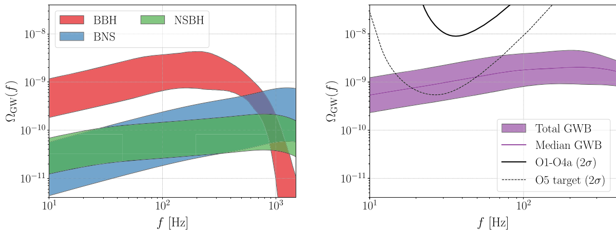
FIG. 7. Left: Projected astrophysical GWB contributions from BBH, BNS, and NSBH coalescences. Shaded bands represent the 90% credible bounds for each CBC class. Right: Solid purple line showing the median estimate of \Omega_{\text{BBH+BNS+NSBH}}(f) as a function of frequency, while the shaded purple band illustrates 90% credible uncertainties. We also show the 2\sigma PI sensitivity curve calculated using data from stochastic isotropic searches O1 through O4a, considering the three HLV baselines. We include the target 2\sigma PI curve for O5, assuming the target sensitivity curves for the HLV baselines as detailed in Refs. [88,192].
