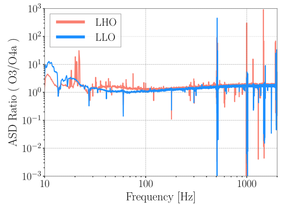
FIG. 3. Ratio of the detector strain sensitivity curves between O3 and O4a for LHO (red) and LLO (blue). A ratio above unity indicates an improvement in sensitivity compared to O3.
