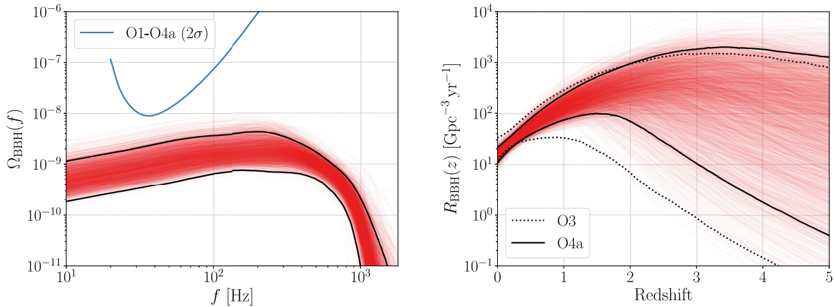
FIG. 6. Left: Forecast for the stochastic energy-density spectrum of the BBH population, given the population of direct BBH detections within the LVK GWTC-4 catalog [86] and the GWB upper limit presented here. The black curves indicate 90% credible bounds on \Omega_{\text{BBH}}(f) , while red traces show individual posterior samples on the energy-density spectrum, obtained by sampling over the possible mass, spin, and redshift distributions of BBH mergers. For comparison, the blue curve indicates the 2\sigma PI curve calculated using O1–O4a Hanford-Livingston-Virgo (HLV) data [151], integrated over all observing runs to date. Right: Inferred redshift evolution of the BBH merger rate density, measured hierarchically using the direct BBH detections in GWTC-4 and the GWB upper limit. Solid black and red lines again mark 90% credible bounds and individual posterior samples, respectively, while dotted black lines denote the 90% credible bounds obtained previously with GWTC-3 [169].
