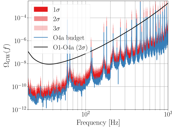
FIG. 1. Computed magnetic budget (blue), including \hat{\Omega}_{\text{mag}} + 1\sigma , \hat{\Omega}_{\text{mag}} + 2\sigma , and \hat{\Omega}_{\text{mag}} + 3\sigma uncertainties (in progressively lighter shades of red). The magnetic budget remains consistently below the 2\sigma power-law integrated sensitivity curve (black), except for narrowband features numerically induced by the ORF and harmonics of the 60 Hz power lines.
