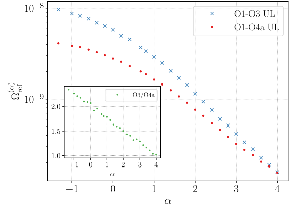
FIG. 5. Upper limits on \Omega_{\text{ref}}^{(\alpha)} at 95% CL as a function of \alpha , obtained assuming the GWB is described by a power-law model using a log-uniform prior on the amplitude \Omega_{\text{ref}}^{(\alpha)} . The blue curve shows the results using data from O1 to O3, while the red curve includes O4a data as well. The inset plot shows the ratio between the two sets of limits, highlighting improvement in O4a as a function of spectral weighting.
