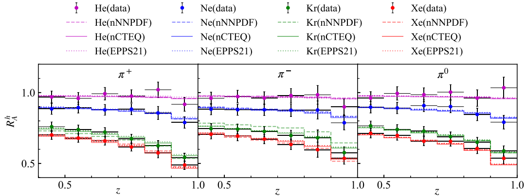
FIG. 13. Benchmark comparison of measured and predicted nuclear modifications for pion production in HERMES experiments [35] using different nPDF inputs while keeping the extracted nFFs fixed.
