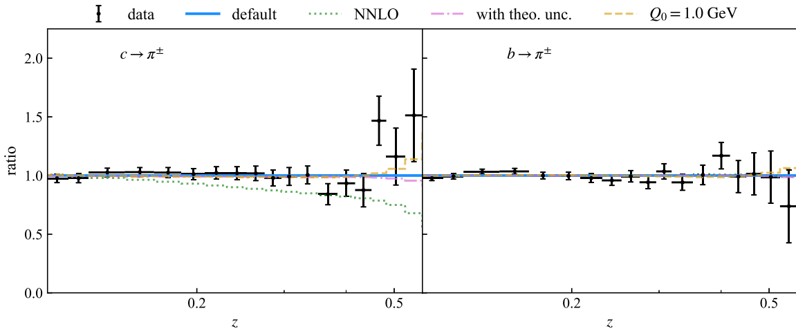
FIG. 3. Similar to Fig. 1, but for \pi^\pm production in SIA at SLD [44], shown as a function of z .
