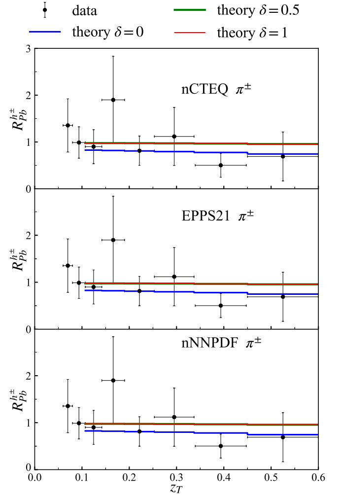
FIG. 12. p\text{Pb} -to- pp nuclear modification ratio for \gamma^{\text{iso}} -tagged fragmentation functions at \sqrt{s_{\text{NN}}} = 5.02 TeV, compared with the ALICE measurements. The three panels show predictions obtained with nFFs extracted using the nCTEQ15WZ, EPPS21, and nNNPDF nPDF inputs, respectively.
