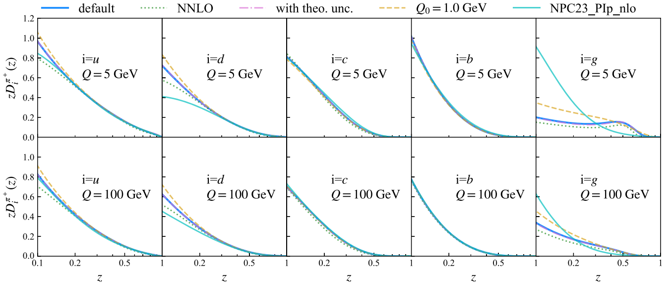
FIG. 4. Comparison of the extracted vacuum FFs for \pi^+ with the NPC23 [80] for different parton flavors at Q = 5 GeV and Q = 100 GeV.
