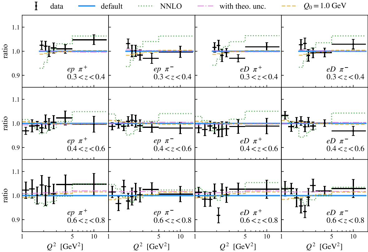
FIG. 1. Comparison of HERMES measurements [42] and theoretical predictions for \pi^+ and \pi^- production in SIDIS off p and D targets, shown in bins of z as functions of Q^2 . All results are presented as ratios to the default prediction, defined as the setup with Q_0 = 1.3 GeV, NLO, and the exclusion of theoretical uncertainties. The black points with error bars represent the experimental data divided by the default prediction. The solid blue line corresponds to the default prediction and is therefore equal to unity by construction. The dotted green line shows the NNLO prediction, the dash-dotted pink line shows the result obtained when theoretical uncertainties are included in the fit, and the dashed orange line corresponds to the initial scale choice Q_0 = 1.0 GeV.
