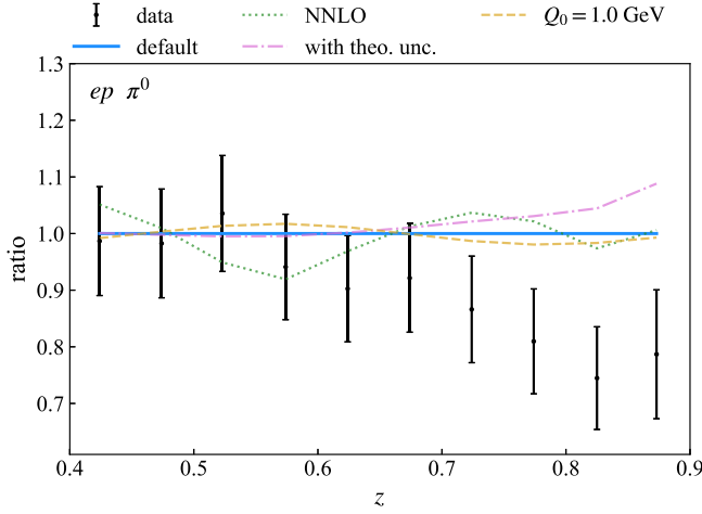
FIG. 2. Similar to Fig. 1, but for \pi^0 production in HERMES experiments [43], shown as a function of z .
