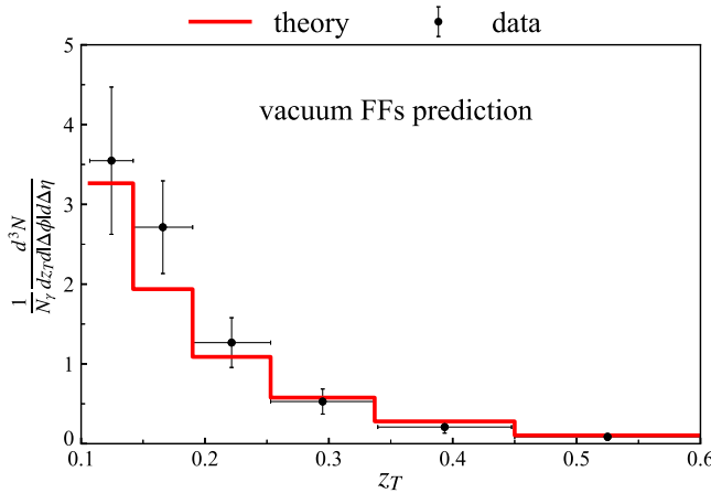
FIG. 11. Comparison of the \pi^\pm NLO prediction obtained with the default vacuum FFs and ALICE measurements for \gamma^{\text{iso}} -tagged fragmentation functions of a charged hadron in pp collisions at \sqrt{s} = 5.02 TeV.
