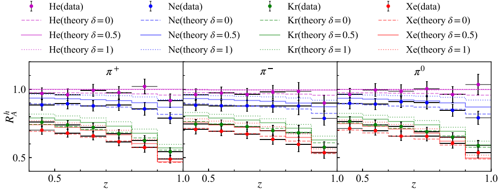
FIG. 7. Comparison of the measured and predicted nuclear modification with respect to z for \pi production in HERMES experiments [35]. Theoretical predictions are obtained for different \nu dependences and curves.
