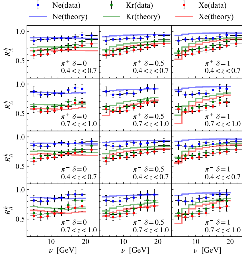
FIG. 5. Comparison of the measured and predicted nuclear modification with respect to z and \nu for \pi^+ and \pi^- in HERMES experiments [36].
