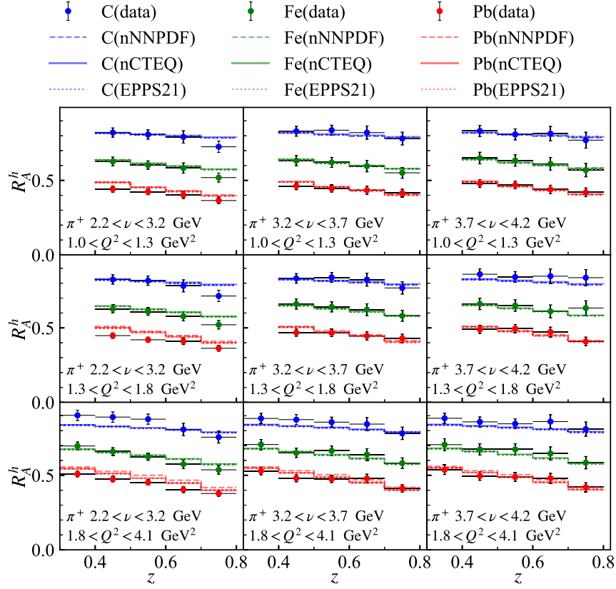
FIG. 14. Similar to Fig. 13, but for the CLAS measurements [37] shown as functions of z and \nu .
