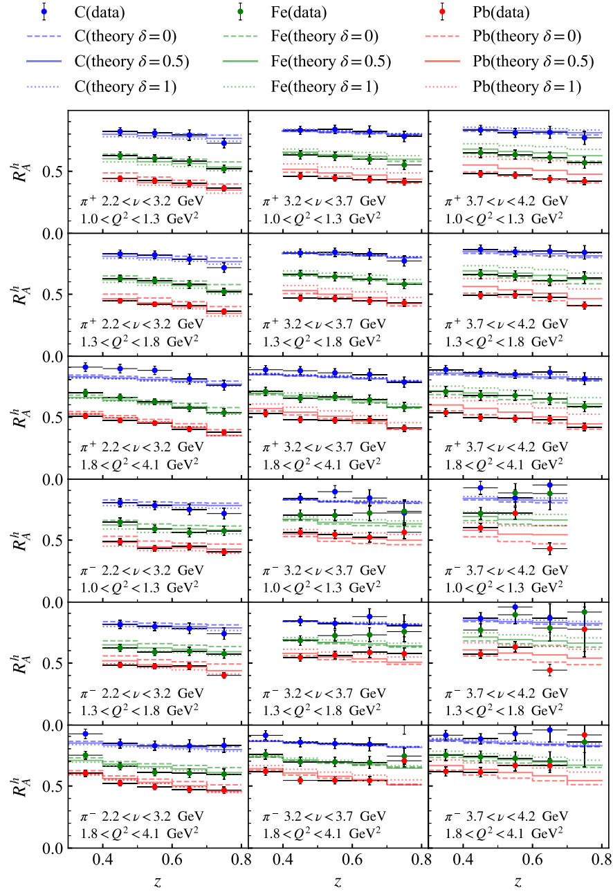
FIG. 8. Comparison of the measured and predicted nuclear modification with respect to z and \nu for \pi^+ and \pi^- in CLAS experiments [37]. Theoretical predictions are shown for different assumptions on the \nu dependence. The C, Fe, and Pb targets are shown in blue, green, and red, respectively. The \delta = 0.5 , \delta = 0 , and \delta = 1 schemes are represented by solid, dashed, and dotted lines, respectively.
