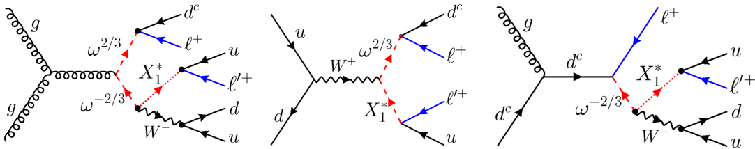
FIG. 4. Representative Feynman diagrams illustrating the QCD pair production of leptoquarks (left), electroweak pair production (center), and single leptoquark production (right), leading to LNV signatures pp \rightarrow \ell^\pm \ell'^\pm + \text{jets} at the LHC.
