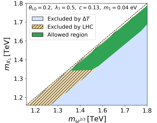
FIG. 3. Parameter space is shown in the m_{\omega^{2/3}} - m_{\tilde{X}_1} plane. The blue shaded region is excluded by constraints from \Delta T at 95% CL, while the yellow shaded region is ruled out by leptoquark pair production searches at the \sqrt{s} = 13 TeV LHC [66,67]. The green shaded region denotes the parameter space consistent with current constraints. Results are shown for the benchmark scenario \{\theta_{\text{LQ}} = 0.2, \lambda_7 = 0.5, c \equiv \lambda_{ij}/\lambda'_{ij} = 0.13, m_1 = 0.04 \text{ eV}\} .
