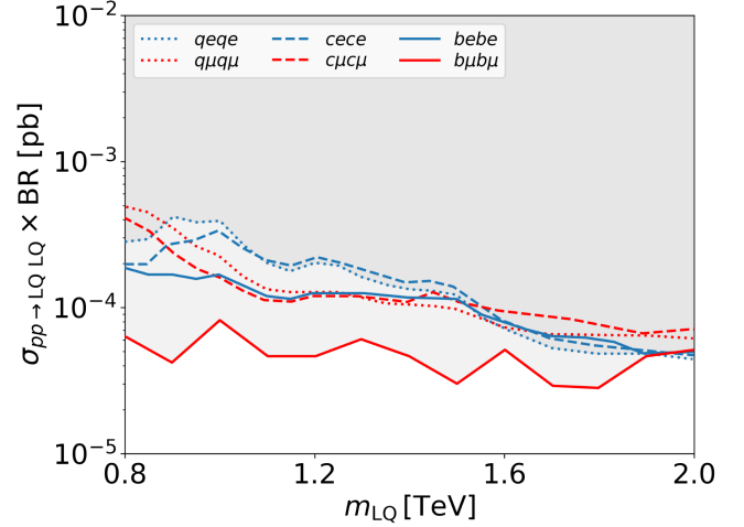
FIG. 2. Upper limits on the leptoquark pair production cross section times branching fraction, pp \rightarrow \text{LQ}\bar{\text{LQ}} \rightarrow X , as a function of leptoquark mass m_{\text{LQ}} , from searches in the X = \{qe qe, q\mu q\mu, ce ce, c\mu c\mu, be be, b\mu b\mu\} channels by ATLAS [66] and CMS [67] at the \sqrt{s} = 13 TeV LHC.
