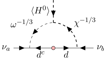
FIG. 1. Feynman diagram representing neutrino mass generation at one-loop in the Leptoquark variant of the Zee model.
