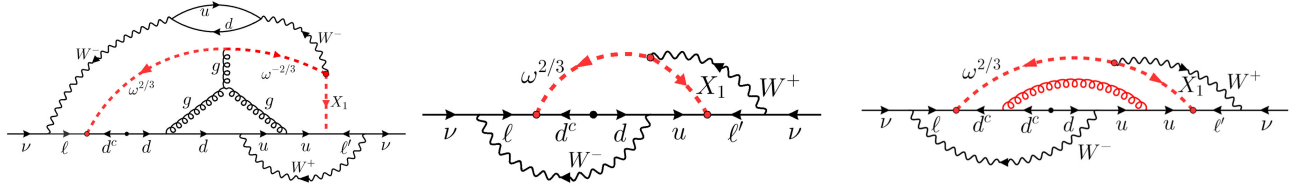
FIG. 5. Diagrams illustrating the connection between Majorana neutrino mass generation and LNV signatures at the LHC [9,10]. The left, center, and right diagrams for neutrino mass generation correspond, respectively, to the LHC processes shown in the left, center, and right panels of Fig. 4.
