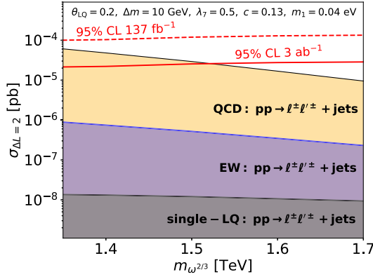
FIG. 6. Stacked cross section for the LNV process, pp \rightarrow \ell^\pm \ell'^\pm + \text{jets} , mediated by QCD pp \rightarrow \text{LQ LQ} (yellow), EW pp \rightarrow \text{LQ LQ} (blue), and single leptoquark production pp \rightarrow \text{LQ} \ell (gray) at \sqrt{s} = 13 TeV, assuming leptoquark mixing angle \theta_{\text{LQ}} = 0.2 , \Delta m \equiv m_{\omega^{2/3}} - m_{X_1} = 10 GeV, \lambda_7 = 0.5 , c \equiv \lambda_{ij}/\lambda'_{ij} = 0.13 , and m_1 = 0.04 eV. The 95% confidence level limits are shown for an integrated luminosity of 137 \text{ fb}^{-1} (red dashed) and for the HL-LHC projection with 3 \text{ ab}^{-1} (red solid).
