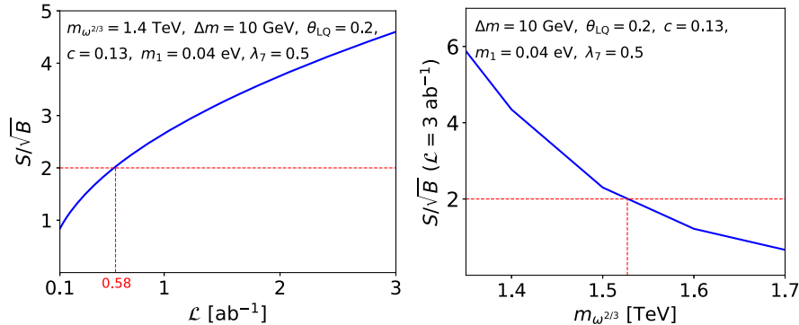
FIG. 7. Signal significance S/\sqrt{B} for the LNV process pp \rightarrow \ell^\pm \ell'^\pm + \text{jets} at the LHC with \sqrt{s} = 13 TeV. Left: Significance as a function of integrated luminosity. Right: Significance at the HL-LHC with \mathcal{L} = 3 \text{ ab}^{-1} as a function of the leptoquark mass m_{\omega^{2/3}} , assuming \theta_{\text{LQ}} = 0.2 , \Delta m = 10 GeV, \lambda_7 = 0.5 , c \equiv \lambda_{ij}/\lambda'_{ij} = 0.13 , and m_1 = 0.04 eV.
