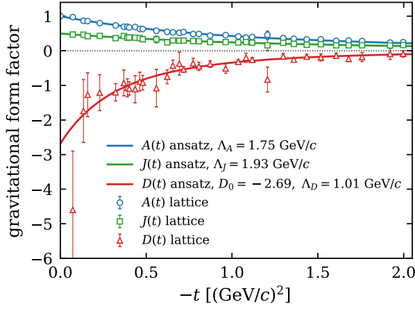
FIG. 1. Momentum transfer dependence of the GFFs based on the ansatz in Eq. (2), fitted to the lattice QCD results [36].
