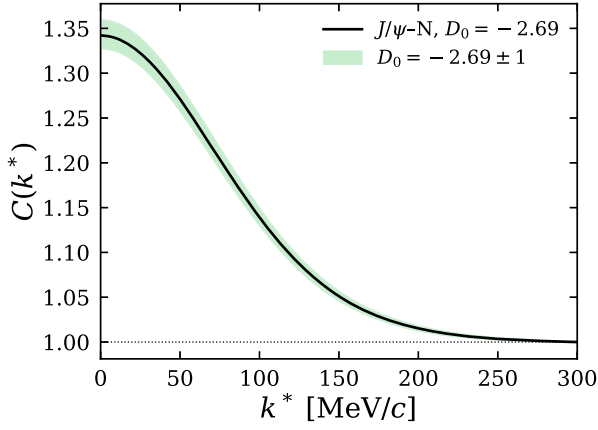
FIG. 6. The J/\psi - N correlation function. The shaded band represents the variation of the correlation function when the D -term parameter is varied within D_0 = -2.69 \pm 1 .
