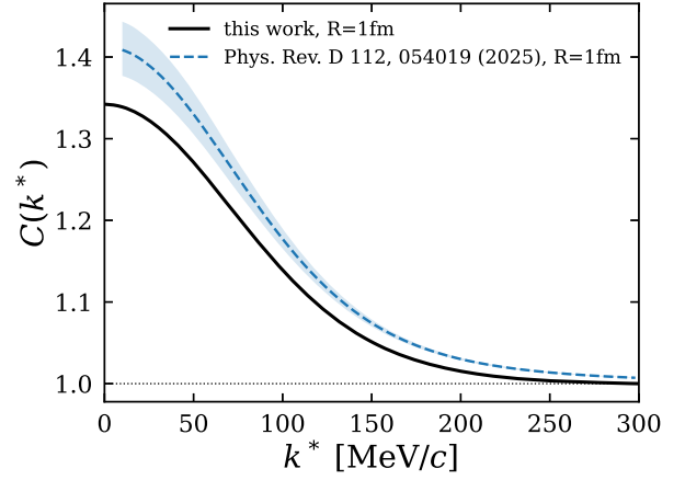
FIG. 5. The J/\psi - N correlation function as a function of k^* . The black solid line is obtained using the smeared J/\psi - N potential, and the result is compared with the model-independent analysis based on the HAL QCD potential [97].
