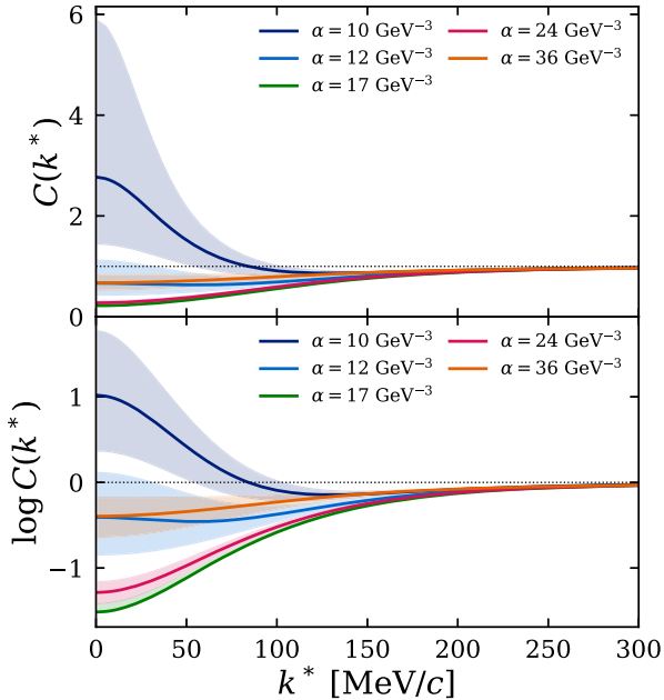
FIG. 7. The \psi(2S) - N correlation function for \alpha_{2S} . The top and bottom panels show C(k^*) and \log C(k^*) , respectively. The shaded bands represent the variation of the correlation function when the D -term parameter is varied within D_0 = -2.69 \pm 1 .
