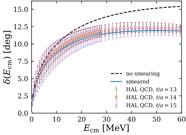
FIG. 4. The J/\psi - N scattering phase shifts as a function of E_{\text{cm}} . The results obtained in this work are compared with those evaluated by solving the Schrödinger equation with the spin-averaged HAL QCD potential shown in Fig. 3.
