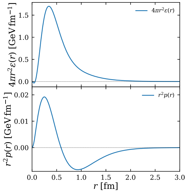
FIG. 2. The radial dependence of the energy distribution (top) and pressure distribution (bottom) inside a nucleon, calculated from the ansatz in Eq. (2).
