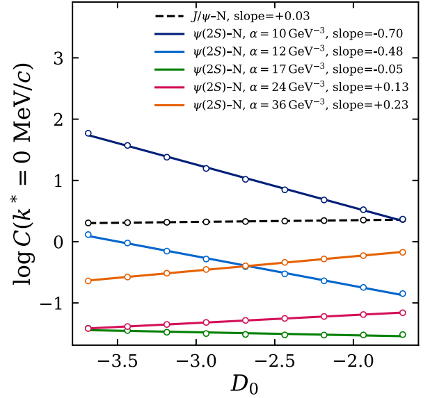
FIG. 8. Response of the charmonium-nucleon correlation function to the value of the D -term in the near-threshold region ( k^* = 0 ). The vertical axis is shown on a logarithmic scale. The data points are fitted with straight lines, and the slope reflects the sensitivity to the D -term.
