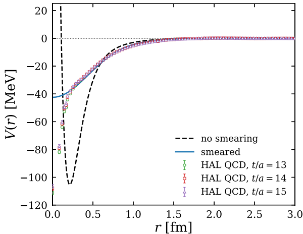
FIG. 3. The J/\psi - N potential. The dashed line shows the potential calculated using Eq. (10), while the blue solid line shows the smeared potential given in Eq. (13). These potentials are compared with the averaged potential evaluated from the HAL QCD data [86]. The values of t/a shown for the HAL QCD data denote the ratio of Euclidean time separation and lattice spacing.
