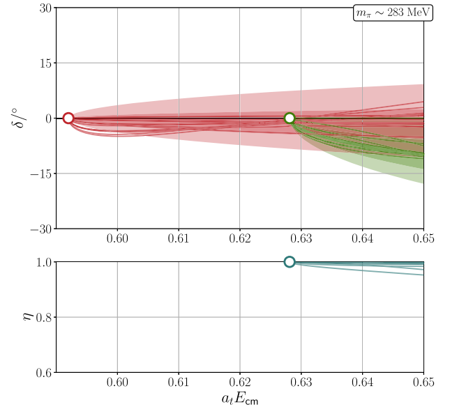
FIG. 3. S -wave coupled-channel phase shifts, \delta_{\eta_c \eta} , \delta_{D\bar{D}} , and inelasticity \eta , as defined in the caption of Fig. 2, for a range of amplitude parametrizations capable of describing the finite-volume spectrum (Tables VI and VII). For the amplitude given in Eq. (3), the uncertainty bands are shown (inner band is the statistical uncertainty, outer band includes also the impact of varying the masses and anisotropy as described in the text). For other amplitude parametrizations, only the central value curves are plotted.
