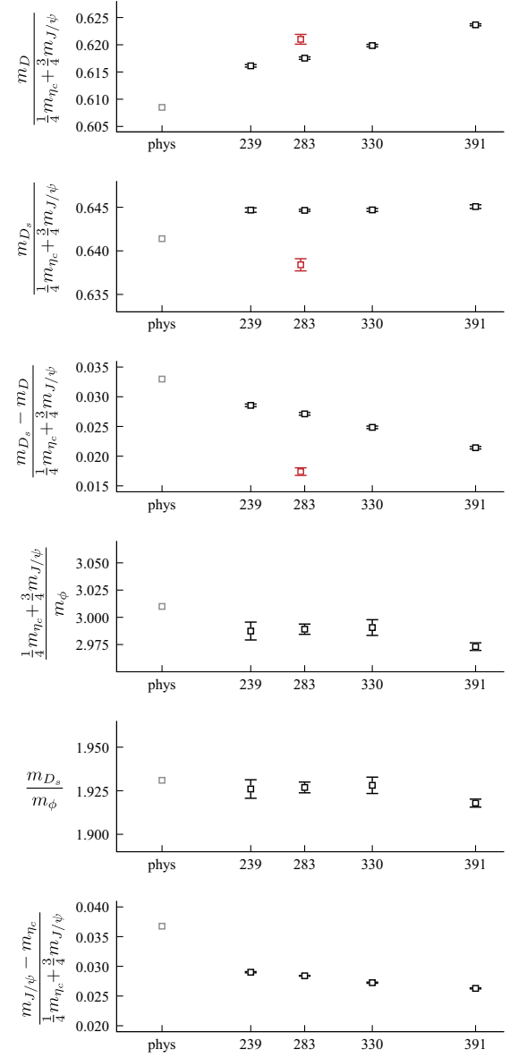
FIG. 8. Ratios of stable hadron masses as a function of m_\pi^2 . Black points determined in the current paper and Refs. [24,25]. Gray points taken from PDG values. Red points from Ref. [27].
