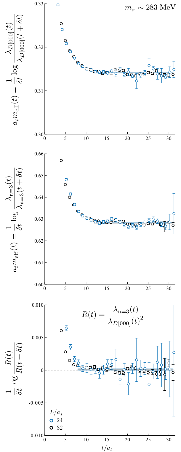
FIG. 9. “Effective masses” for the D -meson at rest (top), the D[000]\bar{D}[000] -dominated level (middle), and a ratio of these (bottom). Each quantity is derived from the principal correlators \lambda_{\mathbf{n}}(t) determined from the variational method analysis of correlation matrices. A representative fit is shown in each case, where the width shows the fit region and the vertical extent shows the value and uncertainty.
