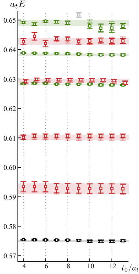
FIG. 7. In same case as Fig. 6, the variation of extracted E_n spectrum with changing choice of t_0 . Solid points show the single best fit-window value, and the ghosted values show the AIC model average. Horizontal bands illustrate the t_0 = 10a_t choice.
