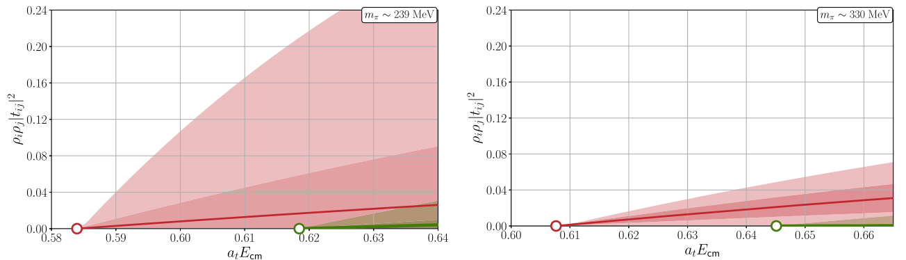
FIG. 4. S -wave scattering amplitudes for m_\pi \sim 239 MeV (left) and 330 MeV (right). Same color coding as in top panels of Fig. 2.
