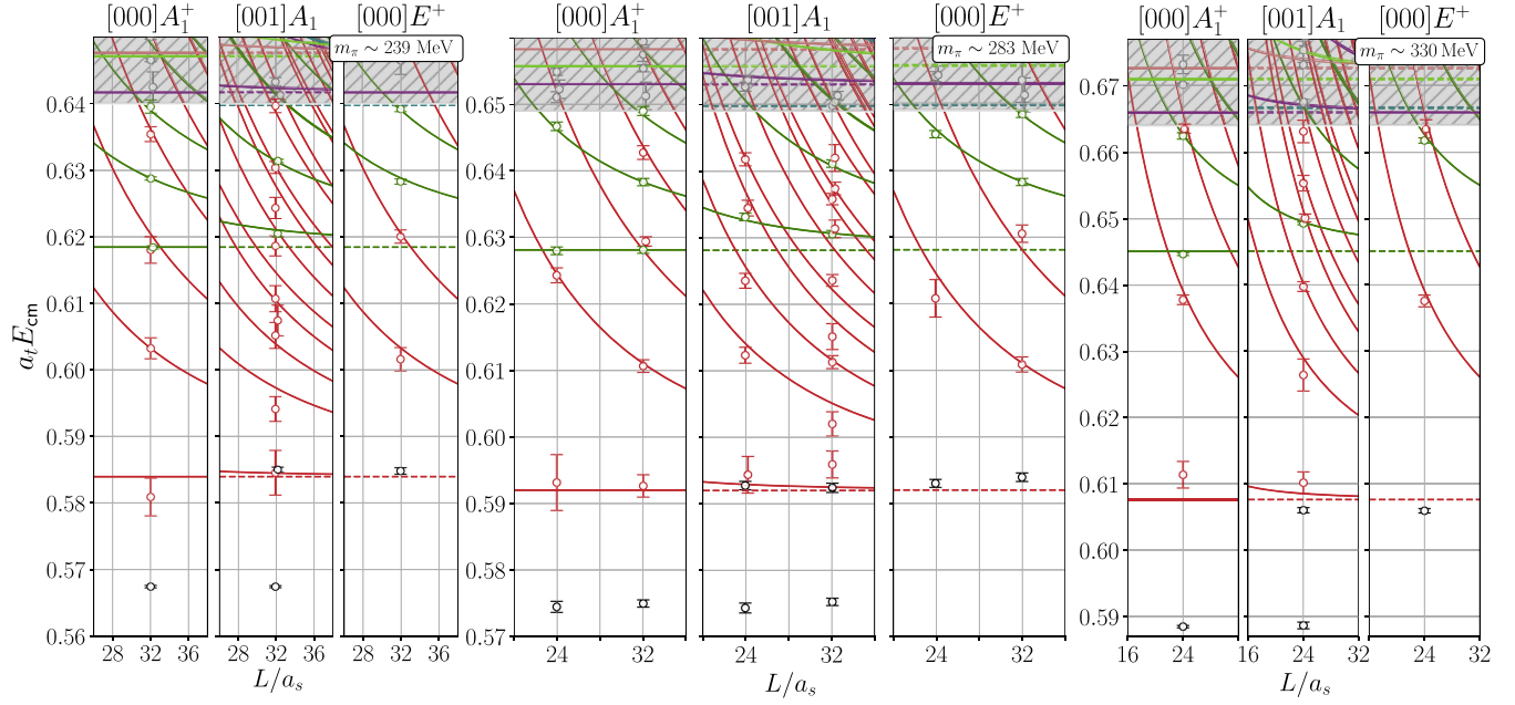
FIG. 1. Finite-volume spectra in three irreps determined on the lattices described in Sec. II. Energy levels are colored according to their dominant operator overlap determined in the diagonalization of the matrix of correlation functions: \eta_c\eta -like (red), D\bar{D} -like (green), c\bar{c} -like (black). Gray points in the hatched high-energy region are not used in the subsequent determination of scattering amplitudes. Curves indicate the noninteracting spectrum of meson pairs on the relevant volumes with the same color coding, with the addition of \psi\omega (purple) and D_s\bar{D}_s (light green) appearing above the energy cutoff. Dashed lines show the relevant meson-meson kinematic thresholds.
