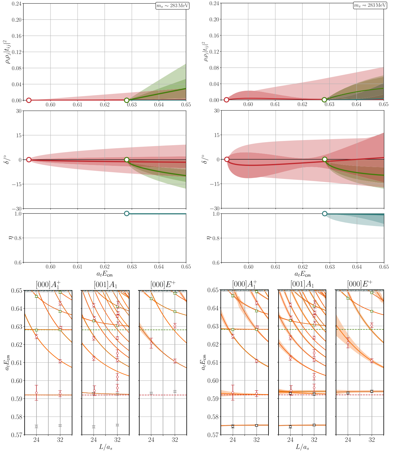
FIG. 2. Coupled \eta_c\eta - D\bar{D} S-wave scattering amplitude descriptions of finite-volume spectra. Left: amplitudes of Eq. (3). Right: amplitudes of Eq. (5). Top panels illustrate the magnitude with a normalization where the unitarity limit is 1 for t_{\eta_c\eta,\eta_c\eta} (red) and t_{D\bar{D},D\bar{D}} (green). Center panels show channel phase shifts, \delta_{\eta_c\eta} (red), \delta_{D\bar{D}} (green) and inelasticity, \eta , defined so that the diagonal elements of the 2 \times 2 t -matrix are t_{ii} = \frac{\eta e^{2i\delta_i} - 1}{2i\rho_i} and the off diagonal element is t_{ij} = \frac{\sqrt{1-\eta^2} e^{i(\delta_i+\delta_j)}}{2\sqrt{\rho_i\rho_j}} . Bottom panels show the finite-volume spectrum given by the amplitude (orange curves) compared with the spectrum constraining the amplitudes.
