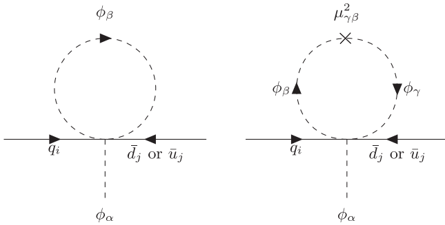
FIG. 3. One-loop radiative corrections to the x_{ij}^\alpha and \tilde{x}_{ij}^\alpha matrices from dimension 6 operators and soft scalar masses in the interaction basis.
