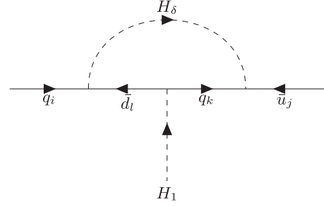
FIG. 2. Feynman diagrams for the one-loop CP -violating contributions to the quark Yukawa couplings x_{ij}^\alpha . Similar diagrams contribute to \tilde{x}_{ij}^\alpha .
