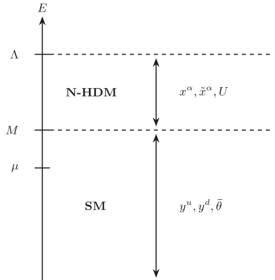
FIG. 1. The framework: energy scales, EFTs, and their flavor parameters. \Lambda is the UV cutoff of theories with N Higgs doublets, all with the same gauge quantum numbers. All but one of these Higgs doublets acquires a mass of order M . Below M , the EFT is the minimal SM.
