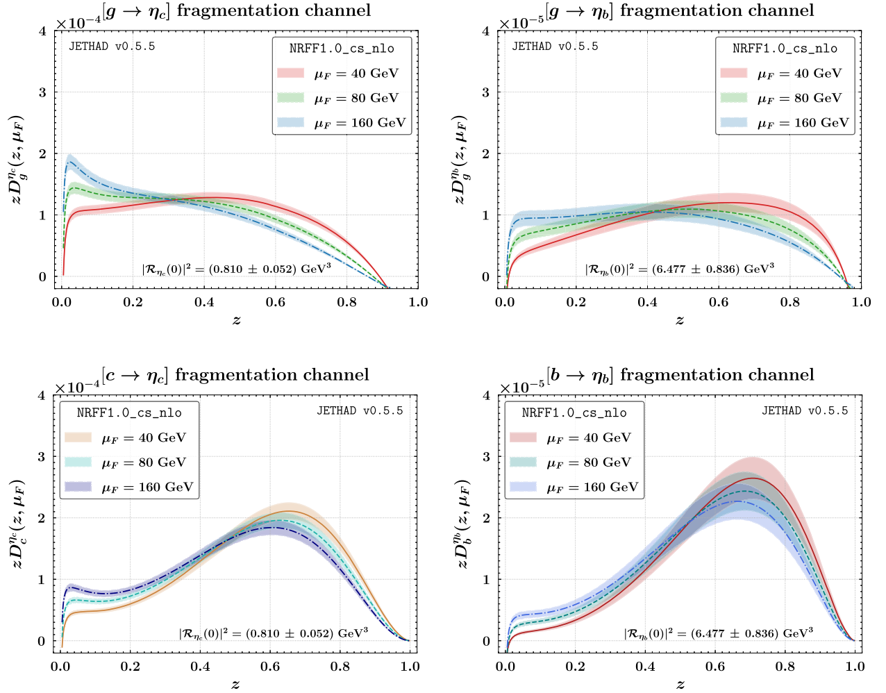
FIG. 8. z dependence of the NRFF1.0 NLO FFs [223] for \eta_c[{}^1S_0^{(1)}] (left) and \eta_b[{}^1S_0^{(1)}] (right) production at \mu_F = 40, 80 , and 160 GeV. The upper (lower) panels show the gluon (constituent heavy quark) fragmentation channel. The shaded bands represent the uncertainty associated with the LDMEs.
