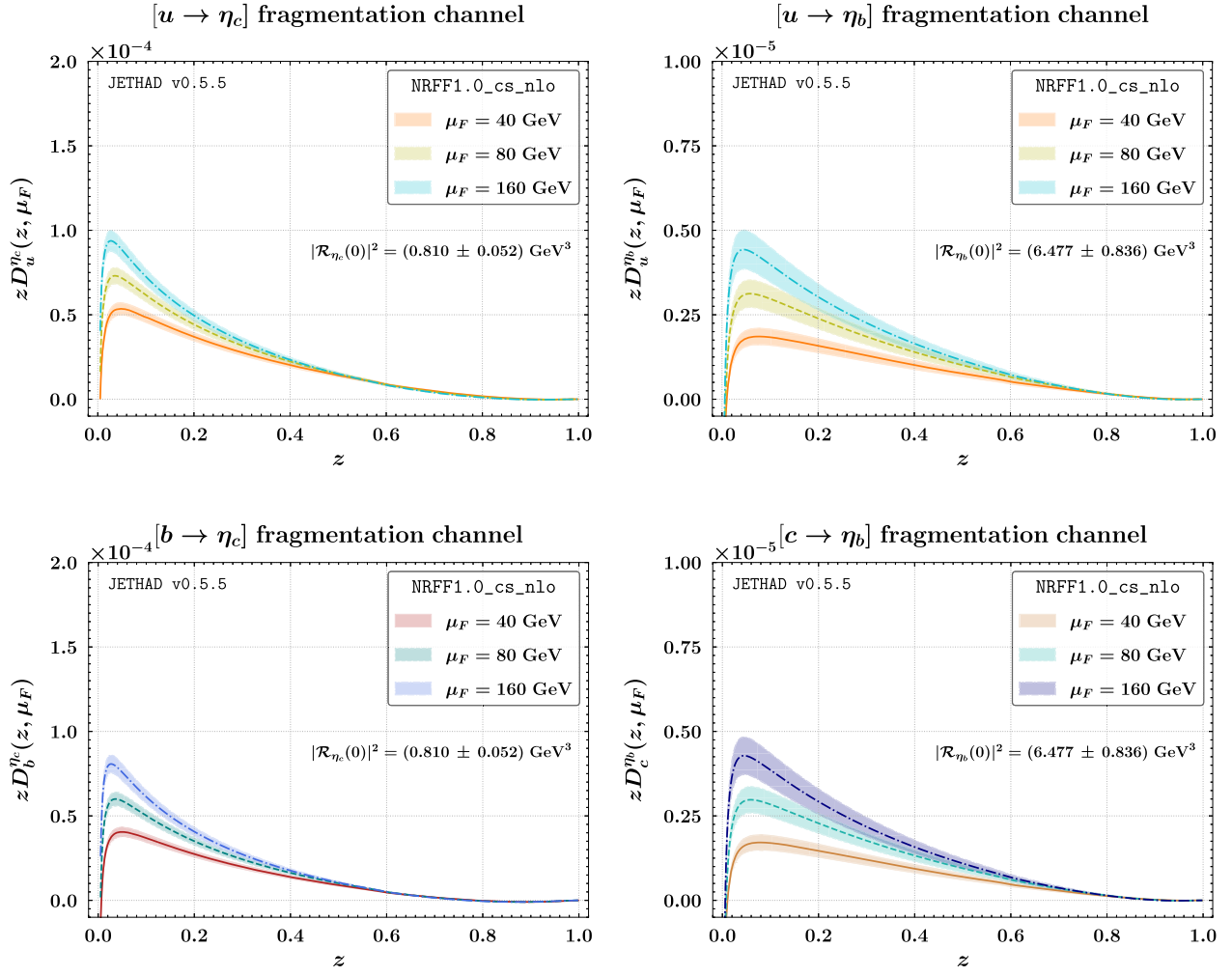
FIG. 9. z dependence of the NRFF1.0 NLO FFs [223] for \eta_c[{}^1S_0^{(1)}] (left) and \eta_b[{}^1S_0^{(1)}] (right) production at \mu_F = 40, 80 , and 160 GeV. The upper (lower) panels show the up-quark (nonconstituent heavy quark) fragmentation channel. The shaded bands represent the uncertainty associated with the LDMEs.
