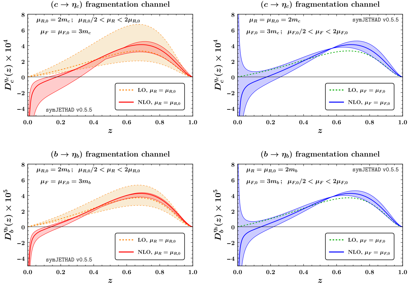
FIG. 4. NRQCD [ c \rightarrow \eta_c , upper] and [ b \rightarrow \eta_b , lower] fragmentation channels at LO and NLO, for \mu_{R,0} = 2m_Q and \mu_{F,0} = 3m_Q . Left plot: \mu_R runs from \mu_{R,0}/2 to 2\mu_{R,0} , while \mu_F is fixed at \mu_{F,0} . Right plot: \mu_R is fixed at \mu_{R,0} , while \mu_F runs from \mu_{F,0}/2 to 2\mu_{F,0} .
