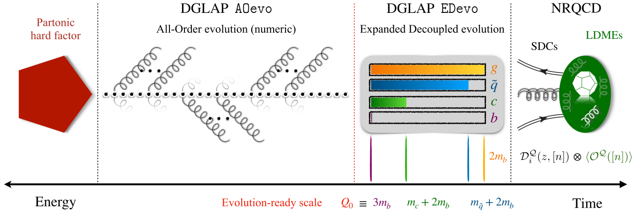
FIG. 7. Evolution workflow for \eta_b[{}^1S_0^{(1)}] FFs within the HF-NRevo scheme. The diagram illustrates the two-stage DGLAP evolution: a semianalytical EDevo phase, starting from the lowest threshold and valid up to the evolution-ready scale Q_0 = 3m_b , where flavor channels are dynamically activated in a stepwise fashion, followed by a numerical AOevo phase.
