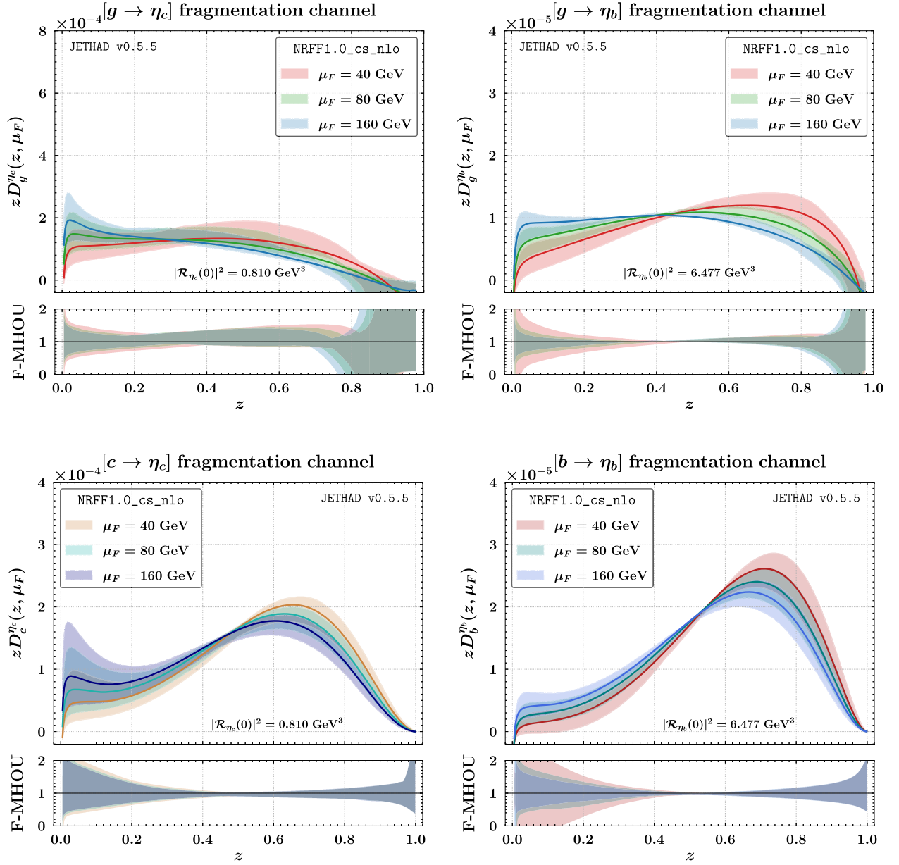
FIG. 10. z dependence of the NRFF1.0 NLO FFs [223] for \eta_c[{}^1S_0^{(1)}] (left) and \eta_b[{}^1S_0^{(1)}] (right) production at \mu_F = 40, 80 , and 160 GeV. The upper (lower) panels show the gluon (constituent heavy quark) fragmentation channel. The shaded bands represent the uncertainty associated with the F-MHOUs, while LDMEs are kept at their central values, as in Eqs. (5) and (6). The ancillary panels below each main plot display the ratio between the FFs evaluated at the central values of the evolution and renormalization scales, and the corresponding FFs obtained by varying each of these scales independently by a factor of 2 around its central value.
