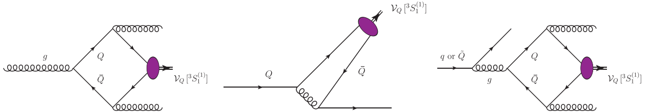
FIG. 2. Left panel: a leading diagram for the fragmentation of a gluon to \mathcal{V}_Q [^3S_1^{(1)}] at \mathcal{O}(\alpha_s^3) . Central panel: one of the leading diagrams for the fragmentation of a constituent heavy quark ( Q ) to a S -wave color-singlet vector quarkonium \mathcal{V}_Q [^3S_1^{(1)}] at \mathcal{O}(\alpha_s^2) . Right panel: a leading diagram for the fragmentation of a nonconstituent light ( \tilde{q} ) or heavy ( \tilde{Q} ) quark to \mathcal{V}_Q [^3S_1^{(1)}] at \mathcal{O}(\alpha_s^4) . Violet blobs refer to the \mathcal{V}_Q [^3S_1^{(1)}] nonperturbative NRQCD LDME.
