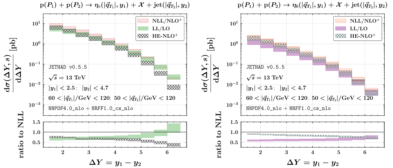
FIG. 16. Rapidity distributions for the semi-inclusive hadroproduction of an \eta_c (left) or \eta_b (right) meson in association with the jet, at \sqrt{s} = 13 TeV. The shaded bands in the main panels represent the combined uncertainty from MHOUs, LDMEs, and multidimensional phase-space integration. The ancillary panels below the main plots display the ratio of the LL/LO and HE-NLO + predictions to the NLL/NLO + result, with bands capturing MHOUs only.
