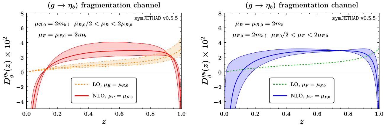
FIG. 3. NRQCD [g \rightarrow \eta_b] fragmentation channel at LO and NLO, for \mu_{R,0} = \mu_{F,0} = 2m_b . Left plot: \mu_R runs from \mu_{R,0}/2 to 2\mu_{R,0} , while \mu_F is fixed at \mu_{F,0} . Right plot: \mu_R is fixed at \mu_{R,0} , while \mu_F runs from \mu_{F,0}/2 to 2\mu_{F,0} .
