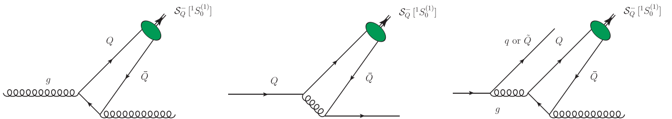
FIG. 1. Left panel: a leading diagram for the fragmentation of a gluon to S_Q^- [1S_0^{(1)}] at \mathcal{O}(\alpha_s^2) . Central panel: one of the leading diagrams for the fragmentation of a constituent heavy quark ( Q ) to a S -wave color-singlet pseudoscalar quarkonium S_Q^- [1S_0^{(1)}] at \mathcal{O}(\alpha_s^2) . Right panel: a leading diagram for the fragmentation of a nonconstituent light ( q ) or heavy ( \bar{Q} ) quark to S_Q^- [1S_0^{(1)}] at \mathcal{O}(\alpha_s^3) . Green blobs refer to the S_Q^- [1S_0^{(1)}] nonperturbative NRQCD LDME.
