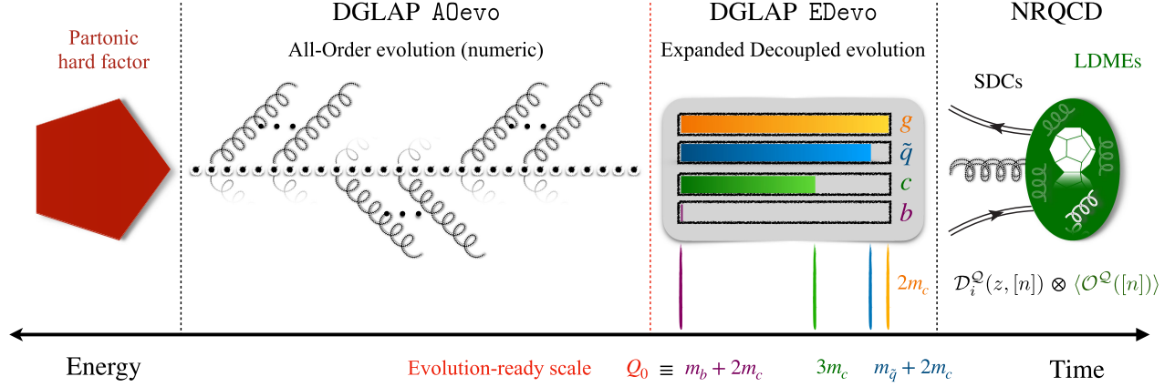
FIG. 6. Evolution workflow for \eta_c[{}^1S_0^{(1)}] FFs within the HF-NRevo scheme. The diagram illustrates the two-stage DGLAP evolution: a semianalytical EDevo phase, starting from the lowest threshold and valid up to the evolution-ready scale Q_0 = m_b + 2m_c , where flavor channels are dynamically activated in a stepwise fashion, followed by a numerical AOevo phase.
