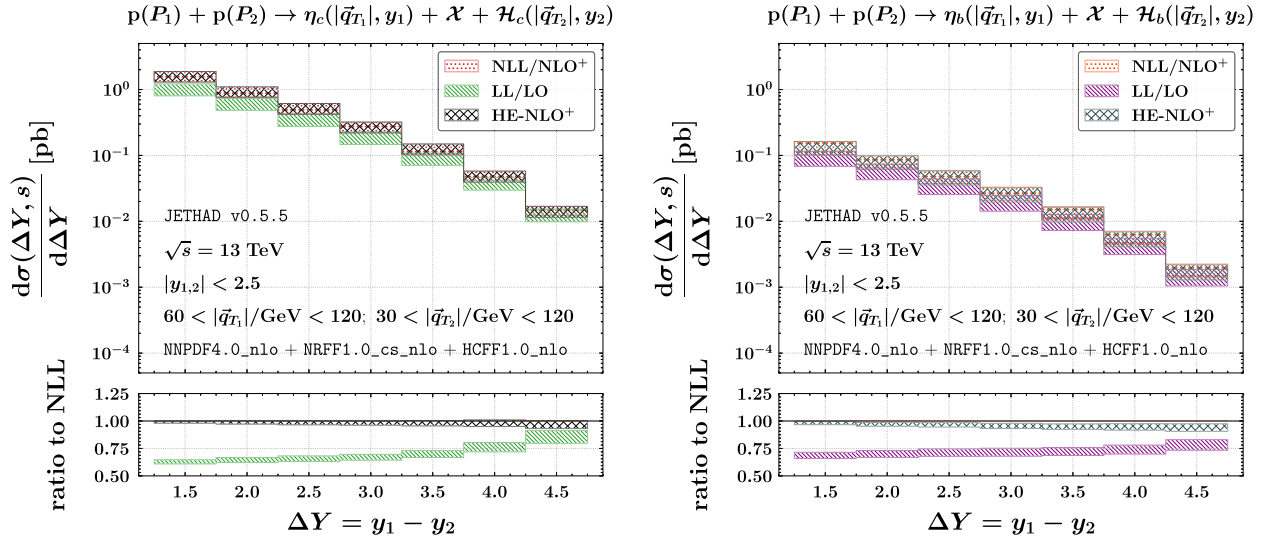
FIG. 15. Rapidity distributions for the semi-inclusive hadroproduction of an \eta_c (left) or \eta_b (right) meson in association with a heavy-light hadron, \mathcal{H}_c or \mathcal{H}_b , respectively, at \sqrt{s} = 13 TeV. Shaded bands in the main panels represent the combined uncertainty from MHOUs, LDMEs, and multidimensional phase-space integration. The ancillary panels below the main plots show the ratio of LL/LO and HE-NLO + predictions to NLL/NLO + , with bands capturing MHOUs only.
