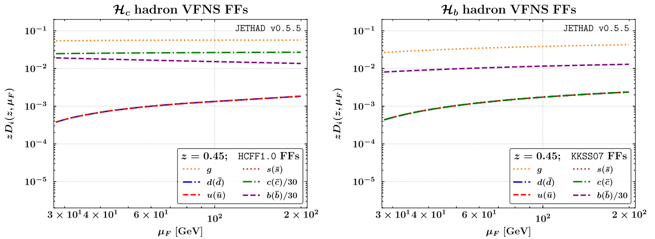
FIG. 13. Factorization scale dependence, at z \equiv \langle z \rangle \simeq 4.5 \times 10^{-1} , of HCFF1.0 NLO FFs depicting \mathcal{H}_c hadron emission (left), and of KKSS07 NLO FFs [230,231] describing \mathcal{H}_b hadron production (right).
