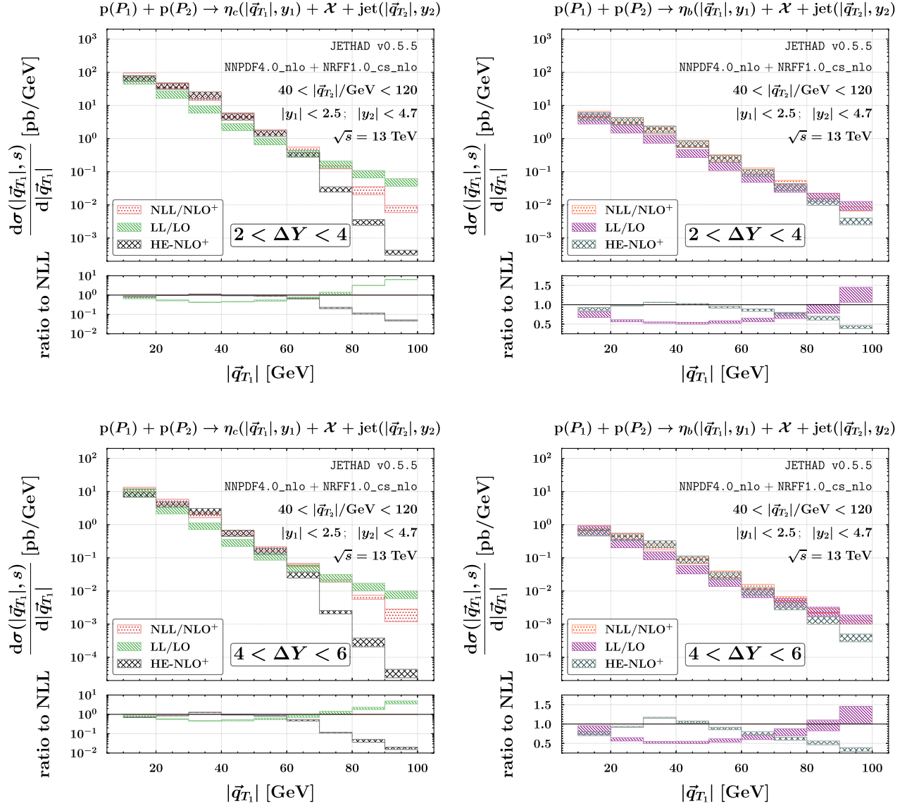
FIG. 18. Transverse momentum distributions for the semi-inclusive hadroproduction of an \eta_c (left) or \eta_b (right) meson in association with a jet, at \sqrt{s} = 13 TeV, and for 2 < \Delta Y < 4 (upper) or 4 < \Delta Y < 6 (lower) rapidity separation intervals. The shaded bands in the main panels represent the combined uncertainty from MHOU, LDMEs, and multidimensional phase-space integration. The ancillary panels below the main plots display the ratio of the LL/LO and HE-NLO + predictions to the NLL/NLO + result, with bands capturing MHOU only.
