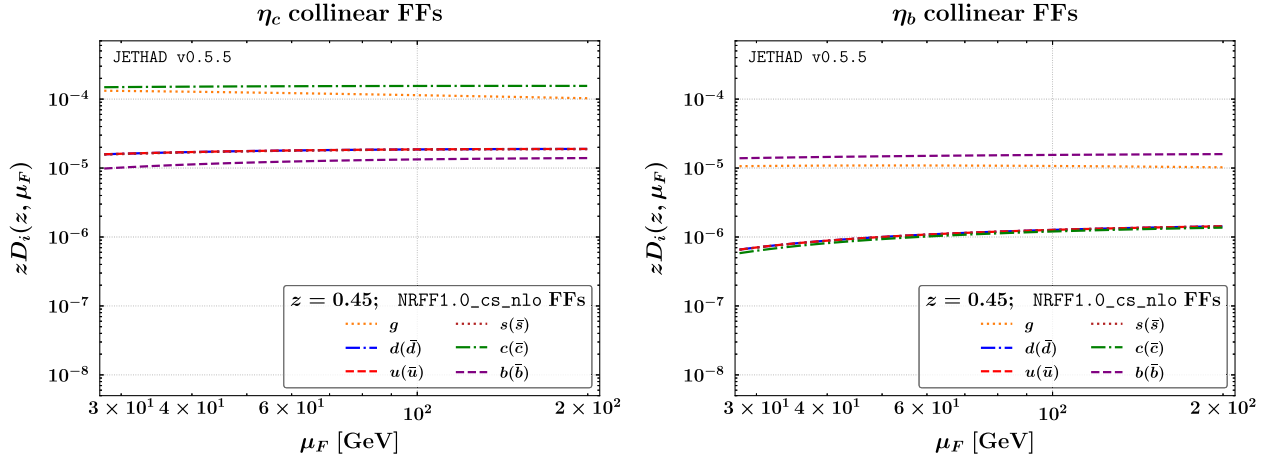
FIG. 11. Factorization scale dependence, at z \equiv \langle z \rangle \simeq 4.5 \times 10^{-1} , of NRFF1.0 NLO FFs [223] depicting \eta_c[{}^1S_0^{(1)}] (left) and \eta_b[{}^1S_0^{(1)}] (right) pseudoscalar quarkonium production. For simplicity, the analysis is performed using only the central value of the LDMEs.
