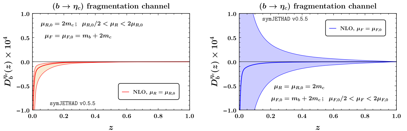
FIG. 5. NRQCD [b \rightarrow \eta_c, \text{lower}] fragmentation channel at NLO for \mu_{R,0} = 2m_c and \mu_{F,0} = m_b + 2m_c . Left plot: \mu_R runs from \mu_{R,0}/2 to 2\mu_{R,0} , while \mu_F is fixed at \mu_{F,0} . Right plot: \mu_R is fixed at \mu_{R,0} , while \mu_F runs from \mu_{F,0}/2 to 2\mu_{F,0} .
