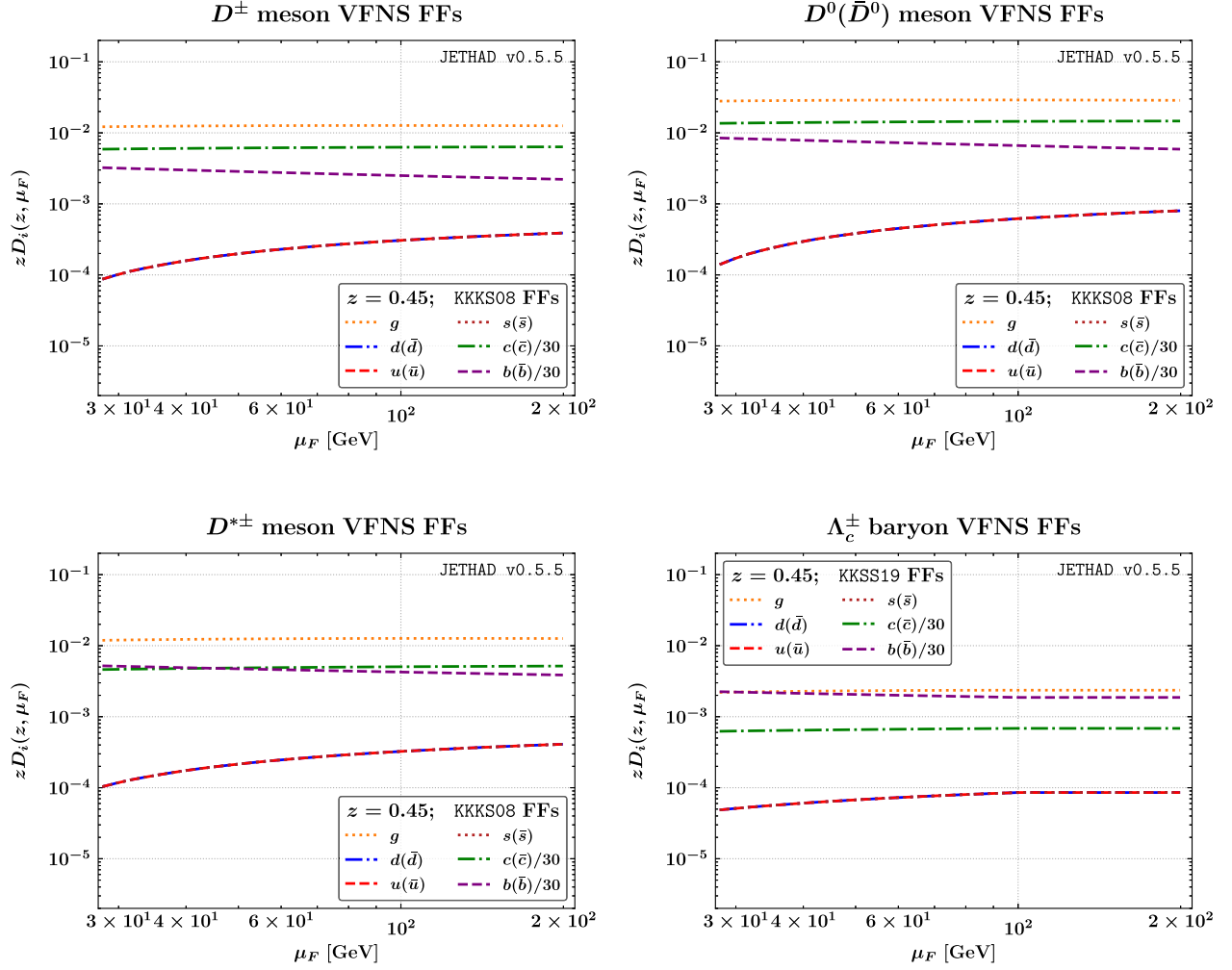
FIG. 12. Factorization scale dependence, at z \equiv \langle z \rangle \simeq 4.5 \times 10^{-1} , of KKKS08 NLO FFs [227,228] depicting D^\pm (upper left), D^0(\bar{D}^0) (upper right), and D^{*\pm} (lower left) meson emissions, and of KKKS19 NLO FFs [229] describing \Lambda_c^\pm baryon production (lower right).
