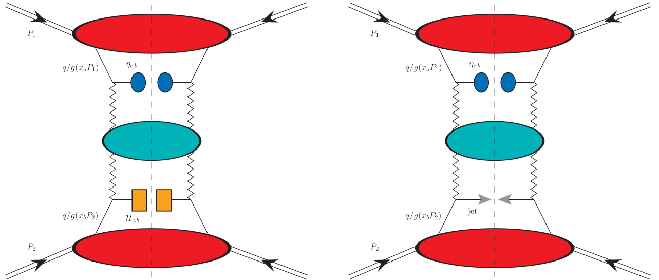
FIG. 14. Hybrid factorization for the semi-inclusive hadroproduction of a \eta_{c,b} quarkonium accompanied by a \mathcal{H}_{c,b} hadron (left) or a light jet (right). Blue ovals and orange squares, respectively, represent \eta_{c,b} and \mathcal{H}_{c,b} collinear FFs, while gray arrows portray jet emissions. Red ovals depict parent-proton collinear PDFs. The BFKL Green's function (turquoise blob) is connected to the two singly off-shell emission functions by wavy Reggeon lines.
