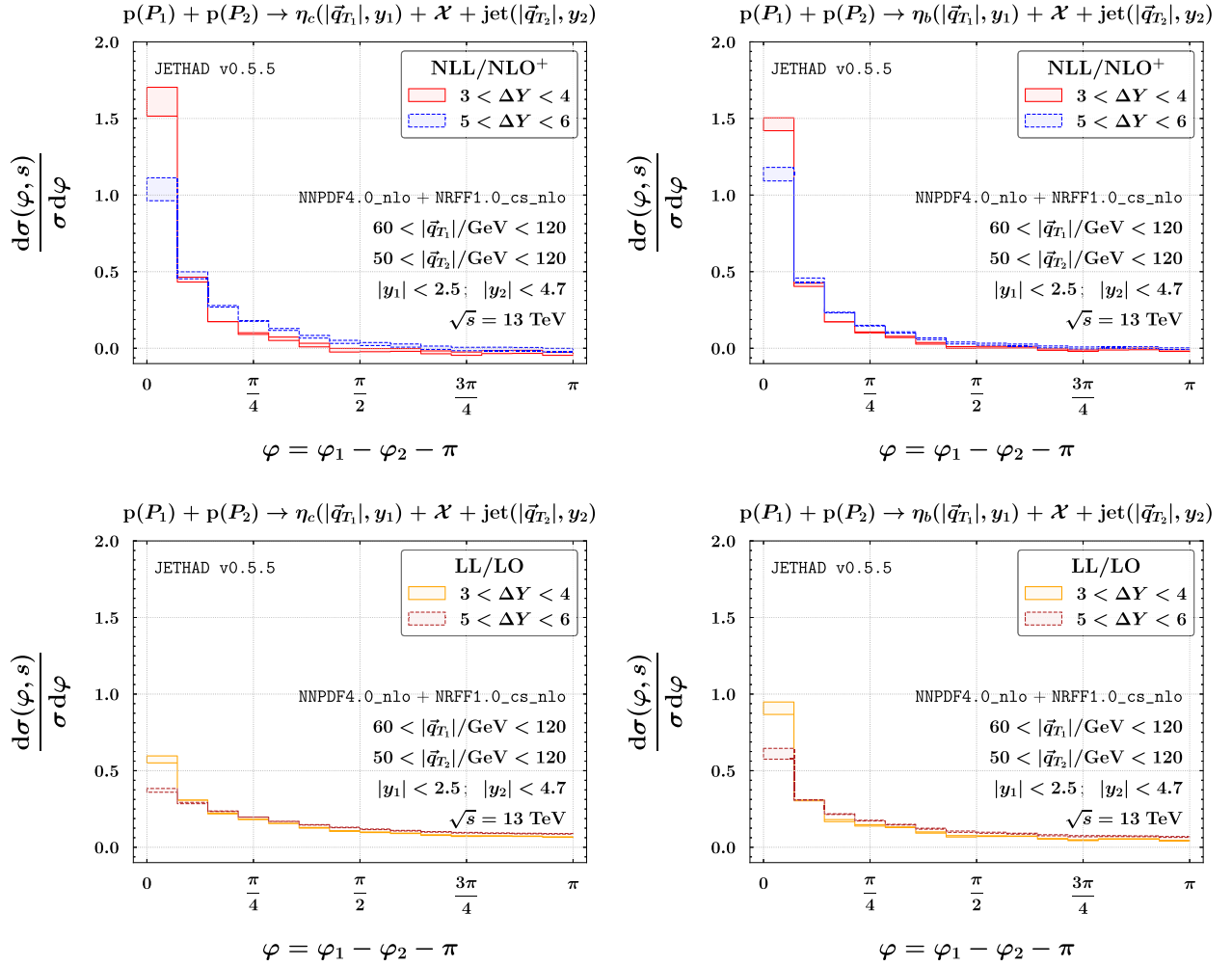
FIG. 17. Angular multiplicities for the semi-inclusive hadroproduction of an \eta_c (left) or \eta_b (right) meson in association with the jet, at \sqrt{s} = 13 TeV. Predictions in the upper (lower) plots are computed at NLL/NLO + (LL/LO) accuracy within the hybrid factorization framework. The shaded bands in the main panels represent the combined uncertainty from MHOUs and multidimensional phase-space integration.
