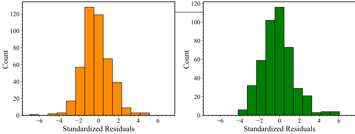
FIG. 10. The distribution of the standardized residuals for models I (orange) and II (green). There are 15 bins in region [-7, 7] .
