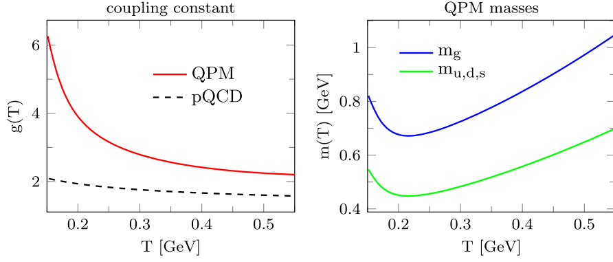
FIG. 6. Left: the coupling g as a function of T for pQCD calculation [black dashed line, from [69]] and QPM (red solid line, for N_f = 3 ). Right: the gluon and quark quasiparticle masses as functions of T .
