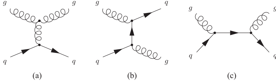
FIG. 8. Leading-order Feynman diagrams of the quark-gluon scatterings. (a) t -channel. (b) u -channel. (c) s -channel.
