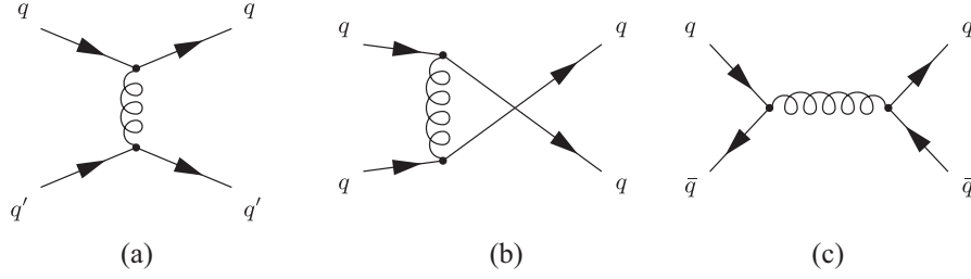
FIG. 7. Leading-order Feynman diagrams of the quark-quark scatterings. (a) t -channel. (b) u -channel. (c) s -channel.
