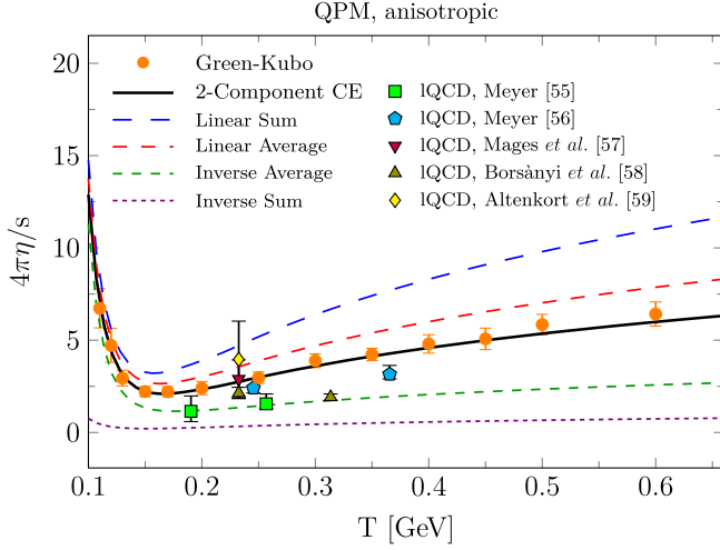
FIG. 5. Ratio shear viscosity over entropy density 4\pi\eta/s in the full 2-component Chapman-Enskog approximation (black full line), compared to the Green-Kubo results, to various combinations of the 1 component results for each of the two species, and various lattice QCD data from [55] (green squares), [56] (cyan pentagon), [57] (purple downward triangle), [58] (brown upward triangles) and [59] (yellow diamond). The calculations have been performed in the QPM, anisotropic case; all the parameters are listed in Table V (check Appendixes B and E for further details).
