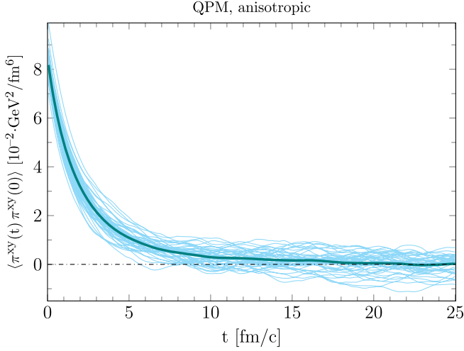
FIG. 4. Behavior of \langle \pi^{xy}(t) \pi^{xy}(0) \rangle with respect to t at a temperature T = 0.5 \text{ GeV} in the QPM, anisotropic case (check Appendixes B and E for details). In cyan, we show the results for 45 different numerical events, in dark blue their average, which highlights a clear exponential behavior.
