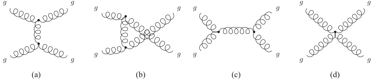
FIG. 9. Leading-order Feynman diagrams of the gluon-gluon scatterings. (a) t -channel. (b) u -channel. (c) s -channel. (d) 4-point.
