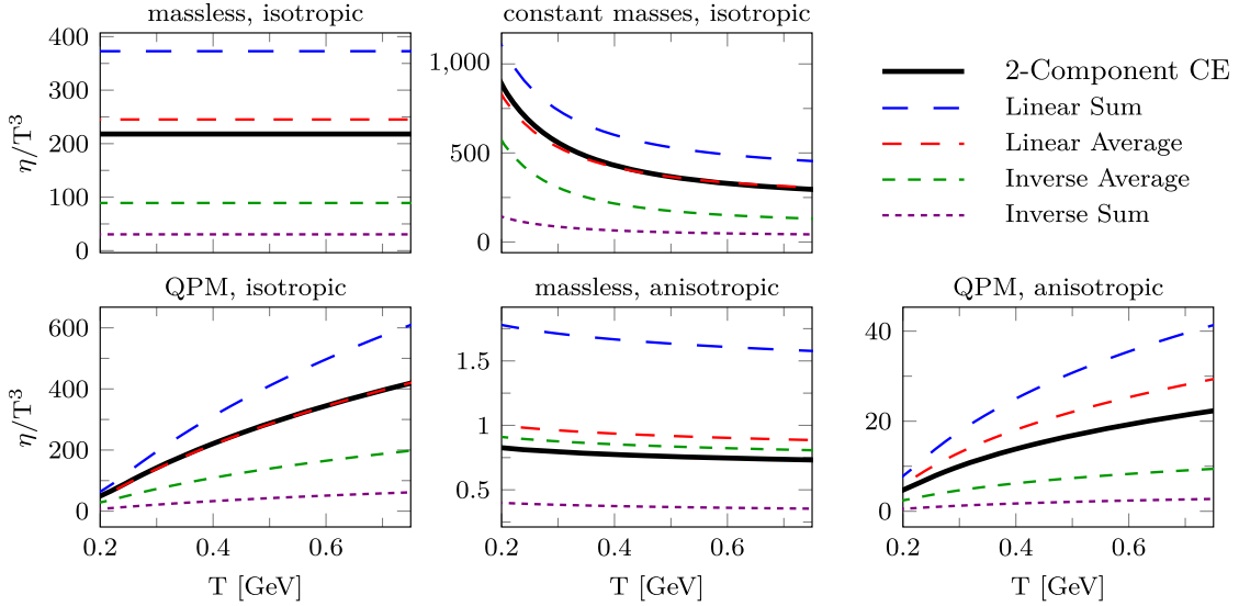
FIG. 1. Scaled shear viscosity \eta/T^3 vs T , for five different configurations of masses and cross sections. We compare the full 2-component result for \eta (black full line) with various interpolations of the 1-component results for each of the two species. Both the five configurations and the various 1-component \eta combinations are described in the main text, as well as in Appendixes B and E.
