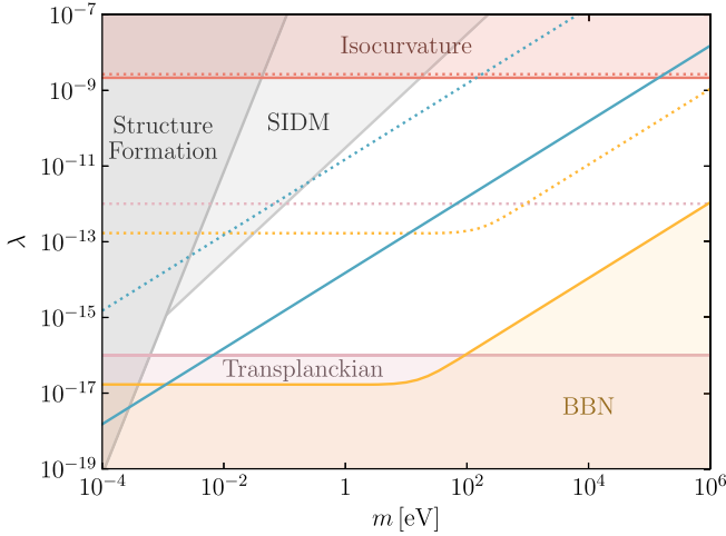
FIG. 2. Parameter space for inflationary production of scalar DM with a quartic potential [see Eq. (25)]. The blue line indicates parameters that produce the correct DM relic abundance for H_I = 10^{10} GeV and N_{\text{tot}} = 80 (assuming instantaneous reheating). Colored regions indicate constraints on this production scenario, including overproduction of isocurvature fluctuations (see right plot of Fig. 1), violation of N_{\text{eff}} constraints at the time of BBN, and transplanckian initial conditions \phi_{0,i} > M_{\text{pl}} . (Note that all parameters below the blue line are also constrained due to overclosure of the universe.) Dotted lines show these curves for H_I = 10^{12} GeV. In gray, we show late-time constraints on self-interacting dark matter (SIDM) and disruption of structure formation [52].
