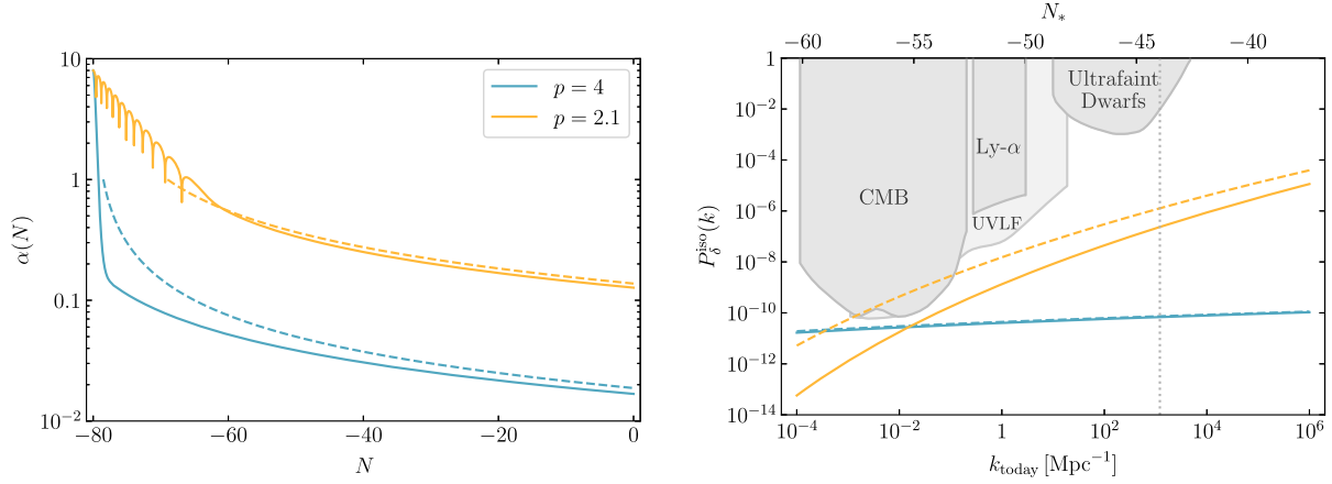
FIG. 1. Left: Evolution of \alpha [see Eq. (2)] as a function of e -folds N during inflation. We take the inflationary Hubble scale to be H_I = 10^{12} GeV in this plot. The spectator begins with \alpha_i \gg 1 at the start of inflation N_i = -80 . Initially, \alpha(N) oscillates and decreases in magnitude exponentially. Once \alpha < 1 , it decreases as 1/N . Dashed lines show the analytic approximation in Eq. (12). We show evolutions for two choices of potential V(\phi) \sim \phi^p . The blue curve has \kappa = \mathcal{O}(1) , while the orange has small \kappa . In accordance with Eq. (12), the latter results in much larger values of \alpha . Right: Primordial isocurvature spectrum for scalar DM with the same potentials as in the left plot. Dashed lines show the analytic approximation in Eq. (21). In both numerical and analytic curves, we include the constant factor from late-time evolution [see Eq. (33)], which for quartic DM with mass m = 10 eV applies to the left of the gray dotted line [see Eq. (31)]. The tilt of the spectrum is related to \alpha at horizon crossing N_* (shown on the top axis), as in Eq. (22). For \kappa = \mathcal{O}(1) , this generically results in a small blue tilt. For smaller \kappa , as in the orange curve, the tilt can be much stronger. In gray, we show constraints on the primordial isocurvature spectrum from observations of the CMB [46], ultraviolet luminosity function (UVLF) [47], Lyman- \alpha forest [48,49], and ultrafaint dwarf galaxies [49] (see also Ref. [50]). To avoid these constraints, the normalizations of the potentials are fixed at \lambda = 10^{-9} [as in Eq. (25)] for the blue curve and \Lambda = 4.4 \times 10^{11} GeV [as in Eq. (6)] for the orange curve. Note that the total matter power spectrum will be the sum of the isocurvature and adiabatic fluctuations [see Eq. (33)].
