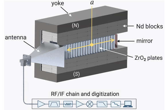
FIG. 1. Schematic view of the DALI(PoP) prototype. A tunnel yoke holds an array of Nd blocks that generates a dipolelike magnetic field. Ambient axions are converted into microwave photons, which are collected by the antenna. The resonator, composed of 20 \text{ZrO}_2 layers and enclosed by a copper mirror, enhances the weak axion-induced signal to an observable level. The detected signal is subsequently processed by the readout chain shown below (from left to right: amplifier, bandpass filter, attenuator, amplifier, down-converter, low-pass filter, analog-to-digital converter, and data storage). The haloscope is housed in a Faraday cage to suppress external spurious signals (not shown). The magnet is segmented along its longitudinal axis.
