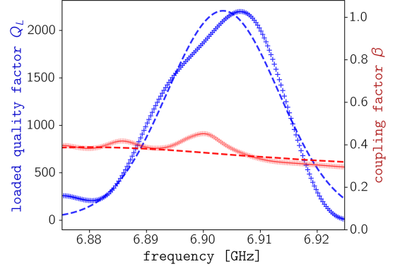
FIG. 3. Quality factor and coupling factor. Measured quality factor data are shown in blue. The full width at half maximum for a fit, represented by a blue dashed line, is \sim 20 MHz. In the present prototype configuration, the receiver is undercoupled. The observed optical power coupling factor \beta is depicted in red, while broadband data ( \sim 5 – 8 GHz) are smoothed with a SG baseline using a window size W = 201 and polynomial order d = 1 , shown by a red dashed line as a reference. Throughout this work, Q_L and \beta are taken from the measured data, not from the fitted or smoothed curves.
