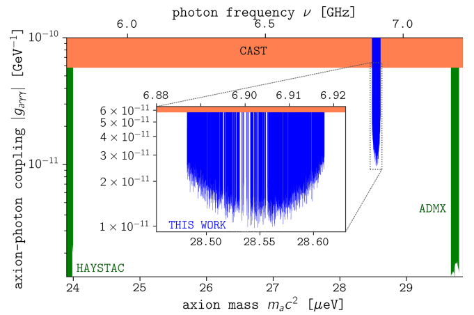
FIG. 5. New exclusion region (blue) at 90% CL. Narrow gaps indicate masked bins and vetoed neighborhoods around above-threshold excursions. Other laboratory-based constraints in the vicinity of the newly excluded region are also shown [27–30].
