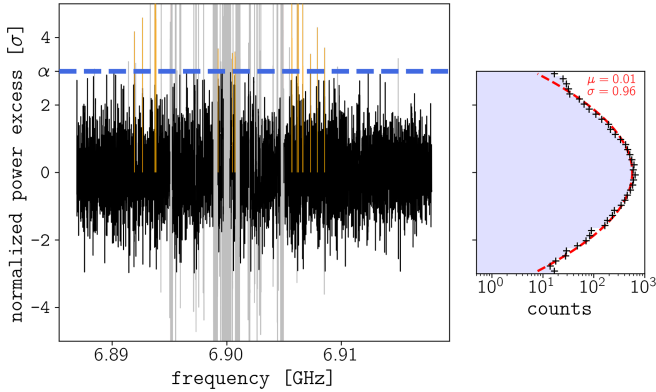
FIG. 4. Normalized, correlation-corrected grand spectrum (left). The black trace shows the retained bins, while gray traces denote masked bins; orange traces mark positive clusters flagged for rescan (see Table II). The blue dashed line indicates the detection threshold, \alpha = 3 . Right: Histogram of the retained normalized power excesses compared with a unit normal reference (red dashed). The grand spectrum is normalized by a robust (median) estimate of the noise scale over the instrumentally unmasked band, so that \alpha = 3 corresponds to 3\sigma ; the measured \hat{\sigma} = 0.96 of the retained bins reflects the symmetric vetoing of positive and negative excursions.
