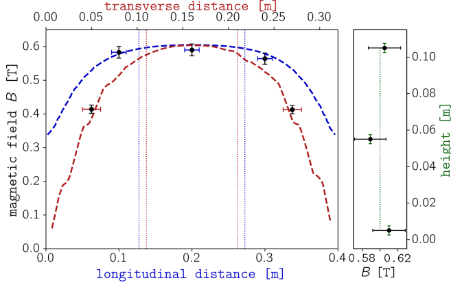
FIG. 2. Field simulation vs measurements. The magnet bore is approximately 30 (transverse) \times 11 (height) \times 40 (longitudinal) cm. Two one-dimensional profiles are extracted from the three-dimensional magnetic-field simulations: a center-longitudinal cut at half height (blue dashed) and a center-transverse cut (red dashed). The field generated by the magnets installed inside the steel yoke was simulated using Elmer FEM [22], employing Gmsh [23] to generate the three-dimensional meshes. The dotted lines indicate the resonator size ( 10 \times 10 \times 14.5 cm 3 ) in its centered configuration, shown for reference. Control Hall-probe measurements are shown with 3% vertical error bars and horizontal probe-positioning bars; the right inset displays three measurements along the bore height at the longitudinal center. The simulated field distribution is in good agreement with the measurements.
