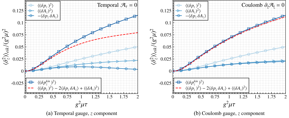
FIG. 11. Averaged eikonal quark kinetic momentum broadening \langle(\delta p_z^{\text{kin}})^2\rangle (square blue markers) and its decomposition (red dashed line), the same representation as in Fig. 9 but using \delta A_z^f instead of \delta A_z . Results are obtained in the temporal [panel (a) left] and Coulomb [panel (b) right] gauges.
