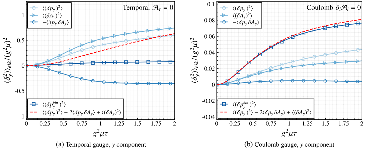
FIG. 10. Averaged eikonal quark kinetic momentum broadening \langle (\delta p_y^{\text{kin}})^2 \rangle (square blue markers) and its decomposition (red dashed line), the same representation as in Fig. 9 but using directly the value of the gauge potential \delta A_y (instead of the one obtained by integrating the corresponding component of the Lorentz force \delta A_y^f ). Results are obtained in the temporal [panel (a) left] and Coulomb [panel (b) right] gauges. Note the different scale on the vertical axis in the two plots.
