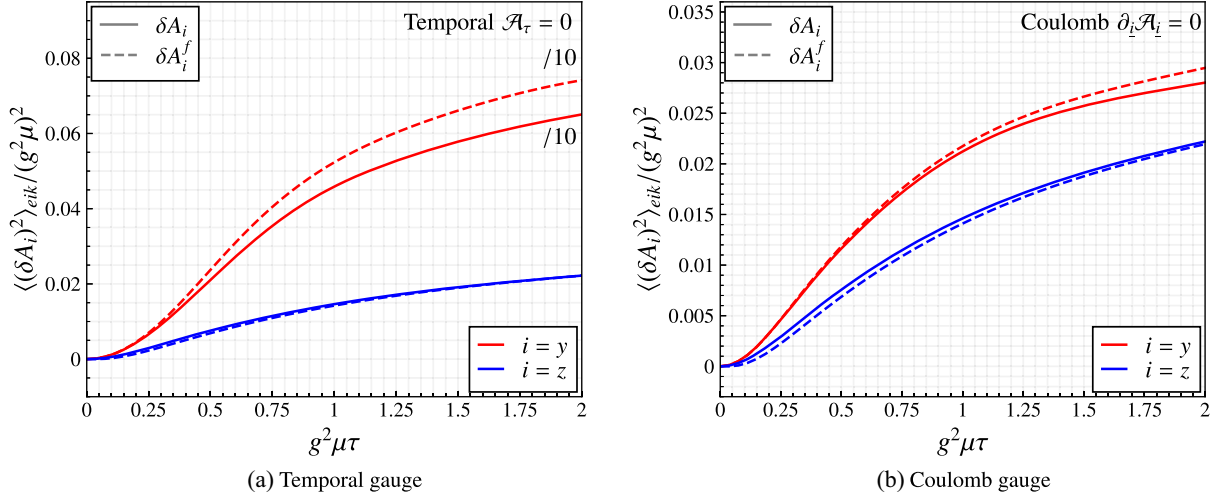
FIG. 8. Comparison between the averaged \langle(\delta A_i)^2\rangle_{eik} (solid line) and \langle(\delta A_i^f)^2\rangle_{eik} (dashed line) for eikonal quarks, rescaled by (g^2\mu)^2 , along the i = y direction (colored red) and the i = z direction (colored blue), in the temporal [panel (a) left] and Coulomb [panel (b) right] gauges, as a function of rescaled proper time g^2\mu\tau . Note that the values corresponding to the y direction in the temporal gauge are divided by 10.
