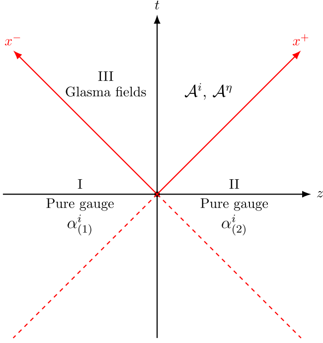
FIG. 1. Illustration of the gauge potential in different regions: pure gauges from individual nucleus in Regions I and II, the resulting glasma field after the collision in Region III, and the vanishing fields in the backward light cone.
