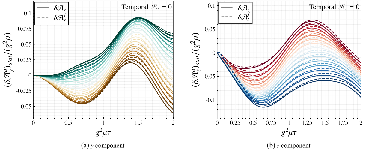
FIG. 4. Comparison between the same color component a of \delta\mathcal{A}_{i,\text{stat}}^a(\vec{x}_\perp) (solid line) and \delta\mathcal{A}_{i,\text{stat}}^{f,a}(\vec{x}_\perp) (dashed line) for static quarks, rescaled by g^2\mu , along the i = y direction (panel (a) left) and the i = z direction (panel (b) right), as a function of rescaled proper time g^2\mu\tau . Different colors correspond to different trajectories, computed at neighboring lattice locations \vec{x}_\perp , with n_{\text{traj}} = 15 distinct trajectories shown. Results are extracted in the glasma temporal gauge.
