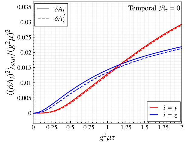
FIG. 5. Comparison between the averaged \langle(\delta\mathcal{A}_i)^2\rangle_{\text{stat}} (solid line) and \langle(\delta\mathcal{A}_i^f)^2\rangle_{\text{stat}} (dashed line) for static quarks, rescaled by (g^2\mu)^2 , along the i = y direction (colored red) and the i = z direction (colored blue), as a function of rescaled proper time g^2\mu\tau . Results are extracted in the glasma temporal gauge.
