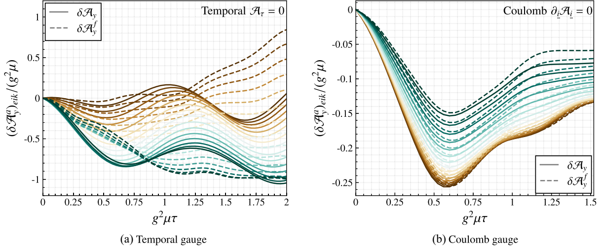
FIG. 6. Comparison between the same color component a along the transverse y direction of \delta\mathcal{A}_{y,eik}^a(\vec{x}_\perp) (solid line) and \delta\mathcal{A}_{y,eik}^{f,a}(\vec{x}_\perp) (dashed line) for eikonal quarks, rescaled by g^2\mu , in the temporal [panel (a) left] and Coulomb [panel (b) right] gauges, as a function of rescaled proper time g^2\mu\tau . Different colors correspond to different trajectories, starting from neighboring lattice locations \vec{x}_\perp and computed along the quark trajectory, with n_{\text{traj}} = 15 distinct trajectories shown.
