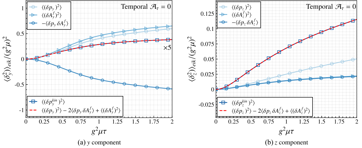
FIG. 9. Averaged eikonal quark kinetic momentum broadening \langle (\delta p_i^{\text{kin}})^2 \rangle (square blue markers) and its decomposition (red dashed line) in the canonical momentum broadening \langle (\delta p_i)^2 \rangle (circle blue markers), the squared gauge potential variation extracted from the Lorentz force \langle (\delta A_i)^2 \rangle (triangle blue markers) and the cross term \langle \delta p_i \delta A_i \rangle (diamond blue markers). Each contribution is rescaled as \langle \delta_i^2 \rangle / (g^2\mu)^2 and represented in terms of the dimensionless proper time g^2\mu\tau . Results are obtained in the temporal gauge, for the i = y [panel (a) left] and i = z [panel (b) right] directions. Note that both the kinetic momentum broadening and the sum of the different terms in the decomposition along the y direction are multiplied by 5.
