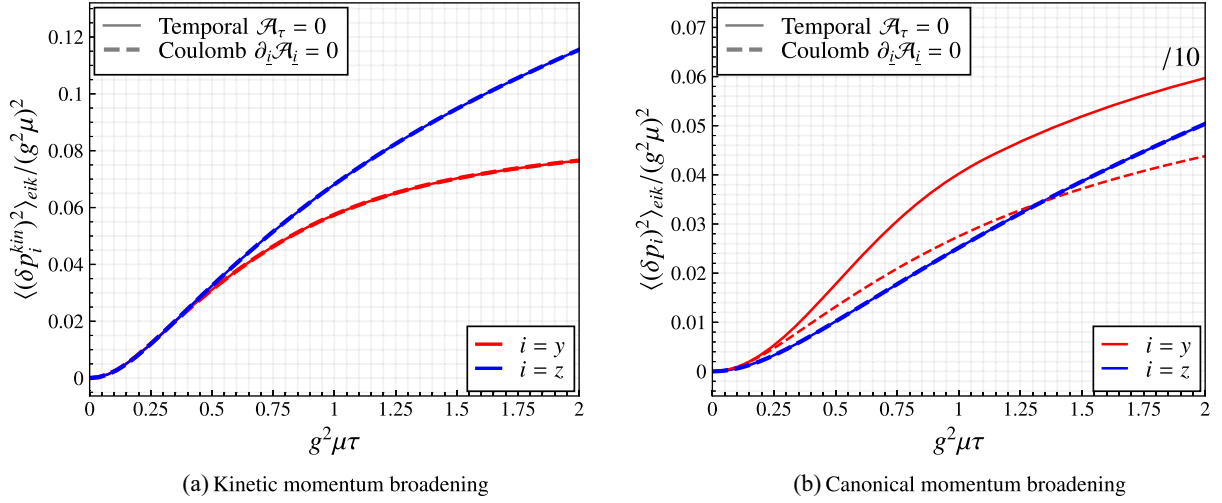
FIG. 2. Kinetic [panel (a) left] and canonical [panel (b) right] momentum broadening for eikonal quarks, scaled by (g^2 \mu)^2 , as a function of g^2 \mu \tau , for the i = y transverse component (colored red) and the i = z longitudinal component (colored blue), extracted in the temporal (solid line) and Coulomb (dashed line) gauges. Note that the value for the y component of the canonical momentum broadening in the temporal gauge is divided by 10.
