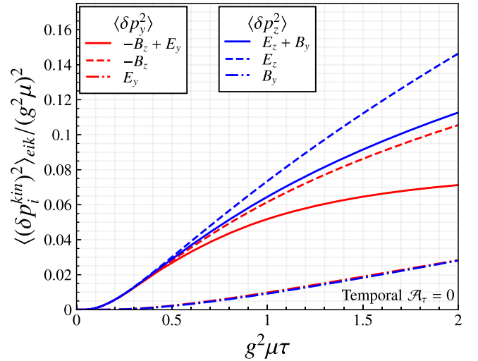
FIG. 3. Kinetic momentum broadening for eikonal quarks (full line), scaled by (g^2 \mu)^2 , as a function of g^2 \mu \tau , for the i = y transverse component (colored red) and the i = z longitudinal component (colored blue), extracted in the temporal gauge \mathcal{A}_\tau = 0 . The contribution to kinetic momentum broadening from only longitudinal electric or magnetic fields (dash line) and only from transverse fields (dash dotted line) are also represented.
