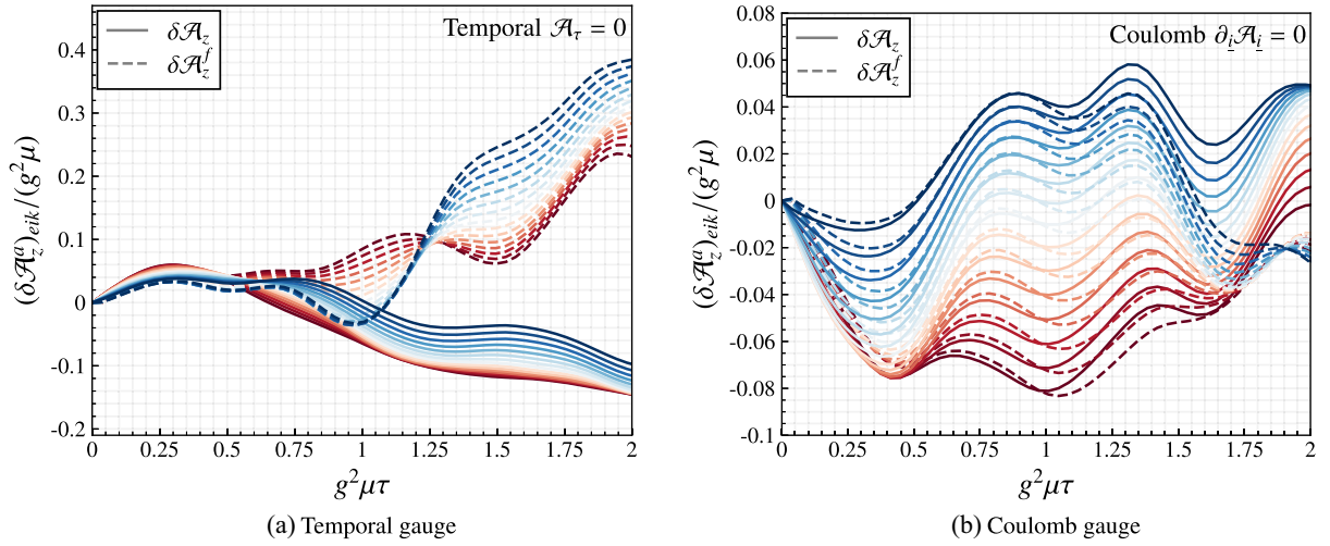
FIG. 7. Comparison between the same color component a along the longitudinal z direction of \delta\mathcal{A}_{z,eik}^a(\vec{x}_\perp) (solid line) and \delta\mathcal{A}_{z,eik}^{f,a}(\vec{x}_\perp) (dashed line) for eikonal quarks, rescaled by g^2\mu , in the temporal [panel (a) left] and Coulomb [panel (b) right] gauges, as a function of rescaled proper time g^2\mu\tau . Different colors correspond to different trajectories, starting from neighboring lattice locations \vec{x}_\perp and computed along the quark trajectory, with n_{\text{traj}} = 15 distinct trajectories shown.
