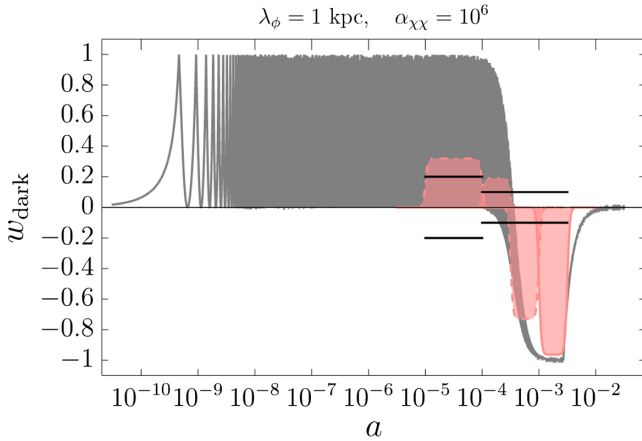
FIG. 4. Evolution of the instantaneous dark sector equation of state w_{\text{dark}} = p_{\text{dark}}/\rho_{\text{dark}} (solid gray) as a function of the scale factor a . The dark sector pressure p_{\text{dark}} and energy density \rho_{\text{dark}} are defined in Eqs. (10) and (11). The widths and amplitudes of the red bars represent the four scale-factor bins 1, 2, 3, 4 [see Eq. (13)] used in our analysis and the averaged equation of state \bar{w}_{\text{dark}}^{(i)} within them. The black lines mark the boundaries of the allowed ranges of \bar{w}_{\text{dark}}^{(i)} ; we consider parameter space with red bars protruding the black lines as ruled out.
