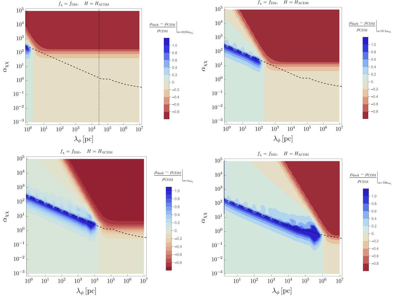
FIG. 15. Fractional of \rho_{\text{dark}} from \rho_{\text{CDM}} . The blue region signifies the mixed DM f_\phi/f_\chi = \mathcal{O}(1) . The blobby part near the case \phi_{\text{rise}}\phi_0\phi_*/\phi_{\text{DM}} -case \phi_{\text{rise}}\phi_{\text{DM}} boundary is because the amplitude of \phi_{\text{DM}} is set by the relative field-space velocity \dot{\phi}_{\text{lin-osc}} - \dot{\phi}_* when \phi_* \approx \phi_0 , and this relative velocity depends on the phase of \phi_{\text{lin-osc}} at that time. In the bottom right figure, \lambda_\phi \lesssim 1 pc was not simulated because that regime is computationally expensive.
