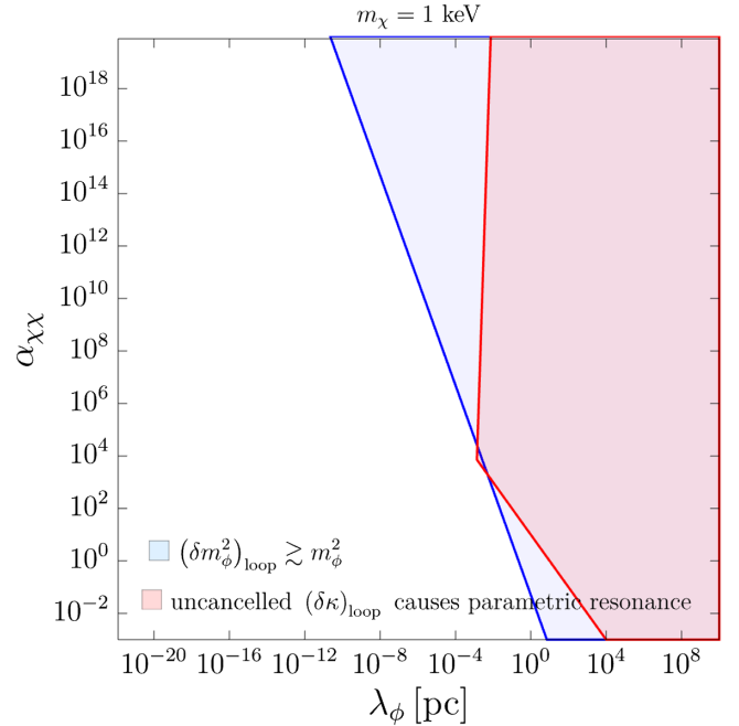
FIG. 12. Fine-tuned parameter space for m_\chi = 1 keV. In the blue region, the squared mass of the scalar mediator m_\phi^2 is smaller than the expected correction to it from \chi loop, (\delta m_\phi^2)_{\text{loop}} . In the red region, the \chi -loop-induced quartic coupling (\delta\kappa)_{\text{loop}} would cause parametric resonance, thus invalidating our analysis, unless this (\delta\kappa)_{\text{loop}} is somehow canceled by other contributions to the quartic coupling.
