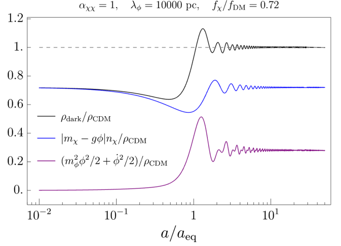
FIG. 10. Mixed DM scenario. Here, we plot as function of the scale factor \chi 's effective energy density |m_\chi - g\phi|n_\chi , \phi 's energy density m_\phi^2 \phi^2 / 2 + \dot{\phi}^2 / 2 , and their sum \rho_{\text{dark}} , all normalized to the backward-in-time extrapolation of the CDM energy density \rho_{\text{CDM}} . The plot shows that the initially negligible average energy density of \phi rises considerably at some point and contributes significantly to \rho_{\text{dark}} at late times. Thus, the DM at late times is an \mathcal{O}(1) mix of \chi and \phi , both behaving as CDM. In this plot, the parameters are chosen to hit the correct total DM abundance today.
