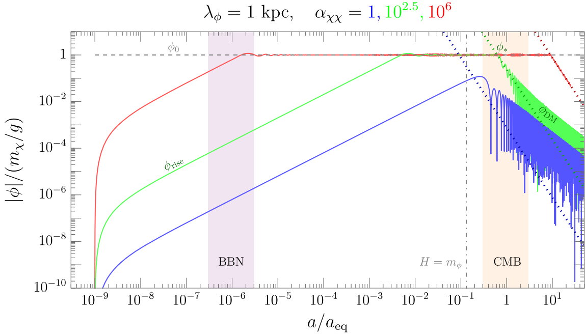
FIG. 2. Evolution of the background scalar field \phi as a function of the scale factor a for \lambda_\phi = 1 kpc and \alpha_{\chi\chi} = 1 (solid blue), \alpha_{\chi\chi} = 10^{2.5} (solid green), \alpha_{\chi\chi} = 10^6 (solid red). Here, we set a_i = 10^{-9} , \phi(a_i) = 0 , and \dot{\phi}(a_i) = 0 , and numerically evolve \phi using the equation of motion Eq. (8). The gray dashed line is the linear finite-density minimum \phi_0 \equiv m_\chi/g defined in Eq. (6). The dotted lines are the quadratic finite-density minima \phi_* \equiv gn_\chi/m_\phi^2 , defined in Eq. (7), corresponding to the values of \alpha_{\chi\chi} matching their colors. The dark green labels “ \phi_{\text{rise}} ” and “ \phi_{\text{DM}} ” indicate, respectively, where in the evolution of the green line the \phi field tracks the attractor solution \phi_{\text{rise}} \equiv (3\alpha_{\chi\chi}f_\chi/4)\phi_0(a/a_{\text{eq}}) , defined in Eq. (9), and oscillates as CDM, with an amplitude scaling as \propto a^{-3/2} . The colored bands labeled “BBN” and “CMB” indicate the very rough points where BBN and recombination take place.
