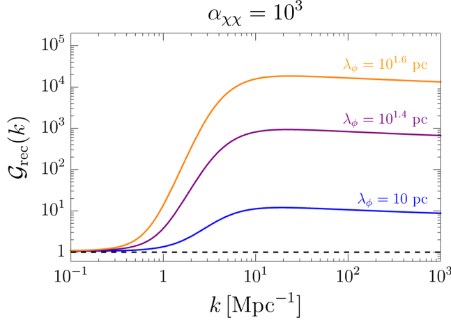
FIG. 6. Extra growth of DM density contrast \mathcal{G}_{\text{rec}}(k) = [\delta_\chi(k)/\delta_\chi^{\text{ACDM}}]_{\text{rec}} by the epoch of recombination as a function of comoving wave number k . Here, the \delta_\chi and \delta_\chi^{\text{ACDM}} are evolved according to Eq. (18) and Eq. (21), respectively, with the dark-force parameters as indicated in the plot.
