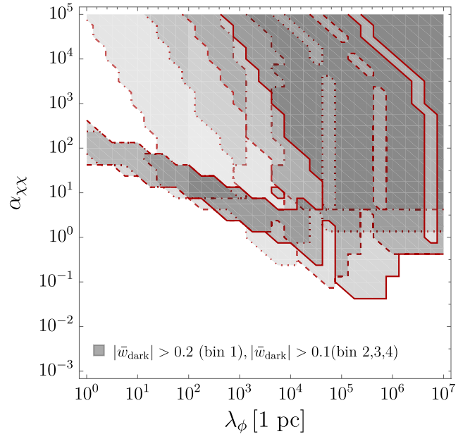
FIG. 14. Background limits from each scale-factor bin, Eq. (13). The limits from bin 1, 2, 3, and 4 are shown in solid, dashed, dotted, and dot dashed.
