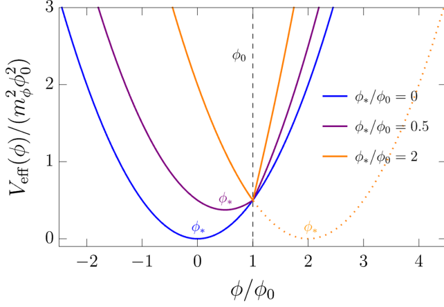
FIG. 1. Effective potential of \phi ; cf. Eq. (5). The labels “ \phi_0 ” and “ \phi_* ” mark the locations of the linear finite-density minimum \phi_0 = m_\chi/g and the quadratic finite-density minimum \phi_* = gn_\chi/m_\phi^2 . In the \phi_*/\phi_0 = 2 case, the \phi_* exists mathematically {the dotted line shows what V_{\text{eff}} would be if the |\phi_0 - \phi| in Eq. (5) is replaced with \phi_0 - \phi without the absolute value}, but in this case, \phi_* cannot be reached because before \phi can get there, the slope of the linear potential flips sign at \phi = \phi_0 .
