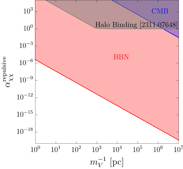
FIG. 8. Limits on repulsive dark forces. In the red (blue) region, the energy density of the Universe is dominated by the scalar potential’s contribution m_V^2(V^0)^2/2 \propto z^{-6} at redshifts z \sim 10^{10} ( z \sim 10^3 ), thus spoiling BBN (CMB). The region labeled “Halo Binding” is ruled out by the observation of ultrafaint dwarf galaxies because the repulsive forces would overcome gravity and destabilize the dwarf galaxies [11].
