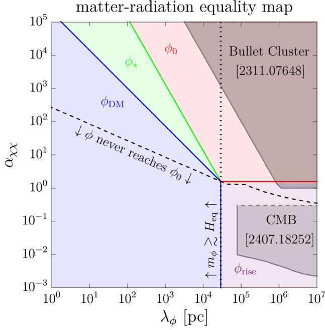
FIG. 3. Types of solutions of \phi at matter-radiation equality. For example, in the red region, \phi is at \phi_0 \equiv m_\chi/g , the linear finite-density minimum. In the green region, \phi is at \phi_* \equiv gn_\chi/m_\phi^2 , the quadratic finite-density minimum. In the purple region, it is at \phi_{\text{rise}} \equiv (3\alpha_{\chi\chi}f_\chi/4)\phi_0(a/a_{\text{eq}}) , the attractor solution initially tracked by \phi for a wide range of initial conditions, and in the blue region, it is at \phi_{\text{DM}} , which is a CDM-like solution where \phi oscillates with its bare mass with an amplitude that scales as a^{-3/2} . In the red region, the dark sector behaves as dark energy to the left of the dotted line and as dark radiation to the right of the dotted line. Also shown are the regions ruled out by Bullet Cluster observation [4] and small-coupling analysis of the CMB data [22]. The CMB limit has a ceiling because Ref. [22] employs a small- \alpha_{\chi\chi} approximation in their analysis. We show a rough approximation to this ceiling as a dashed-gray upper boundary, corresponding to \alpha_{\chi\chi} \sim 0.3 . Above (below) the black dashed line, \phi does (does not) reach \phi_0 , which corresponds to the large (small) mass-change regime, i.e., the \phi_{\text{rise}} \rightarrow \phi_0 \rightarrow \phi_* \rightarrow \phi_{\text{DM}} ( \phi_{\text{rise}} \rightarrow \phi_{\text{DM}} ) case.
