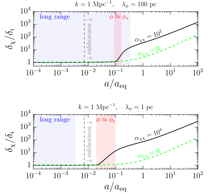
FIG. 5. The evolution of the DM density contrast \delta_\chi = \delta n_\chi / n_\chi (solid black line, normalized to its initial, superhorizon value) as a function of the scale factor a (normalized to that at matter-radiation equality, a_{\text{eq}} ). Here, we follow the mode with comoving wave number k = 1 \text{ Mpc}^{-1} and set the dark-force parameters as indicated in the plots. The gray dashed line marks the point where this mode becomes subhorizon. The black solid lines represent the evolution of \delta_\chi as dictated by Eq. (18), to be contrasted with the evolution in the absence of dark forces ( \alpha_{\chi\chi} = 0 ) as given by Eq. (21) and shown in dashed green lines. The light red region shows the region where \phi is expected to closely track \phi_* , in which the \Theta_* in Eqs. (18) and (19) is equal to unity. The light blue region indicates where the dark-force range is longer than the physical wavelength a/k of the mode. The top ( bottom ) plot corresponds to the case where the dark force is long-range ( \lambda_\phi \gg a/k ) (short-range \lambda_\phi \ll a/k ) when \phi \approx \phi_* . It can be seen that enhanced growth occurs in the light red region in either case. Furthermore, \delta_\chi appears to continue growing relative to the \Lambda CDM one even outside of the light red region. This is due to the speed \dot{\delta}_\chi acquired in the light red region.
