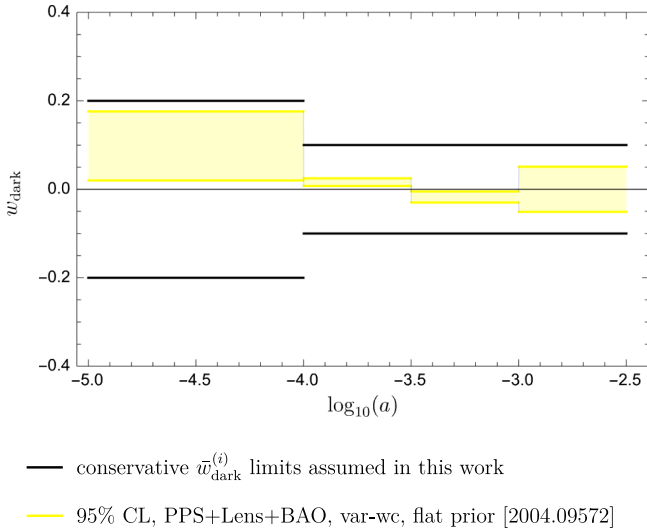
FIG. 13. Comparison between the conservative limits on \bar{w}_{\text{dark}}^{(i)} we assumed in our analysis, as given in Eq. (15), (black lines) and the allowed values of \bar{w}_{\text{dark}}^{(i)} from [37] (yellow).
