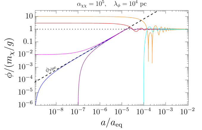
FIG. 9. Dynamical attractors of the background evolution of \phi . The solid lines are the evolutions of \phi obtained by solving Eq. (A1) with different initial conditions for \phi (and with \dot{\phi} = 0 initially). The plot shows that the \phi_{\text{rise}} solution defined in Eq. (A4) (dashed line) and also the linear finite-density minimum \phi_0 = m_\chi/g (dotted line) are attractors for a wide range of initial conditions. For the assumed values of \lambda_\phi and \alpha_{\chi\chi} , the \phi_* = gn_\chi/m_\phi^2 is far greater than \phi_0 = m_\chi/g and thus lies outside of the range of the plot.
