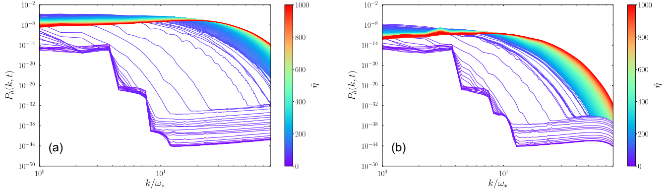
FIG. 4. The evolution of the Higgs field power spectrum P_h(k, t) as a function of the wave number, where \tilde{\tau} is the program variable time. The (a) and (b) panels correspond to q_h = 10^2 and q_h = 10^5 , respectively.
