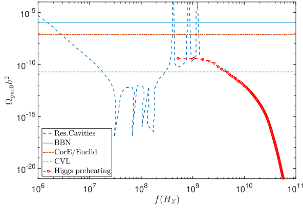
FIG. 6. The present-day GW energy density spectrum \Omega_{\text{gw},0} h^2 predicted in this work, compared with the projected sensitivity of resonant cavity detectors and indirect cosmological constraints. The benchmark parameters are \lambda_\phi = 10^{-13} , q_h = 10^2 , q_{\phi h} = 10^2 , and q_e = 10^{-6} .
