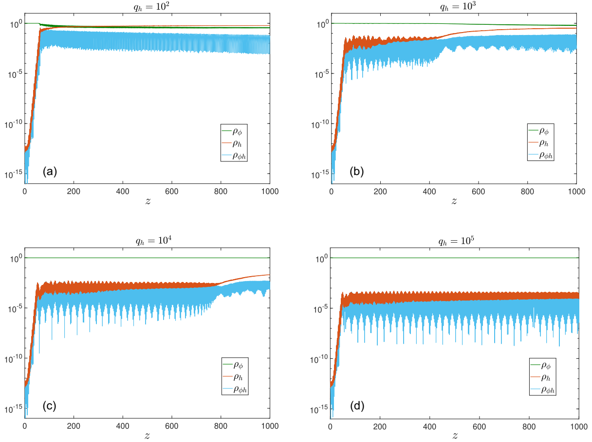
FIG. 2. The evolutions of the energy density of Higgs field \rho_h , inflaton field \rho_\phi , and interaction energy \rho_{\phi h} as a function of the conformal time, where the energy has been normalized to the total energy density. The parameters are set to \lambda_\phi = 10^{-13} , q_{\phi h} = 10^2 , and q_e = 10^{-6} . Panels (a)–(d) correspond to q_h = 10^2 , 10^3 , 10^4 , and 10^5 , respectively.
