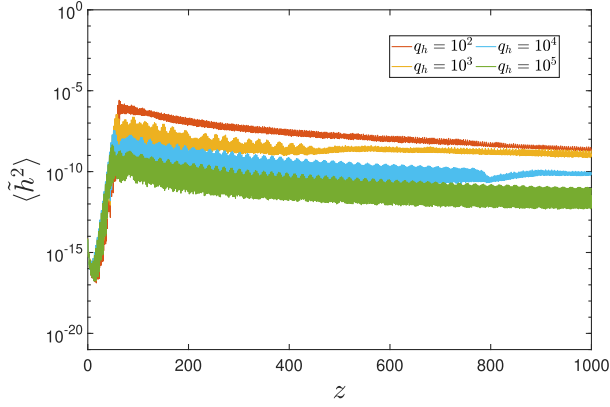
FIG. 3. The evolutions of the volume-averaged mean-square Higgs field \langle \tilde{h}^2 \rangle as a function of the dimensionless time z . The parameters are set to \lambda_\phi = 10^{-13} , q_{\phi h} = 10^2 , and q_e = 10^{-6} .
