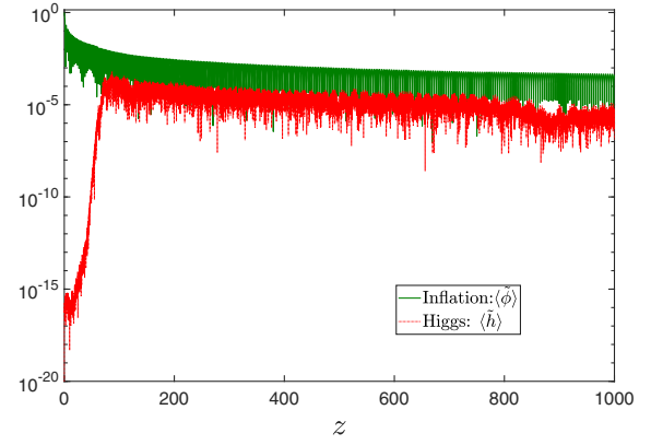
FIG. 1. Evolution of the Higgs and inflaton mean field values, where \lambda_\phi = 10^{-13} , q_{\phi h} = 10^2 , q_e = 10^{-6} , and q_h = 10^2 .
