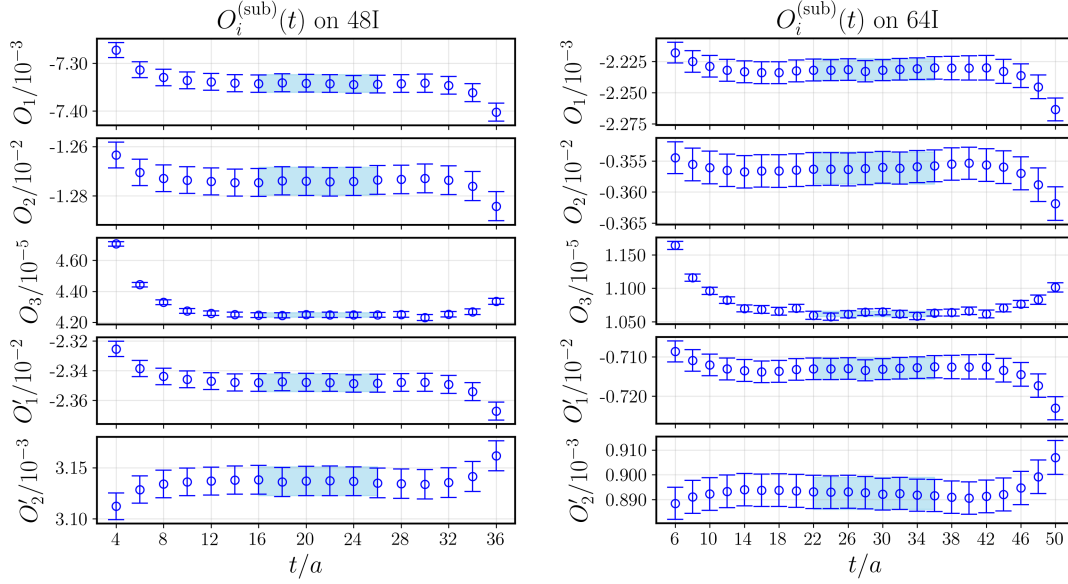
FIG. 6. Same as Fig. 4, but with 48I and 64I ensembles.
