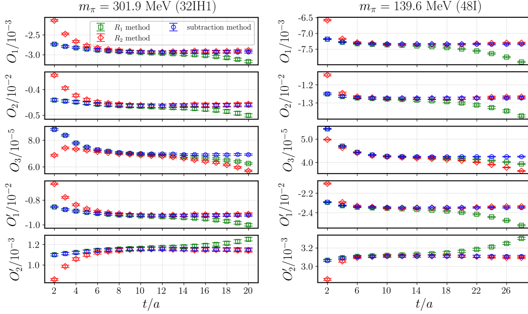
FIG. 3. Comparison between the effective bare matrix elements before subtraction of around-the-world effects, O_i^{(R_1)}(t) (green squares) and O_i^{(R_2)}(t) (red diamonds), and after subtraction, O_i^{(\text{sub})}(t_{\text{sep}}) (blue circles). The left and right panels present results at unphysical and physical pion mass, respectively.
