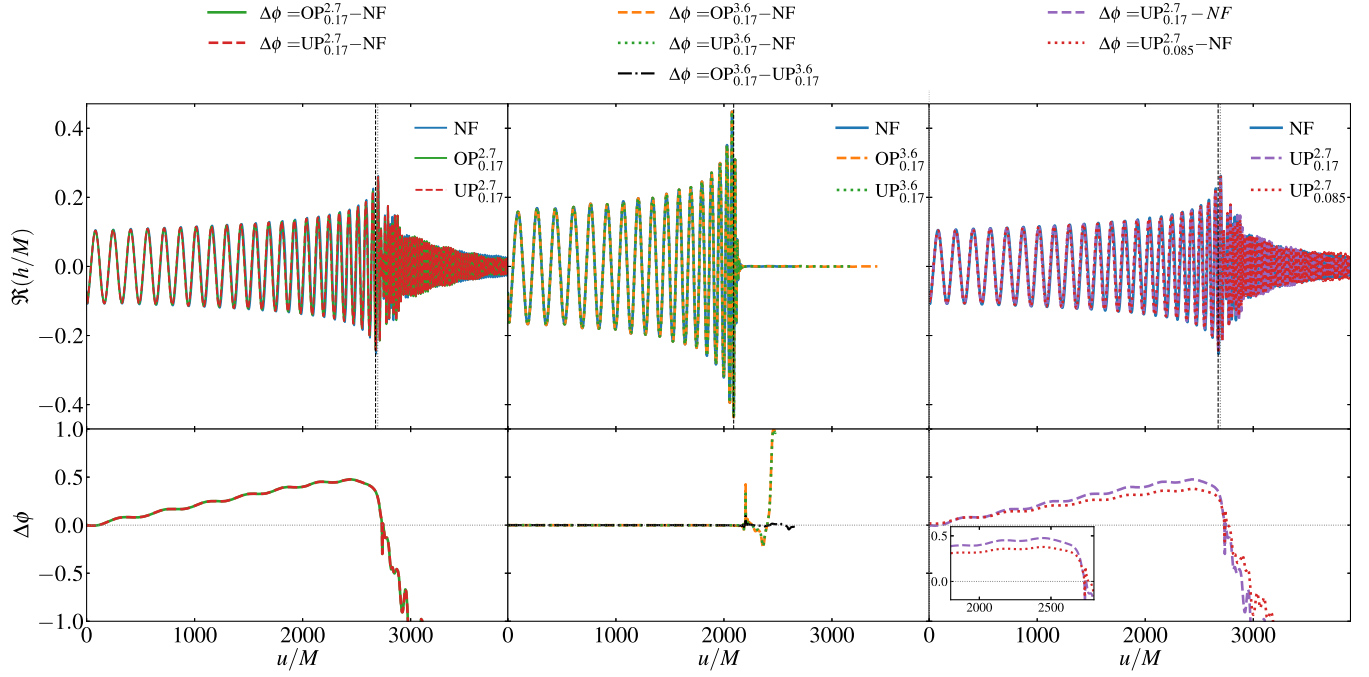
FIG. 5. Left: real part of the GW strain (top panel) and the corresponding phase differences (bottom panel) for different scalar field profiles extracted at a radius R_{\text{ext}} = 1000 . The UP and OP both show the same dephasing with the vacuum case (NF) of roughly 0.3 rad close to the merger. Middle: real part of the GW strain (top panel) and the corresponding phase differences (bottom panel) for different scalar field profiles with a total mass of M_{\text{tot}} = 3.6 , along with the NF of the same M_{\text{tot}} . Only a negligible dephasing is observed between the vacuum case and the configurations with the scalar field. Right: real part of the GW strain (top panel) and the corresponding phase differences (bottom panel) for two different masses, \mu = 0.17 and \mu = 0.085 . The lower scalar field mass exhibits a smaller accumulated dephasing relative to the vacuum case close to the merger, owing to the pressure term, as shown in the inset.
