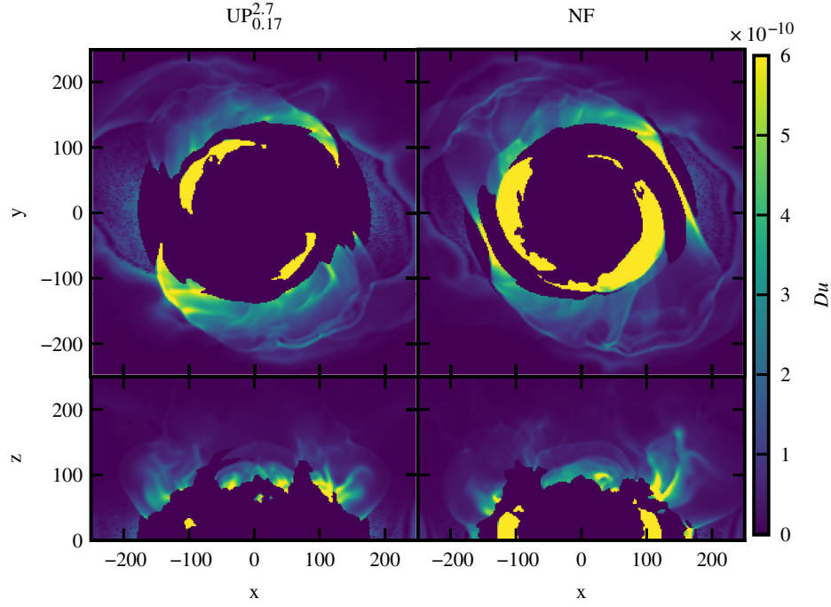
FIG. 6. Two-dimensional snapshots of unbound ejecta for the vacuum (NF) case and the uniform profile ( UP_{0.17}^{2.7} ) with scalar field mass \mu = 0.17 for M_{\text{tot}} = 2.7 binary extracted at an AMR refinement level l = 3 . Top panel: comparison in the equatorial plane, which is typically dominated by shock-driven ejecta, showing a clear suppression in the presence of the scalar field. Bottom panel: corresponding snapshots along the polar plane, confirming the overall reduction of the ejecta due to the scalar field. All snapshots are taken at t = 8800 .
