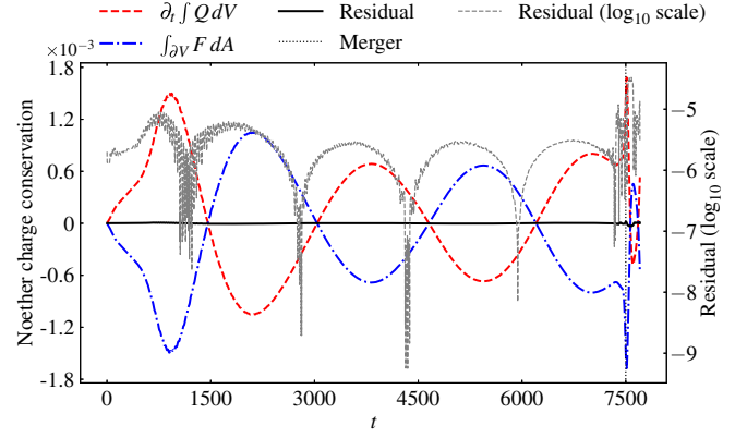
FIG. 2. Noether charge conservation plot for the 2.7 total mass binary for the uniform profile with the scalar field mass \mu = 0.085 , extracted at a radius of R = 40 . The red dotted lines represent the time derivative of the charge ( \int Q dV ), the blue dashed line is the flux ( \int F dA ), both are oscillatory, and the residual is shown in a black solid line and is conserved throughout the simulation. The axis on the right shows the residual on a log scale.
