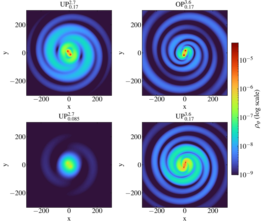
FIG. 4. Two-dimensional snapshots at t = 2000 of the scalar field energy density \rho_\phi . Top left: uniform profile, M_{\text{tot}} = 2.7 , \mu = 0.17 . Top right: overdense profile, M_{\text{tot}} = 3.6 , \mu = 0.17 . Bottom left: uniform profile, M_{\text{tot}} = 2.7 , \mu = 0.085 . Bottom right: uniform profile, M_{\text{tot}} = 3.6 , \mu = 0.17 . The lower-mass field ( \mu = 0.085 ) shows markedly reduced central accumulation, consistent with a stronger gradient pressure. The 3.6 mass binary simulations exhibit broader, more extended spiral-arm features, potentially due to higher oscillations of the scalar field and a deeper gravitational potential well.
