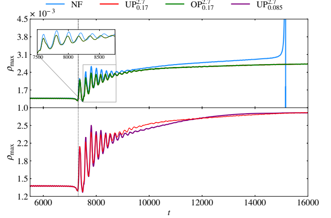
FIG. 9. Top panel: evolution of the baryonic central rest-mass density, \rho_{\text{max}} , through merger and into the postmerger phase for both the scalar field profiles (UP and OP) and for the vacuum reference (NF). The inset enlarges the first t \sim 10^3 after merger, showing suppressed oscillations in the presence of the field. Further, the black hole formation is also delayed relative to the vacuum case, as indicated by the energy density growth at t = 15000 . Bottom panel: evolution of the maximum baryonic rest-mass density across merger (vertical dotted line) and into the postmerger phase for two scalar field masses, \mu = 0.17 (red) and 0.085 (purple). Lowering the mass of the field increases the amplitude of oscillations in the initial stage of oscillations, followed by a marginally reduced value compared to the 0.17 case. In the presence of a scalar field, the postmerger oscillations of \rho_{\text{max}} are damped, due to an additional (gradient) pressure that opposes compression of the remnant.
