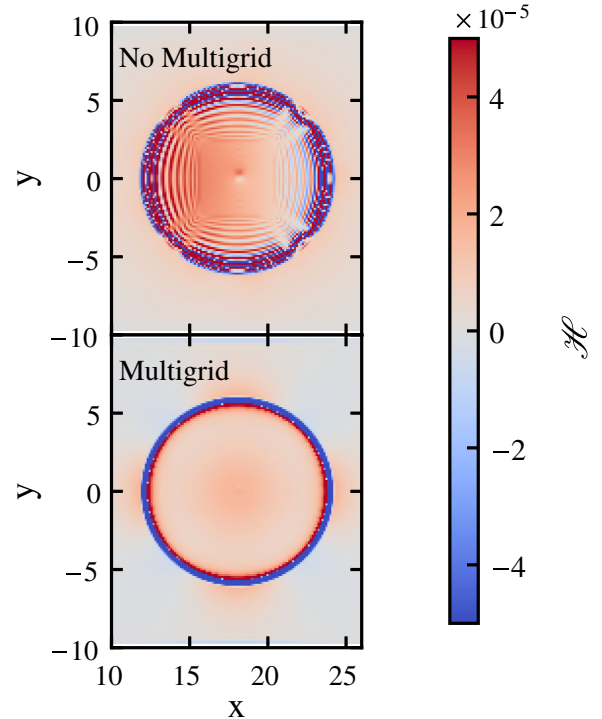
FIG. 12. Two-dimensional snapshot of the Hamiltonian constraint at t = 0 around a single star at the finest refinement level. Top: result without the multigrid solver. Bottom: result with multigrid, showing comparatively smoother and reduced constraint violations around and within the star.
