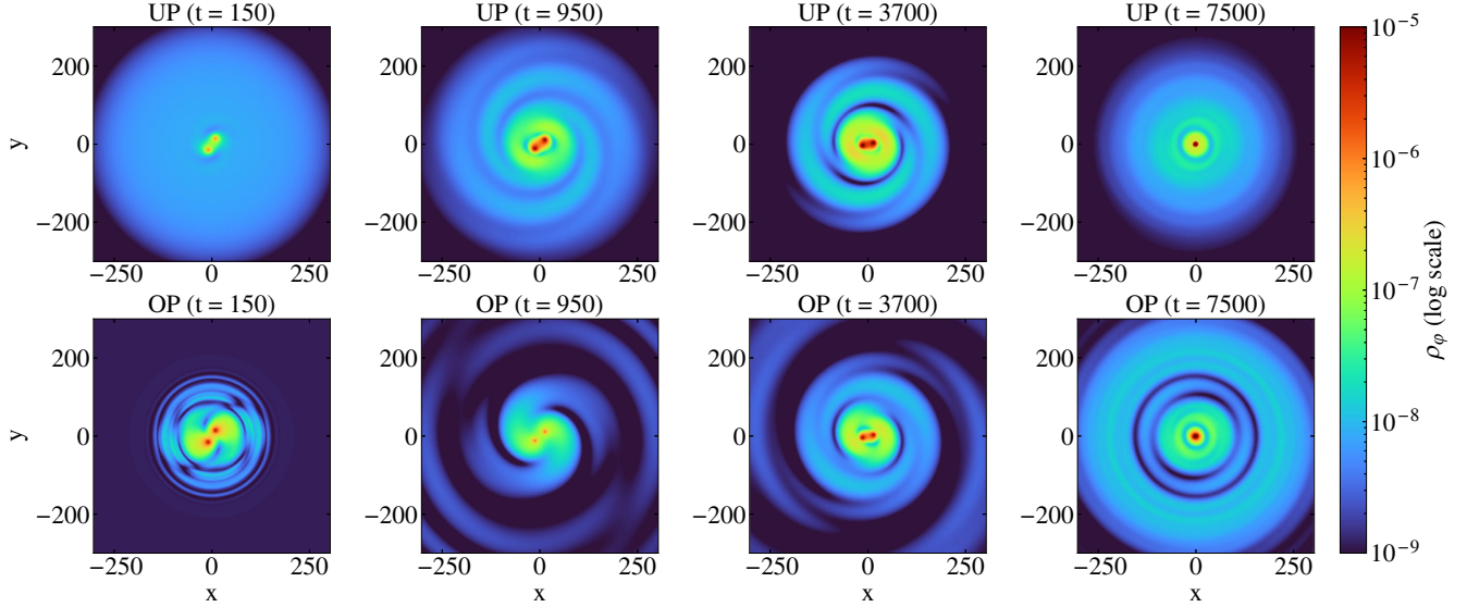
FIG. 1. Two-dimensional schematics showing the comparison of the energy densities for the two scalar field initial profiles. Top row: for the UP at different times starting from early-inspiral till the postmerger phase. Bottom row: energy densities snapshots for the overdense profile OP at the same time stamps of the simulation, showing localized enhancement close to the binary even at t = 150 . The UP is effectively a nearly homogeneous field initially, as the cut-off is set at a large radius. At later times, a corotating configuration develops, giving rise to characteristic spiral-arm features in the energy density.
