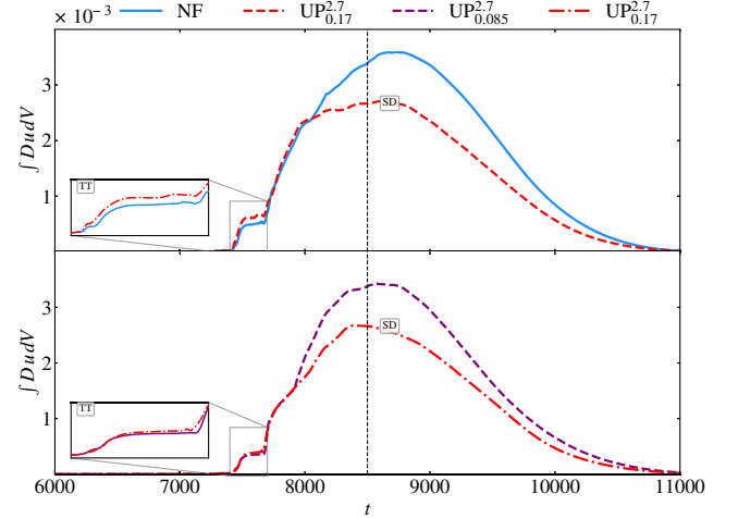
FIG. 7. Volume-integrated unbound ejecta mass at the AMR level l = 3 . Top panel: comparison between the UP_{0.17}^{2.7} and the vacuum (NF) case. Regions dominated by tidal and shock-driven ejecta are marked, with insets zooming in on the tidal-tail contribution. The scalar field enhances the tidal-tail ejecta while suppressing the shock-driven component, resulting in a net reduction of total ejecta. Bottom panel: comparison of the same for two scalar field masses, UP_{0.17}^{2.7} and UP_{0.085}^{2.7} . Reducing the scalar field mass shifts the behavior closer to the vacuum case, increasing the shock-driven ejecta while reducing the tidal-tail contribution.
