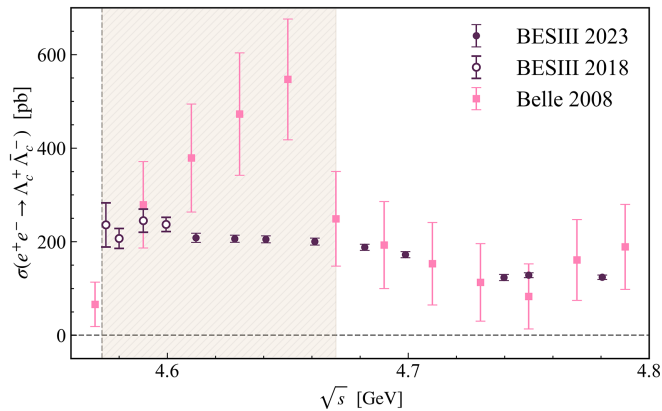
FIG. 1. Comparison of the e^+e^- \rightarrow \Lambda_c^+\bar{\Lambda}_c^- cross section data from Belle [21] and BESIII [26,27]. The shaded band highlights the region of significant tension between the two datasets above the \Lambda_c^+\bar{\Lambda}_c^- threshold, marked by the vertical dashed line.
