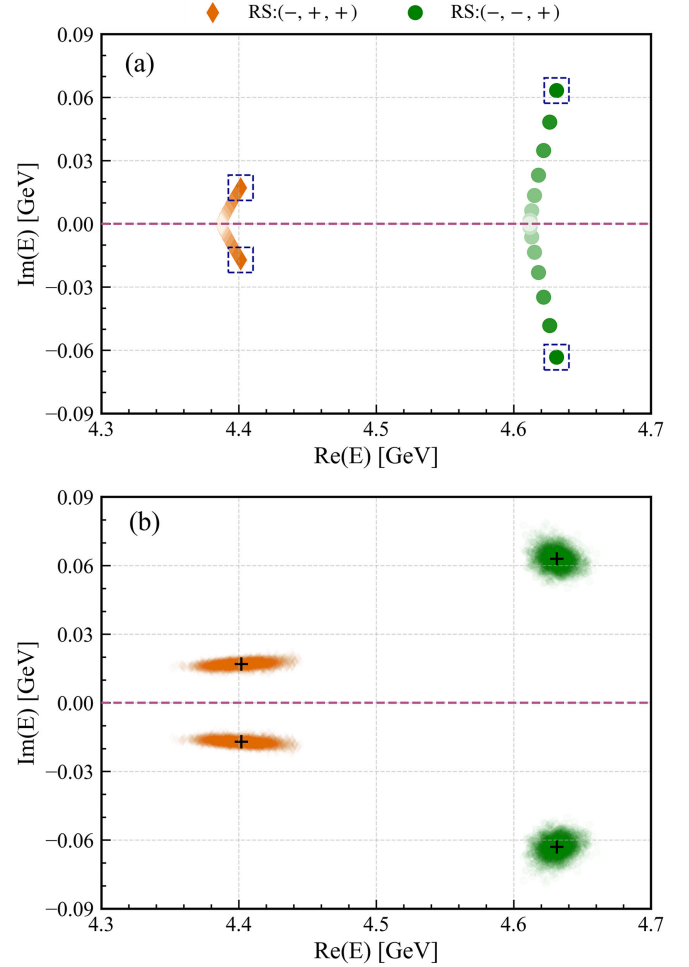
FIG. 5. Panels (a): Pole trajectories of \psi(4360) (orange diamonds) and \psi(4660) (green circles) on different Riemann sheets (RSs), obtained using the best-fit parameters, with the coupling constants g_{4S} or g_{5S} gradually reduced from their fitted values to zero. The pink horizontal dashed line denotes the real axis. The blue dashed boxes indicate the initial pole positions, while the color gradient from dark to light illustrates their evolution. Panels (b): Error regions of the pole positions on the corresponding Riemann sheets. The orange and green regions correspond to the \psi(4360) and \psi(4660) states, respectively. The black crosses mark the central values of the pole positions within the error intervals.
