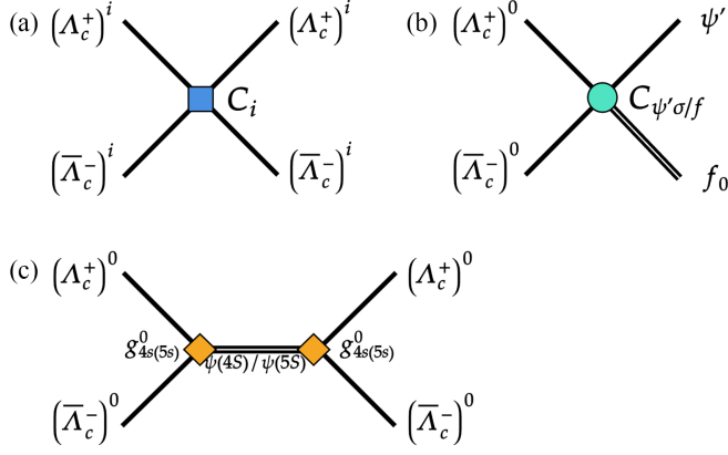
FIG. 2. (a), (b): Short-range contact potentials. (c): Effective potential mediated by the bare resonance states \psi(4S) or \psi(5S) .
