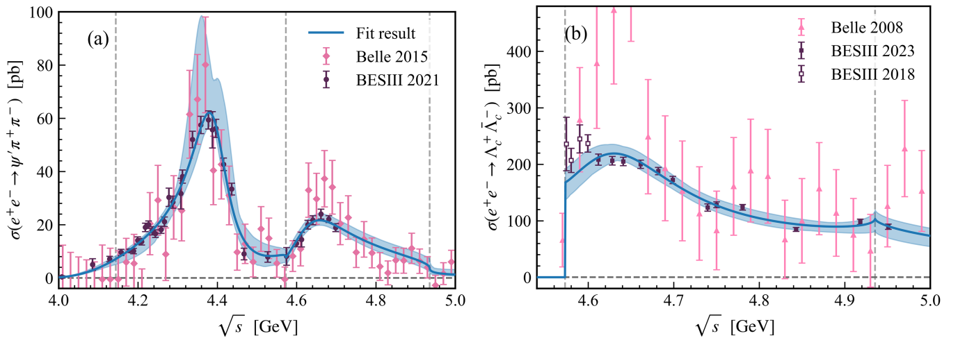
FIG. 4. Comparison of the fitted line shapes (blue solid line) with experimental measurements for (a) e^+e^- \rightarrow \psi'\pi^+\pi^- and (b) e^+e^- \rightarrow \Lambda_c^+\bar{\Lambda}_c^- . Data are from both Belle [21,23] (pink triangles and diamonds) and BESIII [25–27] (purple circles, purple boxes and hollow squares) collaborations. The vertical dashed lines indicate the relevant thresholds, from (a) to (b): \psi(2S)\sigma(500) , \Lambda_c^+\bar{\Lambda}_c^- , and \Xi_c^+\bar{\Xi}_c^- .
