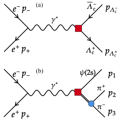
FIG. 3. Feynman diagrams for e^+e^- \rightarrow \Lambda_c^+ \bar{\Lambda}_c^- and e^+e^- \rightarrow \psi(2S) \sigma(500)/f_0(980) \rightarrow \psi(2S) \pi^+ \pi^- . Red square denotes the physical production amplitude and blue circle denotes the coupling between the \pi\pi system and the intermediate resonance.
