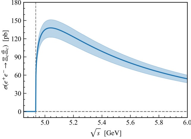
FIG. 6. Prediction of the \Xi_c \bar{\Xi}_c cross section.
