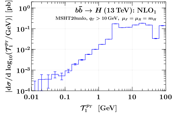
FIG. 3. Nonsingular T_1^{pT} spectrum for b\bar{b} \rightarrow H .
