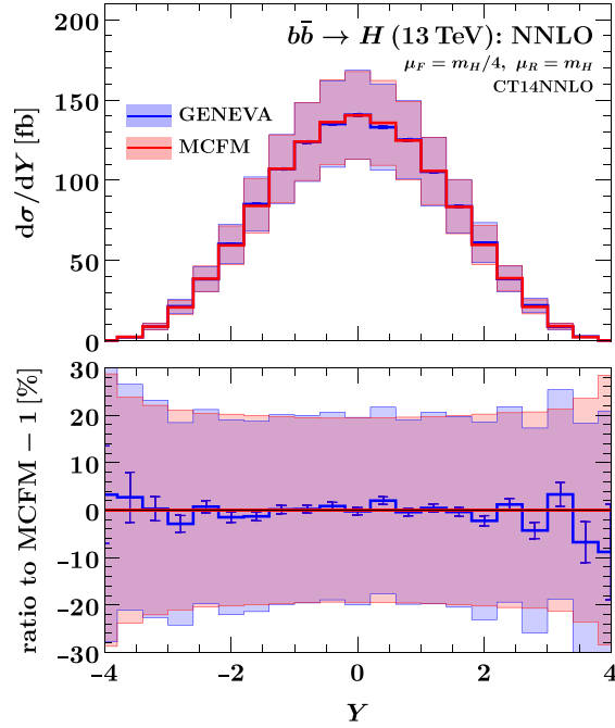
FIG. 1. Comparison between MCFM and GENEVA for the NNLO Higgs boson rapidity spectrum in b\bar{b} \rightarrow H . Uncertainty bands are obtained via a 7-pt. scale variation procedure.
