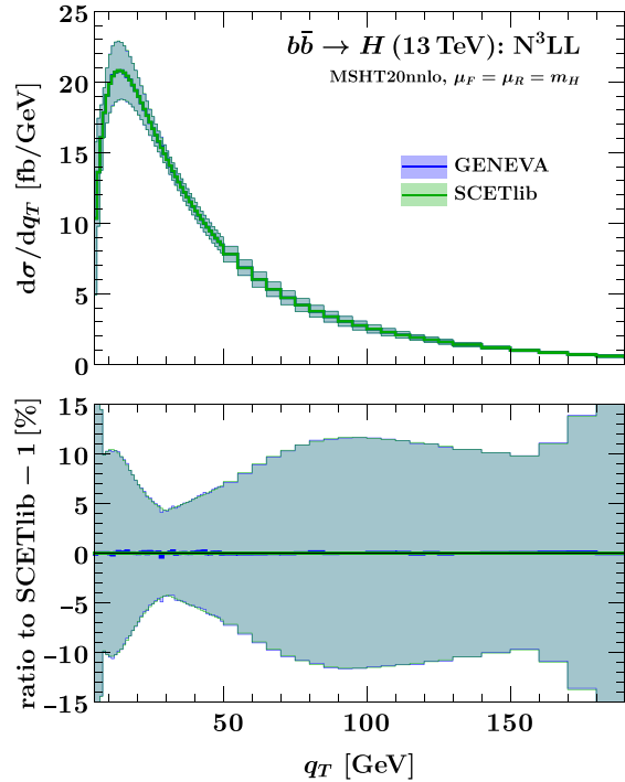
FIG. 2. Comparison between SCETlib and GENEVA for the N 3 LL Higgs boson q_T spectrum in b\bar{b} \rightarrow H . Uncertainty bands are obtained as explained in Appendix A.
