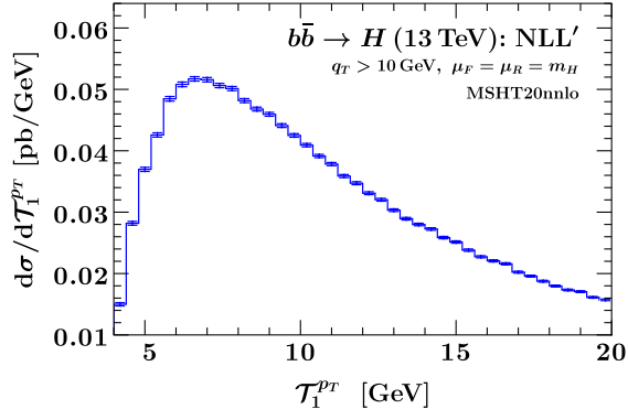
FIG. 4. Resummed T_1^{pr} spectrum for b\bar{b} \rightarrow H .
