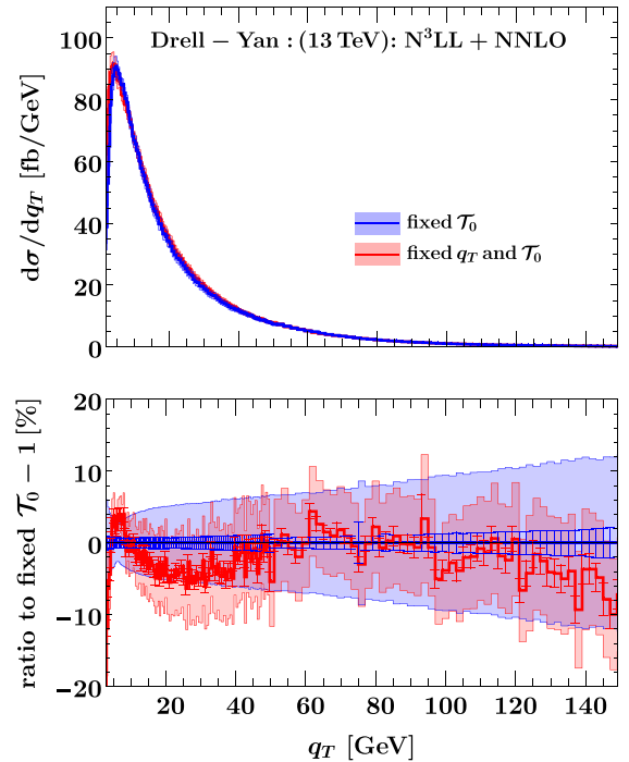
FIG. 11. Transverse momentum spectrum of the vector boson for the Drell-Yan process with different splitting mappings.
