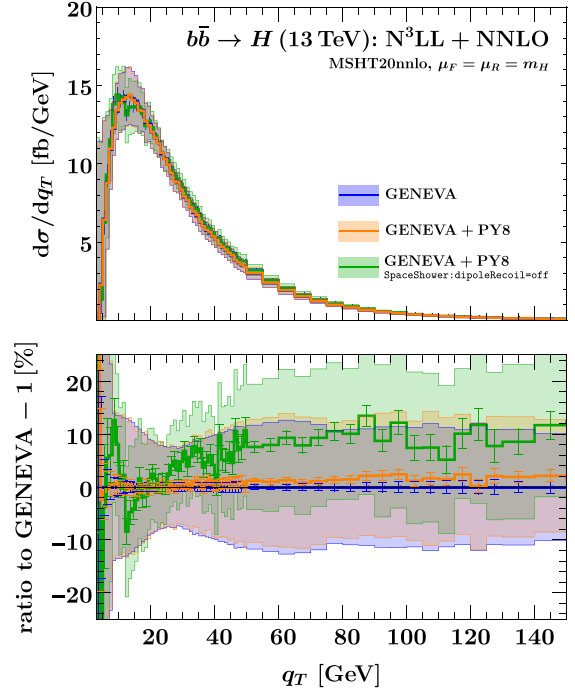
FIG. 6. Higgs boson q_T spectrum in b\bar{b} \rightarrow H . Results are shown at parton level and after showering.
