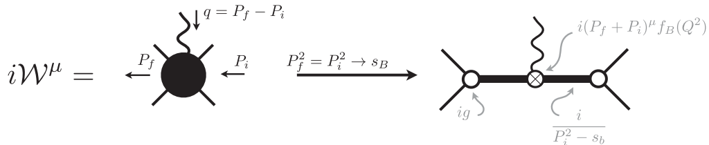
FIG. 1. Shown is a qualitative depiction of the 2 + \mathcal{J}^\mu \rightarrow 2 amplitude \mathcal{W}^\mu and its relation to the bound-state form factor f_B . Note Q^2 = -(P_f - P_i)^2 .
