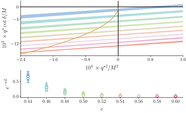
FIG. 4. Top: the resulting parametrized q^* \cot \delta / M ( q^* refers to CM relative momentum) for the different values of the coupling c considered in Fig. 2 as a function of the CM compared to the bound-state condition, as given in Eq. (9). Bottom: the expected finite-volume corrections on the matrix elements as a function of the coupling of the theory.
