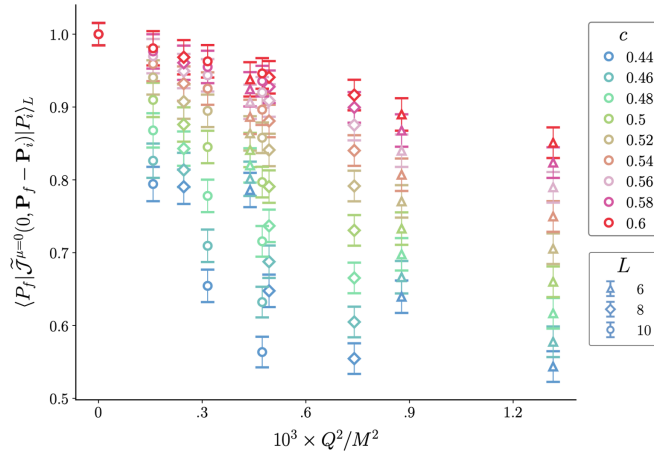
FIG. 6. Shown are the finite-volume matrix elements, obtained using the construction in Sec. III A, for the transition from the ground state to moving frames mediated by the temporal electromagnetic current, interacting with only one of the particles, as a function of Q^2 . The matrix elements are calculated for the finite-volume spectrum across various values of the coupling and lattice sizes.
