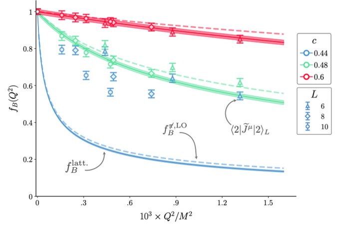
FIG. 10. Shown is the final result for the bound-state elastic form factor using Eq. (1) and the parametrized form of \mathcal{A}^0 in Eq. (55) for three couplings compared to the LO perturbative result from Eq. (61) and to the finite-volume matrix elements defined in Sec. III A.
