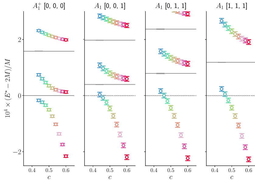
FIG. 2. Shown is the finite-volume spectra for the A_1^{(+)} cubic irreps for a range of values of c and fixed values of L = 10 and M = 50 . The errors are introduced as discussed in the main body of text. The solid lines show the noninteracting spectrum, and the dashed line shows the two-particle threshold.
