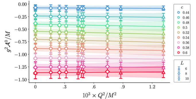
FIG. 7. We present the results for the dimensionless quantity g^2 \mathcal{A}^0/M , where g^2 is the residue of the bound state and \mathcal{A}^0 is obtained using Eq. (14). For each value of c , we fit the discrete points using the parametrization given in Eq. (55).
