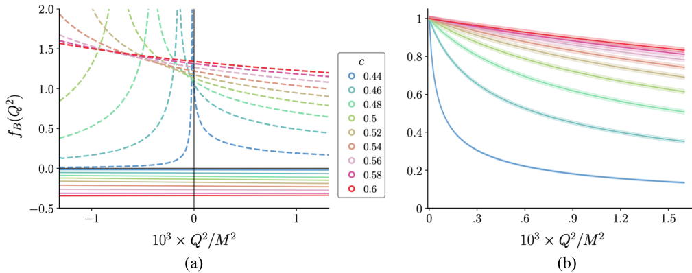
FIG. 8. Shown is the final result for the bound-state ground-state elastic form factor using Eq. (1) and the parametrized form of \mathcal{A}^0 in Eq. (55) for a range of couplings from deep- to shallow-bound states. In (a), we show the decomposition of factors contributing to the bound-state form factor, where the solid lines are the \mathcal{A}^0 contributions [Eq. (56)] and the dashed lines are the contributions from the scalar and vector triangle functions [Eq. (57)] for a range of couplings. In (b), we show the resulting form factor with propagated errors.
