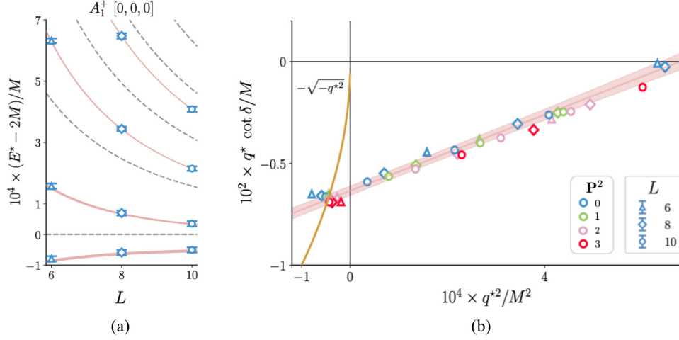
FIG. 3. Shown is the procedure for constraining the scattering amplitude from the finite-volume spectrum using the Lüscher quantization condition in Eq. (27) for c = 0.5 . Using the finite-volume energy levels in Fig. 2, the ERE parametrization in Eq. (8) is numerically constrained. In (a), we show the result of inverting this procedure, allowing us to predict the finite-volume spectrum as a function of the lattice size in any frame, where we present the case of the rest frame. The red line is the predicted energy levels with error, while the points are the obtained finite-volume spectrum, and the dashed gray lines are the noninteracting energy levels. In (b), we show the resulting 1\sigma band for q^* \cot \delta / M alongside the finite-volume spectrum and the bound-state condition, -\sqrt{-q^{*2}} .
