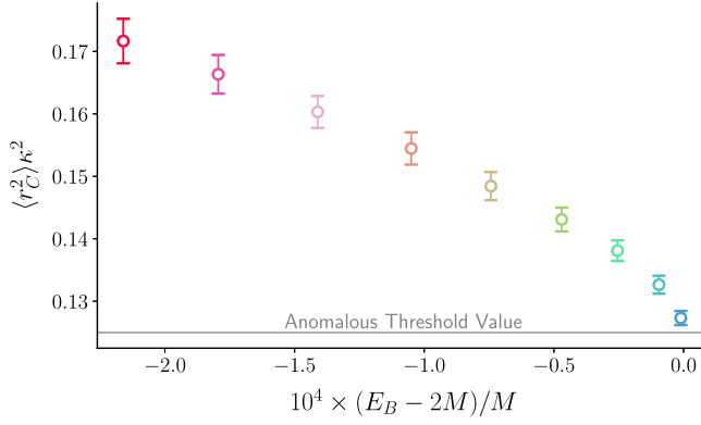
FIG. 9. The extracted charged radius of the bound states as a function of the extracted bound-state energy compared to the predicted value of the anomalous threshold.
