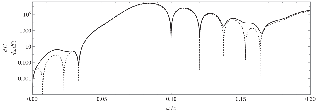
FIG. 4. The energy spectrum for nonlinear Compton scattering \frac{dE}{d\omega d\Omega} as a function of \omega/\varepsilon , the photon angles are \theta_{pk,x} = \theta_{pk,y} = 0 . The details of numerical computation are discussed in the text. The black line corresponds to the exact result, the dashed line corresponds to the soft photon approximation result.
