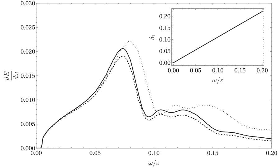
FIG. 5. The energy spectrum for nonlinear Compton scattering \frac{dE}{d\omega} as a function of \omega/\varepsilon . The details of numerical computation are discussed in the text. The black line corresponds to the exact result, the dashed line corresponds to the soft photon approximation result, and the dotted line corresponds to the classical result. Inset: the relative difference \delta_1 between the exact and the soft photon energy spectra as a function of \omega/\varepsilon .
