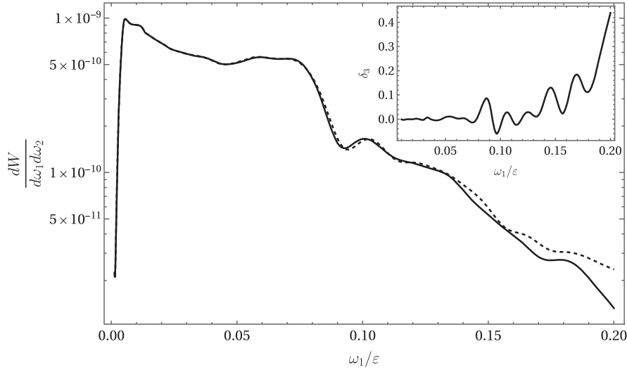
FIG. 11. The probability of double nonlinear Compton scattering integrated over the photon angles as a function of \omega_1/\varepsilon , \omega_2 = \varepsilon/25 . The details of numerical computation are discussed in the text. The black line corresponds to dW (soft photon result) and the dashed line corresponds to dW_c (the cascade contribution (31) in the soft-photon approximation). Inset: the relative difference \delta_3 between dW and dW_c as a function of \omega_1/\varepsilon .
