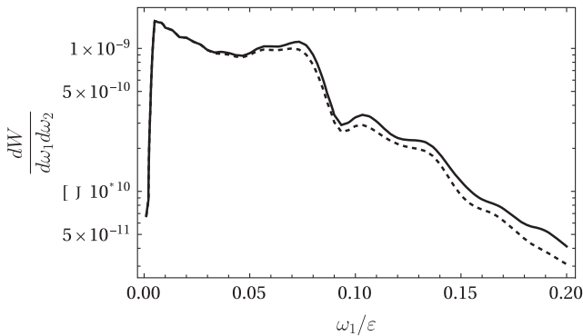
FIG. 9. The probability of double nonlinear Compton scattering integrated over the photon angles as a function of \omega_1/\varepsilon , \omega_2 = \varepsilon/100 . The details of numerical computation are discussed in the text. The black line corresponds to dW^{(1)} (exact in \omega_1 , soft photon approximation in \omega_2 ) and the dashed line corresponds to dW (soft photon approximation for both photons).
