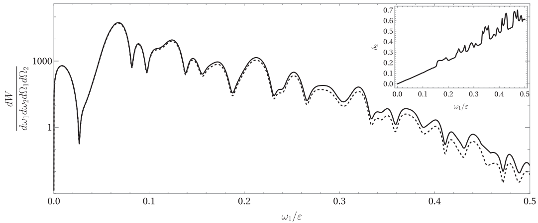
FIG. 7. The probability of double nonlinear Compton scattering \frac{dW}{d\omega_1 d\omega_2 d\Omega_1 d\Omega_2} as a function of \omega_1/\varepsilon , the photon angles are \theta_{pk_1x} = \frac{m}{4\varepsilon} , \theta_{pk_1y} = \frac{m}{2\varepsilon} , \theta_{pk_2x} = \frac{m}{3\varepsilon} , \theta_{pk_2y} = \frac{m}{\pi\varepsilon} , and \omega_2 = \varepsilon/100 . The details of numerical computation are discussed in the text. The black line corresponds to dW^{(1)} and the dashed line corresponds to dW . Inset: the relative difference \delta_2 between dW^{(1)} and dW as a function of \omega_1/\varepsilon .
