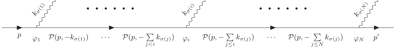
FIG. 12. The Feynman diagram for N -photon nonlinear Compton scattering which corresponds to the emission order k_{\sigma(1)}, k_{\sigma(2)}, \dots, k_{\sigma(N)} for permutation \sigma . Here, we also depict the phase of each interaction point and the momenta of the intermediate electron.
