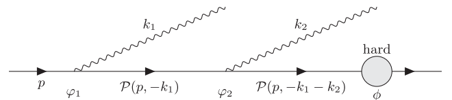
FIG. 1. Space-time picture of double soft photon emission from an initial electron line.
