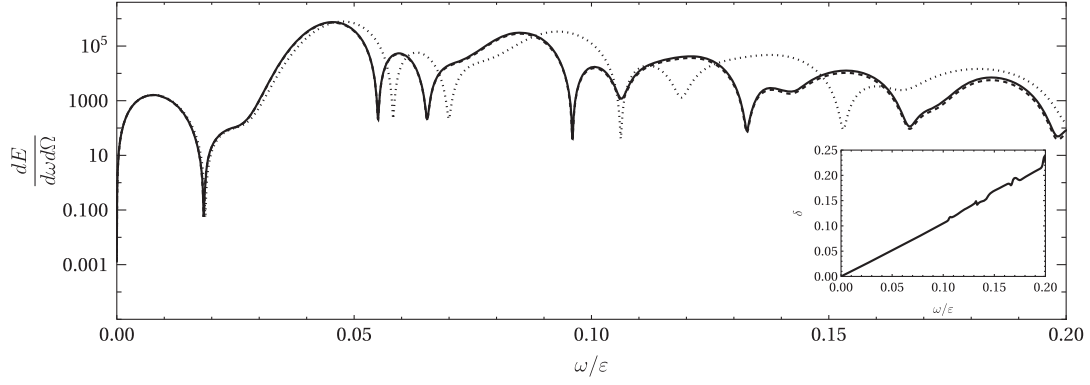
FIG. 3. The energy spectrum for nonlinear Compton scattering \frac{dE}{d\omega d\Omega} as a function of \omega/\varepsilon , the photon angles are \theta_{pk,x} = \frac{m}{2\varepsilon} , \theta_{pk,y} = \frac{m}{\varepsilon} . The details of numerical computation are discussed in the text. The black line corresponds to the exact result, the dashed line corresponds to the soft photon approximation result, and the dotted line corresponds to the classical result. Inset: the relative difference \delta between the exact and the soft photon energy spectra for nonlinear Compton scattering as a function of \omega/\varepsilon .
