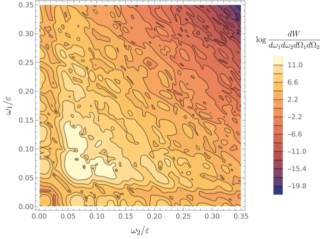
FIG. 8. The logarithm of the probability of double nonlinear Compton scattering \log \frac{dW}{d\omega_1 d\omega_2 d\Omega_1 d\Omega_2} as a function of \omega_1/\varepsilon and \omega_2/\varepsilon . The photon angles are \theta_{pk_1x} = \frac{m}{4e} , \theta_{pk_1y} = \frac{m}{2e} , \theta_{pk_2x} = \frac{m}{5e} , \theta_{pk_2y} = \frac{m}{\pi e} . The details of numerical computation are discussed in the text.
