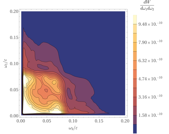
FIG. 10. The angle-integrated probability of double nonlinear Compton scattering \frac{dW}{d\omega_1 d\omega_2} as a function of \omega_1/\varepsilon and \omega_2/\varepsilon . The details of numerical computation are discussed in the text.
