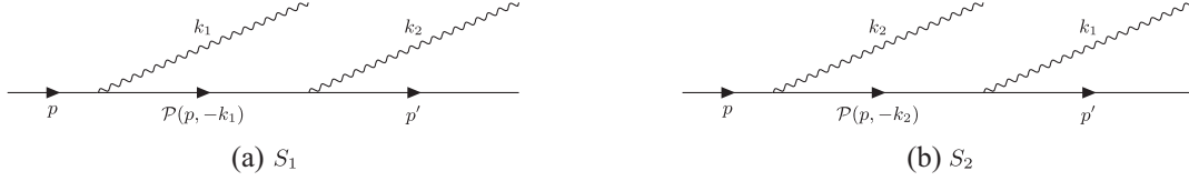
FIG. 6. Feynman diagrams for nonlinear double Compton scattering. (a) S_1 and (b) S_2 .
