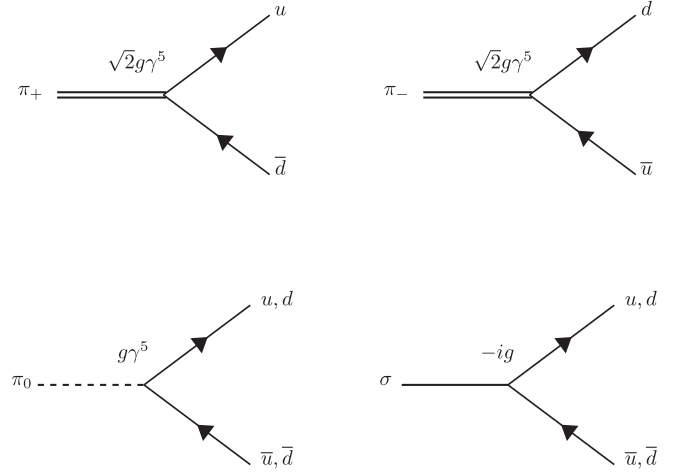
FIG. 2. Feynman diagrams corresponding to the four meson-quark interaction vertices in the LSMq. Solid, dashed, and double solid lines, and solid lines with arrows denote the sigma meson, the neutral pion, the charged pions, and the quarks, respectively.
