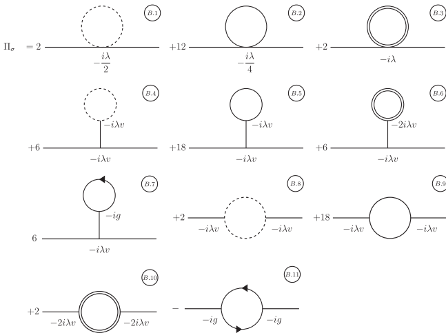
FIG. 4. One-loop self-energy diagrams for the sigma meson field. Solid lines represent the sigma meson, dashed lines correspond to neutral pions, double solid lines denote charged pions, and solid lines with arrows represent quark fields. Each vertex explicitly displays the corresponding coupling coefficient, and the factors multiplying each diagram account for the associated combinatorial factors.
