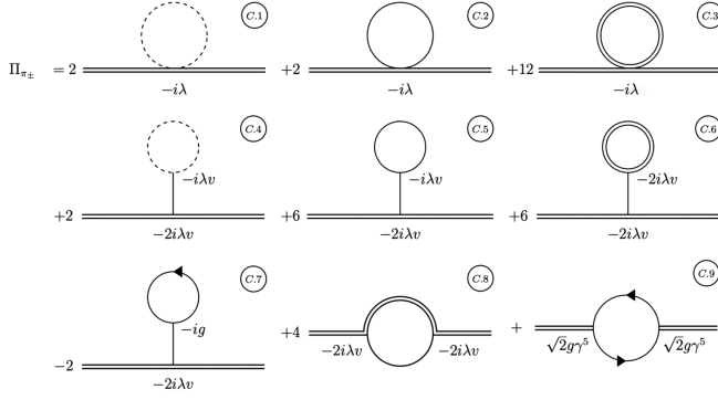
FIG. 5. One-loop self-energy diagrams for the charged pion fields. Solid lines represent the sigma meson, dashed lines correspond to neutral pions, double solid lines denote charged pions, and solid lines with arrows represent quark fields. Each vertex explicitly displays the corresponding coupling coefficient. The coefficients multiplying each diagram are the corresponding combinatorial factors.
