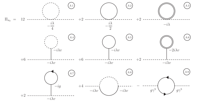
FIG. 3. One-loop self-energy diagrams for the neutral pion field. Solid lines represent the sigma meson, dashed lines correspond to neutral pions, double solid lines denote charged pions, and solid lines with arrows represent quark fields. Each vertex includes the corresponding coupling coefficient, and the factors multiplying the diagrams account for the associated combinatorial factors.
