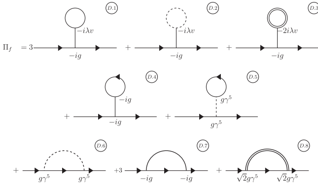
FIG. 6. One-loop self-energy diagrams for the quark fields (up and down). Solid lines represent the sigma meson, dashed lines correspond to neutral pions, double solid lines denote charged pions, and solid lines with arrows represent quark fields. Each vertex explicitly displays the corresponding coupling coefficient. The coefficients multiplying each diagram are the corresponding combinatorial factors.
