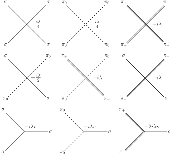
FIG. 1. Feynman diagrams corresponding to the nine interaction vertices among the mesonic fields in the LSMq. Solid, dashed, and double solid lines denote the sigma meson, the neutral pion, and the charged pions, respectively.
