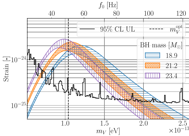
FIG. 4. Upper limit estimates at a 95% confidence level (black curve) as a function of frequency (top axis) and the corresponding boson mass assuming the central values for the mass and age of Cygnus X-1 (bottom axis). The hashed regions correspond to the predicted strain amplitude from a VBC around Cygnus X-1, assuming the central value (orange, circles), fifth percentile (blue, horizontal lines), and 95th percentile (purple, vertical lines) of the BH mass posterior distribution from [90]. We assume the BH initial spin to be \chi_i = 0.95 and the hashed regions account for uncertainties in the BH age and distance.
