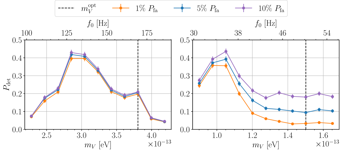
FIG. 3. The detection probability P_{\text{det}} as a function of m_V (bottom axis) and the corresponding GW frequency f_0 in the detector frame (top axis) with a 1% (orange), 5% (blue), and 10% (purple) false alarm probability for the remnant BHs from the GW230814 (left) and GW231123 (right) mergers. A redshift correction has been applied to obtain f_0 in the detector frame using the median D_L value for each remnant (as reported in Table I). The vertical dashed lines mark the optimal boson masses m_V^{\text{opt}} for the remnants with median parameters also shown in Table I. The error bars represent the 1\sigma beta-binomial uncertainty in P_{\text{det}} [156].
