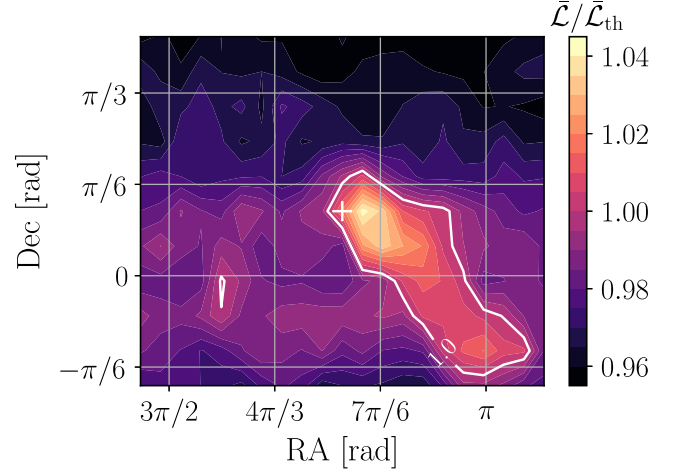
FIG. 2. Colored contour of \tilde{\mathcal{L}}/\tilde{\mathcal{L}}_{\text{th}} as a function of RA and Dec for a synthetic signal injected at [3.854, 0.370] rad, shown with a white cross marker. The signal was generated using the median BH remnant parameters from the GW230814 merger shown in Table I and using m_V = 2.283 \times 10^{-13} eV. The bright EPSF enclosed within the white contour signifies the region of the sky with \tilde{\mathcal{L}} > \tilde{\mathcal{L}}_{\text{th}} where the signal has been recovered.
