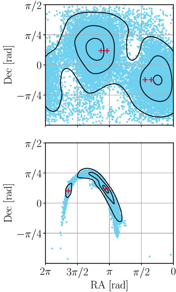
FIG. 1. Joint RA and Dec posterior distribution for the merger remnants from GW230814 (top) and GW231123 (bottom). The black contours show the 90%, 50%, and 10% confidence intervals. The red crosses indicate the sky positions targeted in the search for each remnant.
