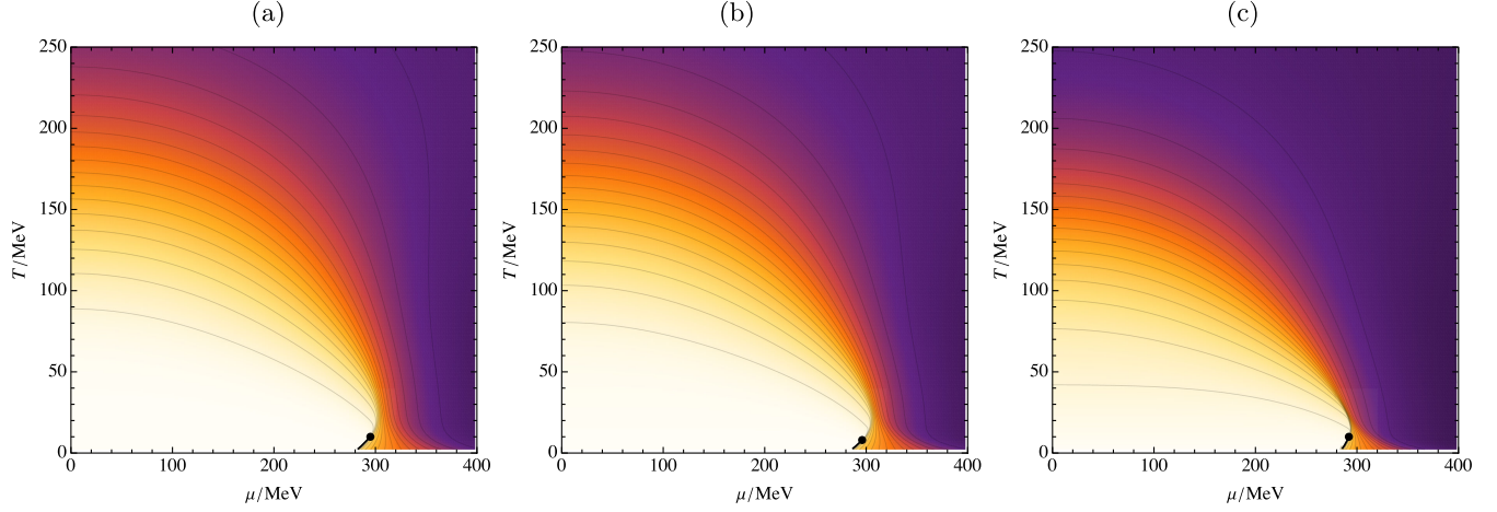
FIG. 6. Phase diagrams for (a) zero damping ( \gamma_\sigma = \gamma_\pi = 0 ), (b) infinite damping for the sigma, but zero damping for the pion ( \gamma_\sigma = \infty , \gamma_\pi = 0 ), and (c) infinite damping for both sigma and pions ( \gamma_\sigma = \gamma_\pi = \infty ). Here the UV cutoff is reduced to \Lambda = 647.3 MeV, which quantitatively changes also the zero-damping phase diagram in (a) compared to the one in Fig. 2(a) at high temperatures T \sim \Lambda/(2\pi) \sim 103 MeV.
