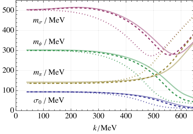
FIG. 5. Flow of static observables in vacuum ( \mu = 0, T = 0 ) for \gamma_\sigma = \gamma_\pi = 0 (solid), \gamma_\sigma = \infty, \gamma_\pi = 0 (dashed), and \gamma_\sigma = \gamma_\pi = \infty (dotted). Here the UV cutoff is \Lambda = 647.3 MeV.
