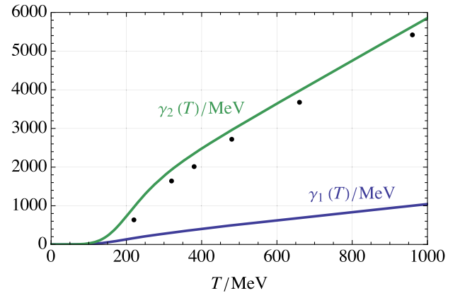
FIG. 8. The two models \gamma_1(T) (blue) and \gamma_2(T) (green) for the temperature dependence of the pion damping from Eqs. (92) and (93) plotted against the reconstructed damping-factor exponents of Ref. [65] (black).
