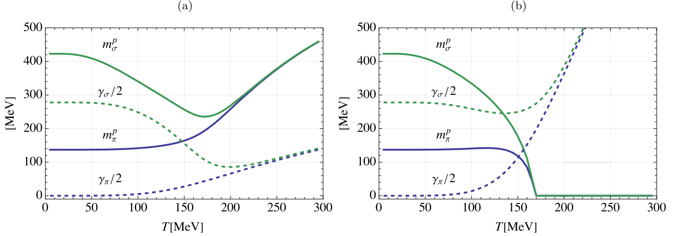
FIG. 4. Temperature dependence of real and imaginary parts of the sigma and pion poles at \mu = 0 , where (a) on the left and (b) on the right correspond to the two different models of pion damping \gamma = \gamma_1(T) and \gamma_2(T) as defined in Eqs. (92) and (93), respectively, and with constant Y adjusted so that the sigma pole mass m_\sigma^p reproduces that of the broad two-pion resonance in the vacuum at T = 0 in both cases.
