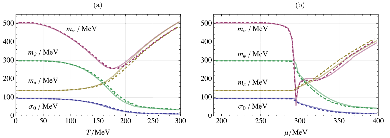
FIG. 3. Static IR observables that correspond to the three phase diagrams in Fig. 2, for zero damping (solid lines), for the first model \gamma = \gamma_1(T) defined in (92) (dotted), and for the second model \gamma = \gamma_2(T) defined in (93) (dashed). As discussed in the main text, in both cases with O(4) -symmetric damping \gamma \neq 0 we use the same constant Y in the sigma damping to reproduce the broad two-pion resonance pole in the vacuum. (a) \mu = 0 . (b) T = 10 MeV.
