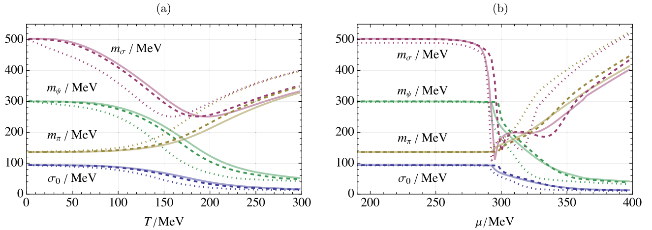
FIG. 7. Static IR observables for \gamma_\sigma = \gamma_\pi = 0 (solid), \gamma_\sigma = \infty , \gamma_\pi = 0 (dashed) and \gamma_\sigma = \gamma_\pi = \infty (dotted). Here the UV cutoff is \Lambda = 647.3 MeV. (a) \mu = 0 . (b) T = 10 MeV.
