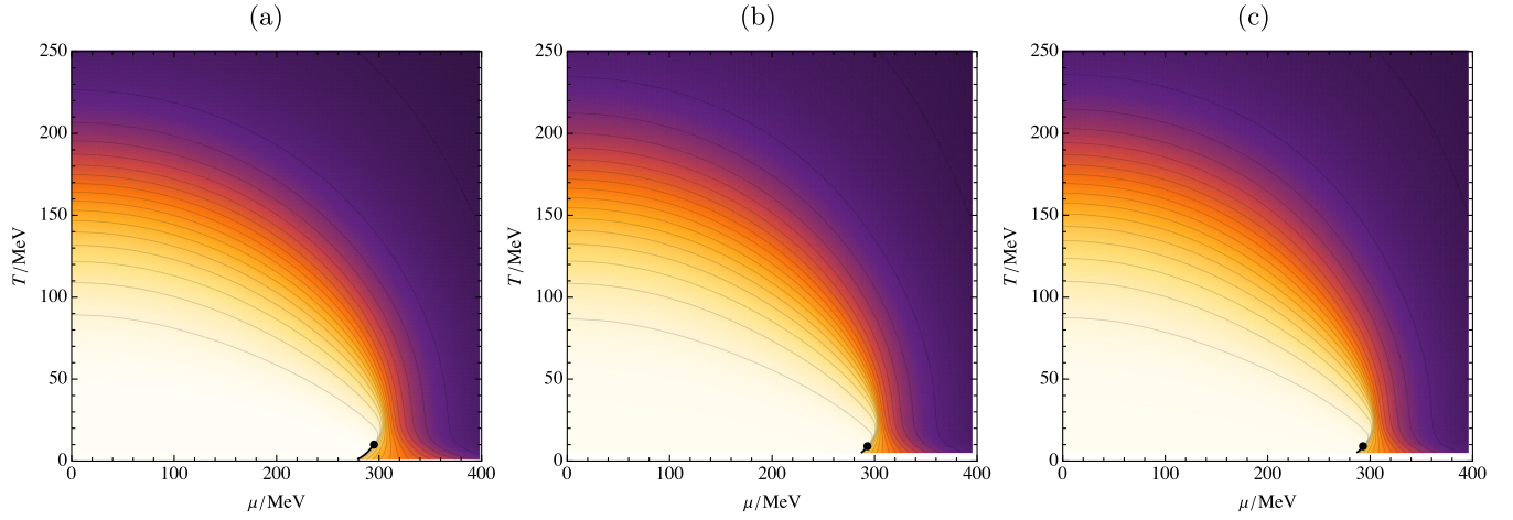
FIG. 2. Quark-meson model phase diagram (a) for zero damping ( Y = 0 , \gamma = 0 ), (b) for constant Y adjusted so that the sigma pole reproduces that of the broad two-pion resonance in the vacuum combined with the O(4) -symmetric damping \gamma = \gamma_1(T) from Eq. (92), and (c) for Y chosen as in (b) but with \gamma = \gamma_2(T) from Eq. (93).
