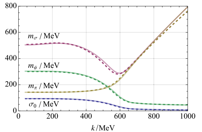
FIG. 1. FRG flow of static observables in vacuum ( \mu = 0 , T = 0 ) for zero damping (solid lines), and for \gamma = 0 , Y = 0.064 \text{ MeV}^{-1} (dashed lines).
