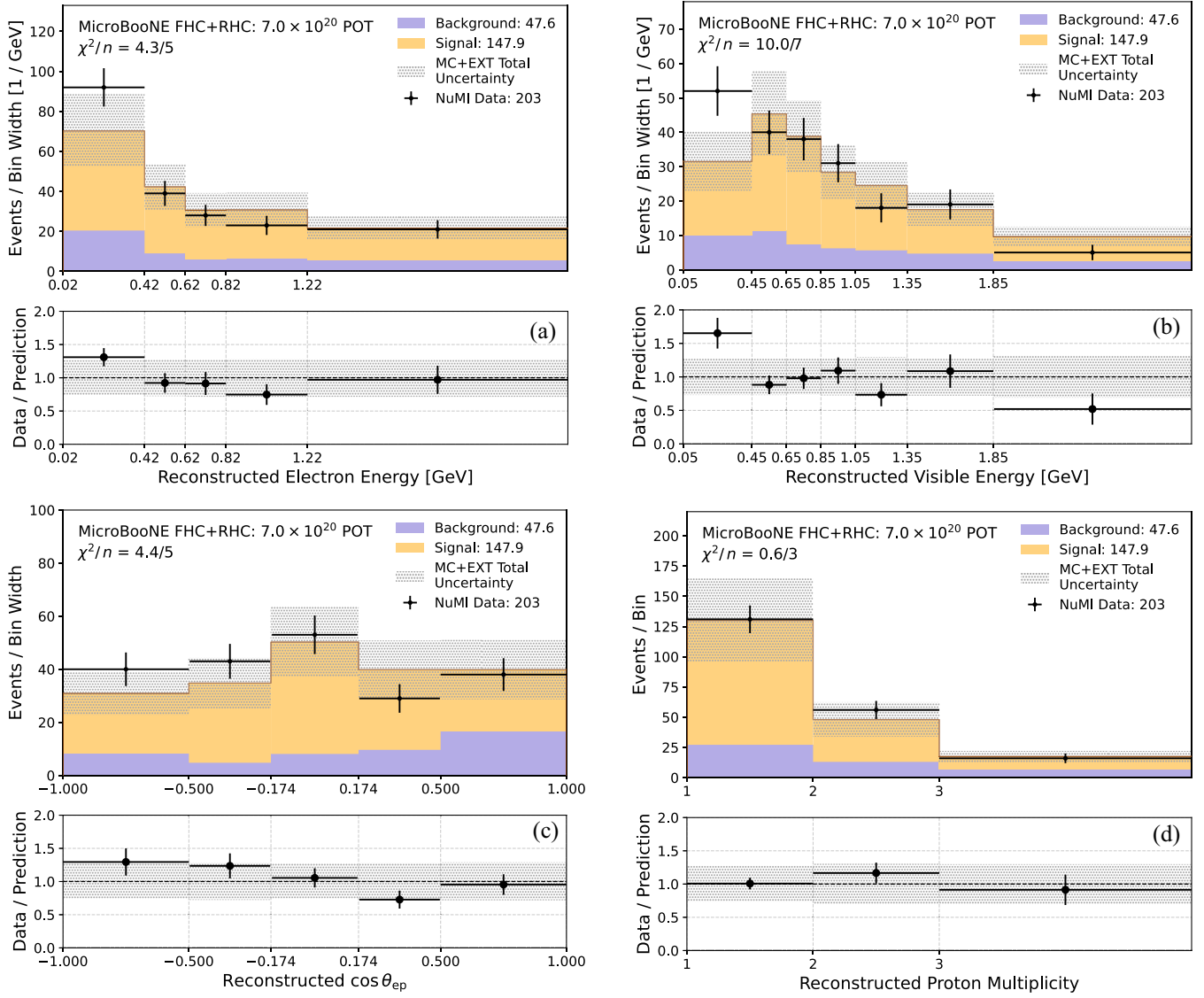
FIG. 5. Estimated signal (orange) and background (purple) predictions of the FHC + RHC selected events after the full selection (including the BDT threshold requirement) for reconstructed electron energy (a), visible energy (b), \cos \theta_{ep} (c), and proton multiplicity (d). The rightmost bin for the electron energy, visible energy, and proton multiplicity distributions is overflow. The gray band represents the total MC + EXT uncertainty, as described in Sec. IV. Data is overlaid for comparison, shown in black with associated statistical uncertainties. The data/MC ratios are also shown, where again the gray band represents the total MC + EXT uncertainty.
