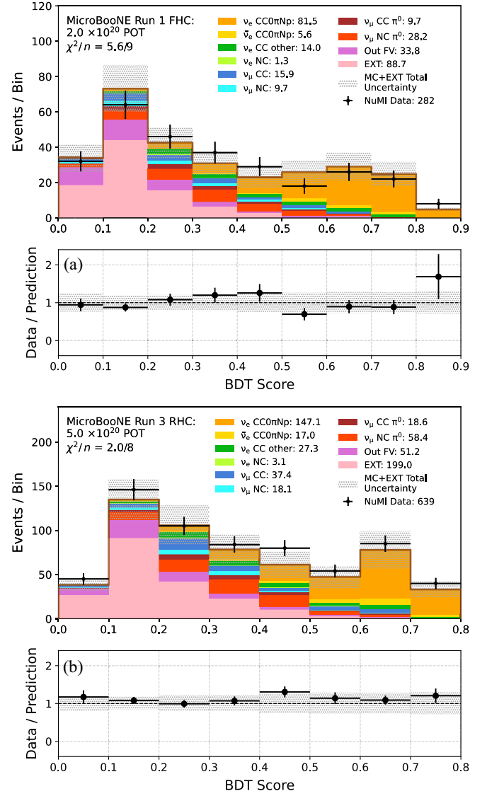
FIG. 4. Estimated event rates for Run 1 FHC (a) and Run 3 RHC (b) as a function of the output of the BDT trained to discriminate signal (orange) from various sources of background. The gray band represents the total MC + EXT uncertainty, as described in Sec. IV. Data is overlaid for comparison, shown in black with associated statistical uncertainties.
