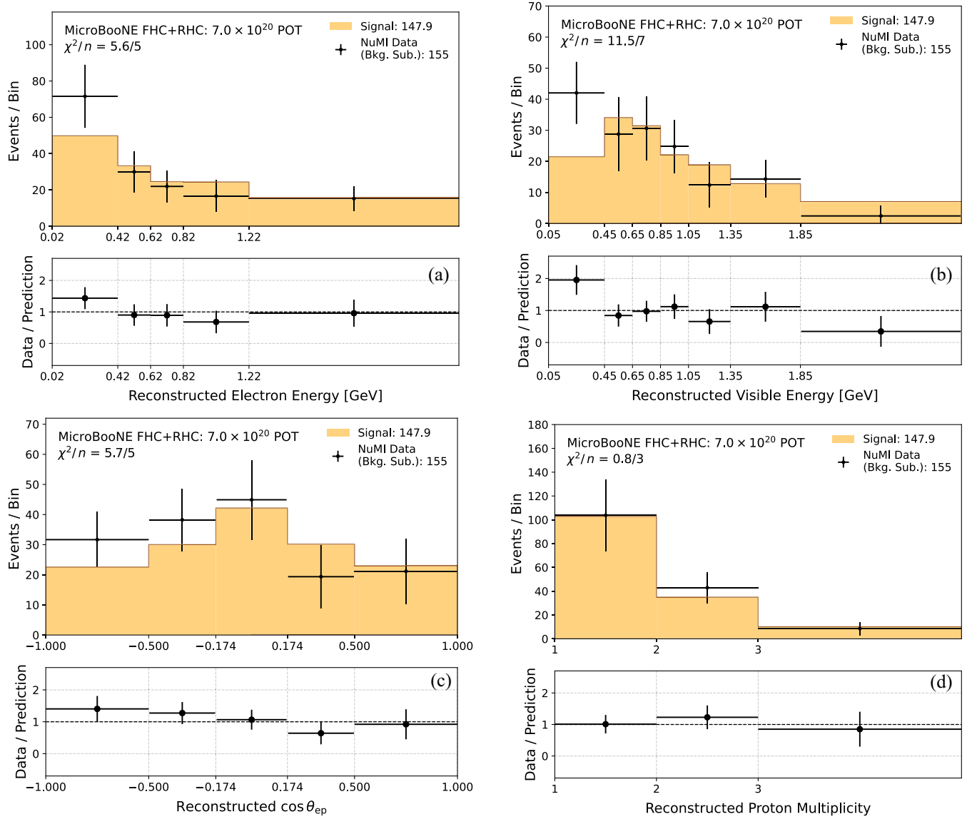
FIG. 6. Estimated signal (orange) predictions of the FHC + RHC selected events after background subtraction for reconstructed electron energy (a), visible energy (b), \cos \theta_{ep} (c), and proton multiplicity (d). The rightmost bin for the electron energy, visible energy, and proton multiplicity distributions is overflow. Background-subtracted NuMI data is overlaid for comparison, shown in black with associated statistical and systematic uncertainties. Included in these error bars are the systematic uncertainties on the signal prediction. The data/MC ratios are also shown.
