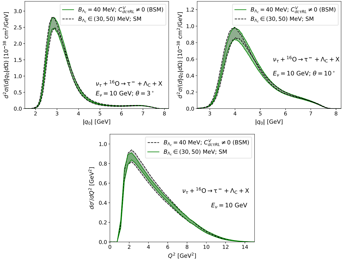
FIG. 5. Nuclear uncertainties versus sensitivity to BSM effects. Top left (right) panel: Double-differential cross section d^2\sigma/(d\Omega_\tau d|q_0|) for the QE reaction \nu_\tau + {}^{16}\text{O} \rightarrow \tau^- + \Lambda_c + X evaluated in {}^{16}\text{O} for E_\nu = 10 GeV and \theta_\tau = 3^\circ ( \theta_\tau = 10^\circ ). The green band stands for the variation induced in the distribution by the allowed values for the C^V_{dctRL} WC and fixing B_{\Lambda_c} = 40 MeV. The black dashed-lines show the uncertainty in the SM results when B_{\Lambda_c} varies in the 30–50 MeV range. Bottom panel: The d\sigma'/dQ^2 [ \sigma' = (8\pi M_n^2 \sigma)/(G_F |V_{cd}|)^2 ] cross section, per number of neutrons, for the same reaction.
