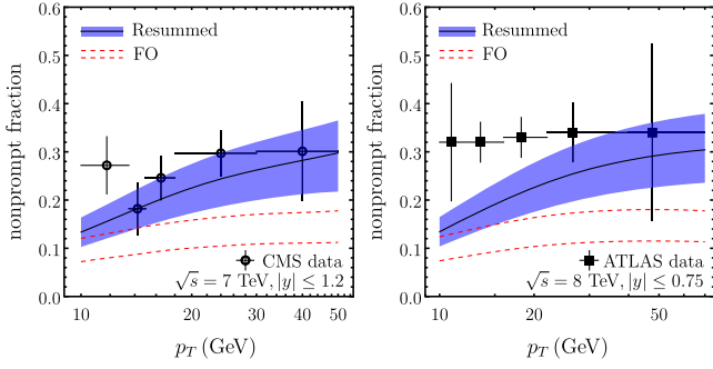
FIG. 1. Nonprompt fractions for \chi_{c1}(3872) production computed from Eq. (2) compared to CMS (left) and ATLAS (right) data.
